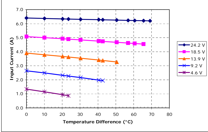
Unpotted VT-199-1.4-1.5 at a hot-side temperature of 30 °C
