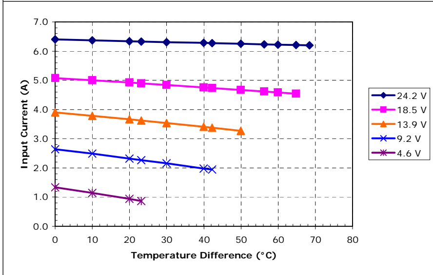
Potted VT-199-1.4-1.5 at a hot-side temperature of 30 °C
