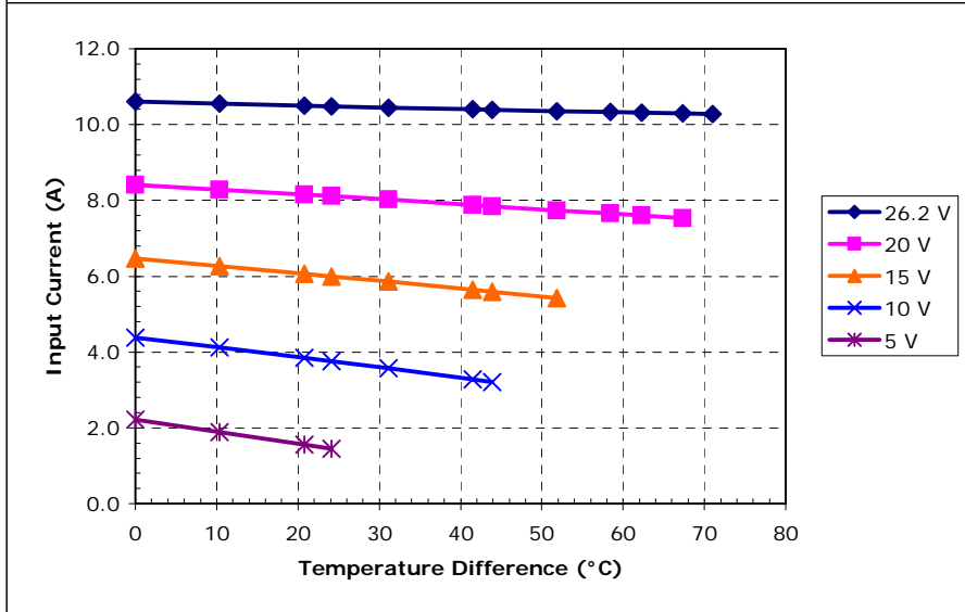
Potted VT-199-1.4-0.8 at a hot-side temperature of 50 °C
