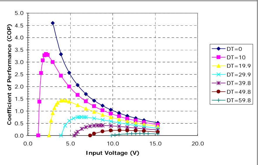
Unpotted VT-127-1.4-1.15-71 at a hot-side temperature of 30 °C
