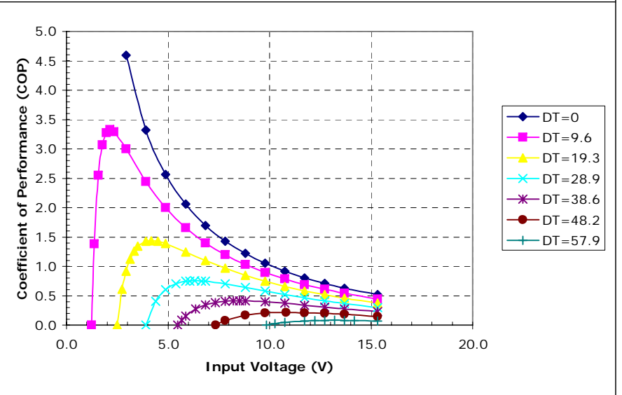
Potted VT-127-1.4-1.15-71 at a hot-side temperature of 30 °C
