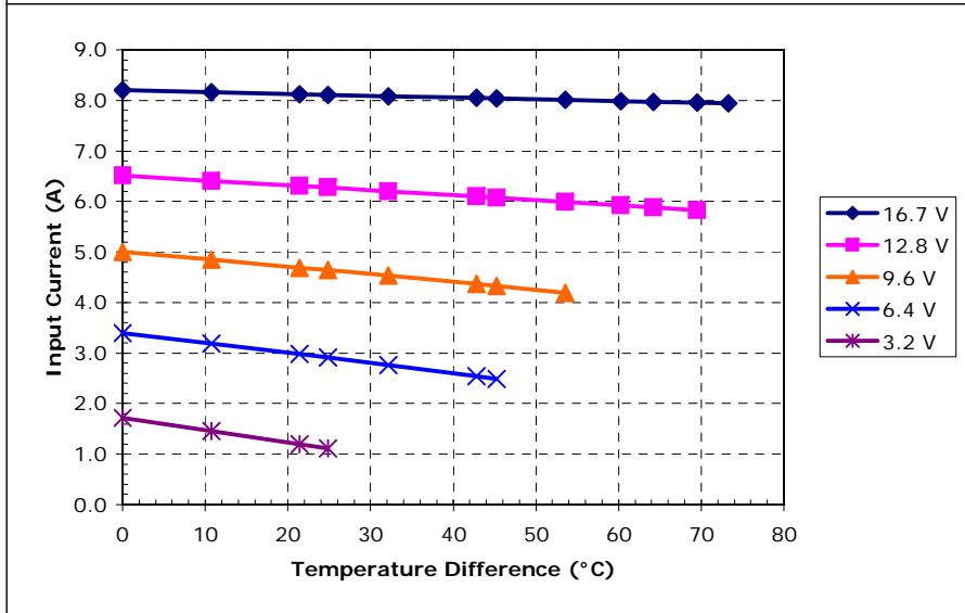
Potted VT-127-1.4-1.15-71 at a hot-side temperature of 50 °C
