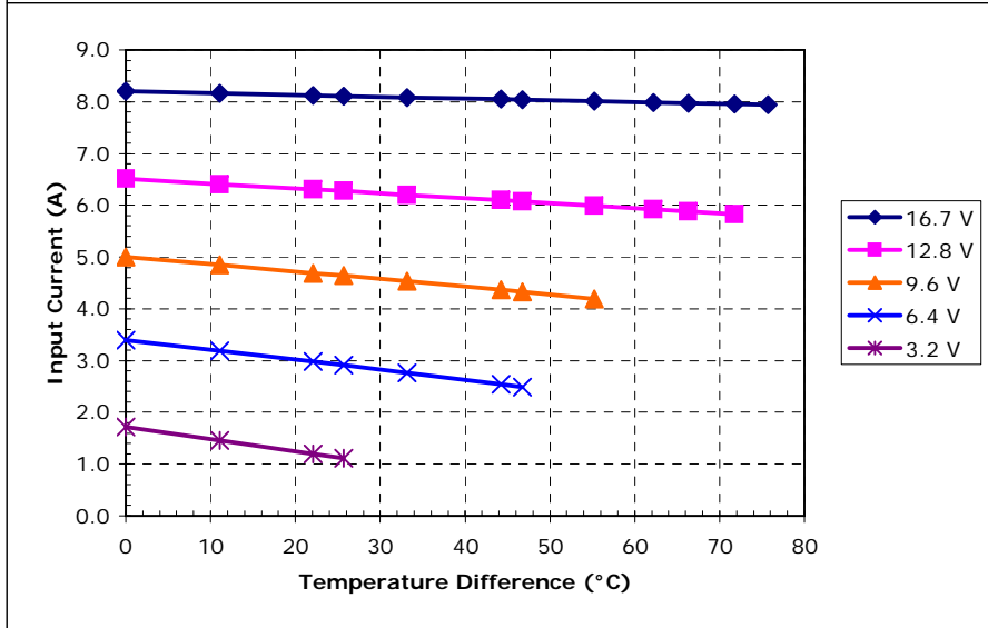
Unpotted VT-127-1.4-1.15-71 at a hot-side temperature of 50 °C
