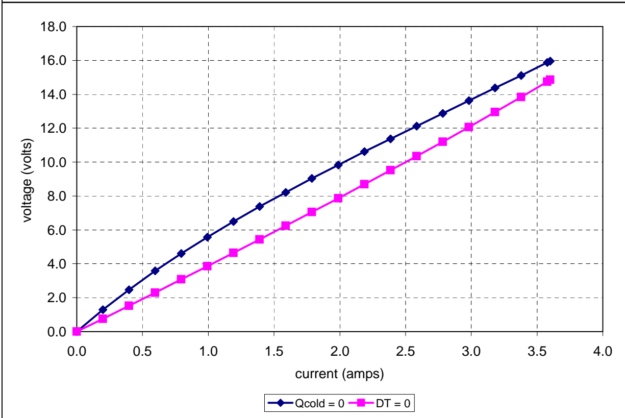
Potted VT-127-1.0-1.3-71 at a hot-side temperature of 25 °C
