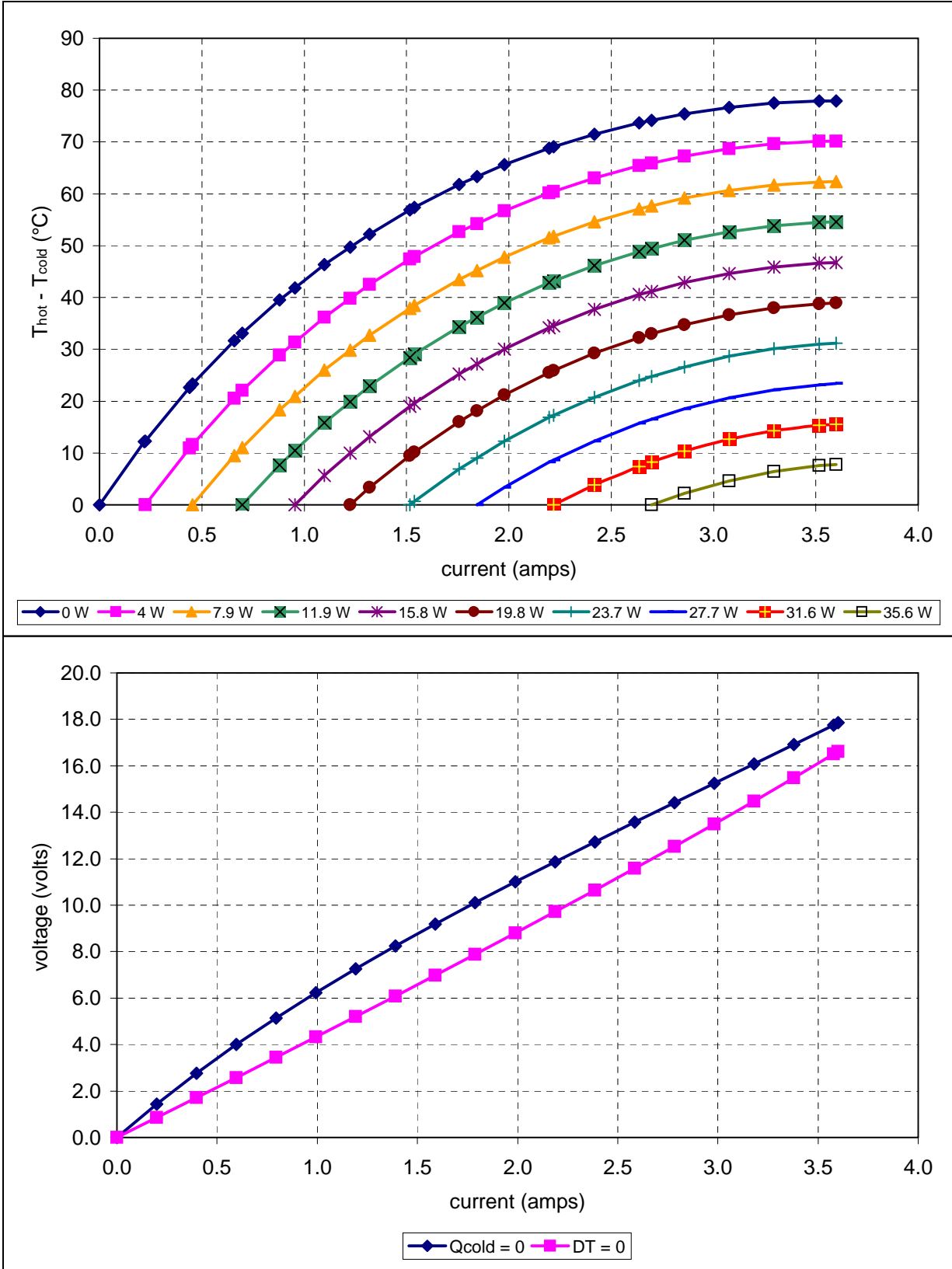
Potted VT-127-1.0-1.3-71 at a hot-side temperature of 50 °C
