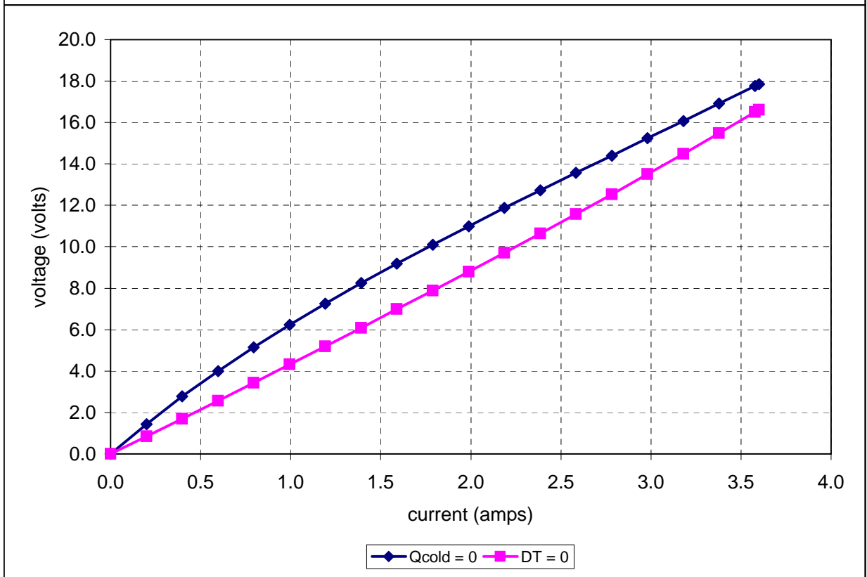
Unpotted VT-127-1.0-1.3-71 at a hot-side temperature of 50 °C
