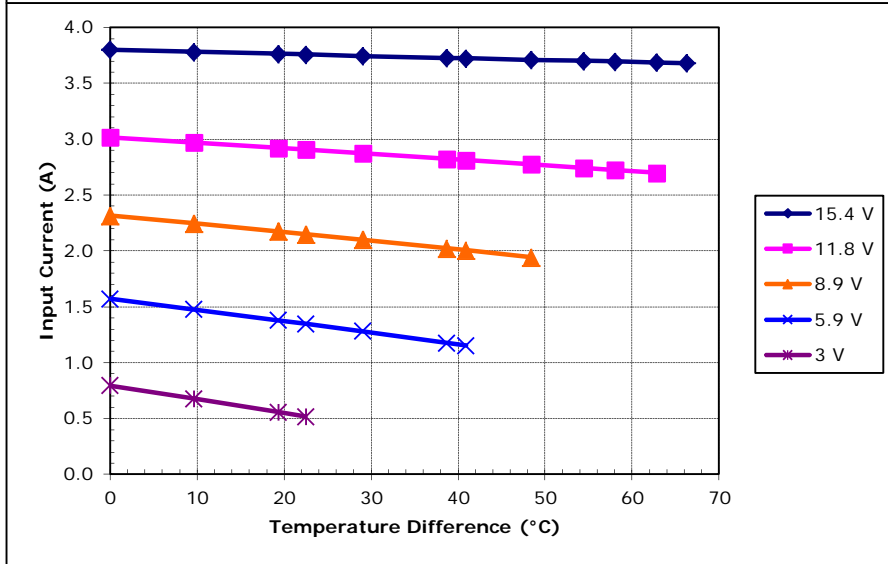
Potted VT-127-1.0-1.3-71 at a hot-side temperature of 30 °C
