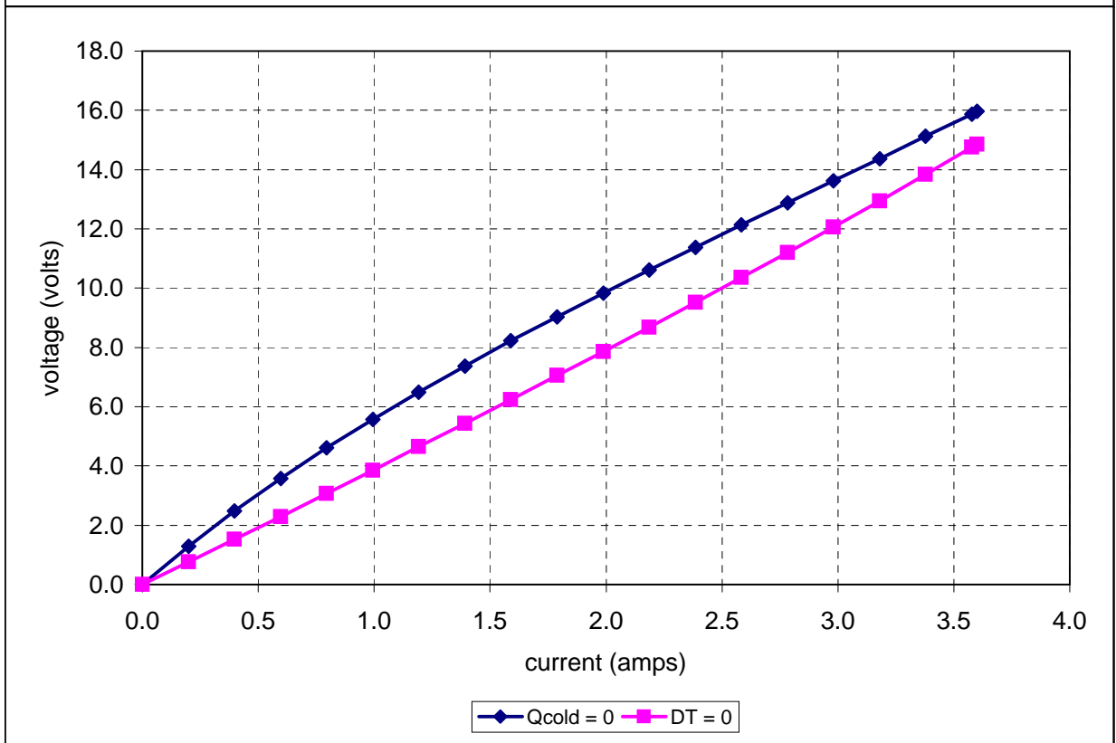
Unpotted VT-127-1.0-1.3-71 at a hot-side temperature of 25 °C
