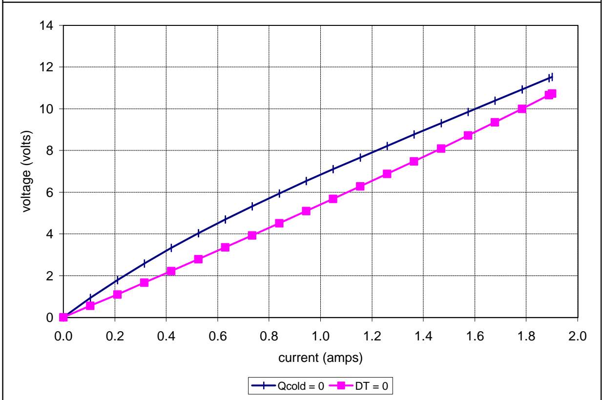
Potted TE-83-1.0-2.5 at a hot-side temperature of 50 °C
