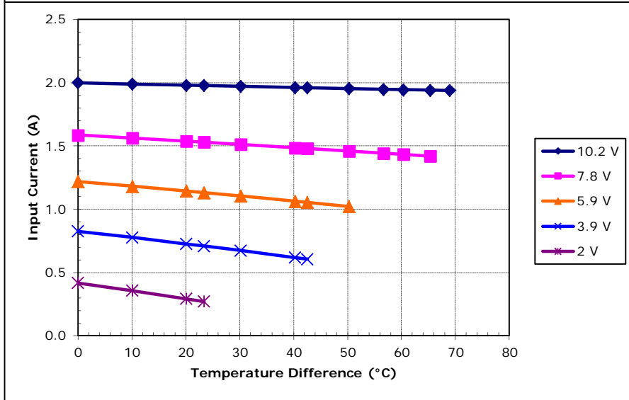
Potted TE-83-1.0-2.5 at a hot-side temperature of 30 °C
