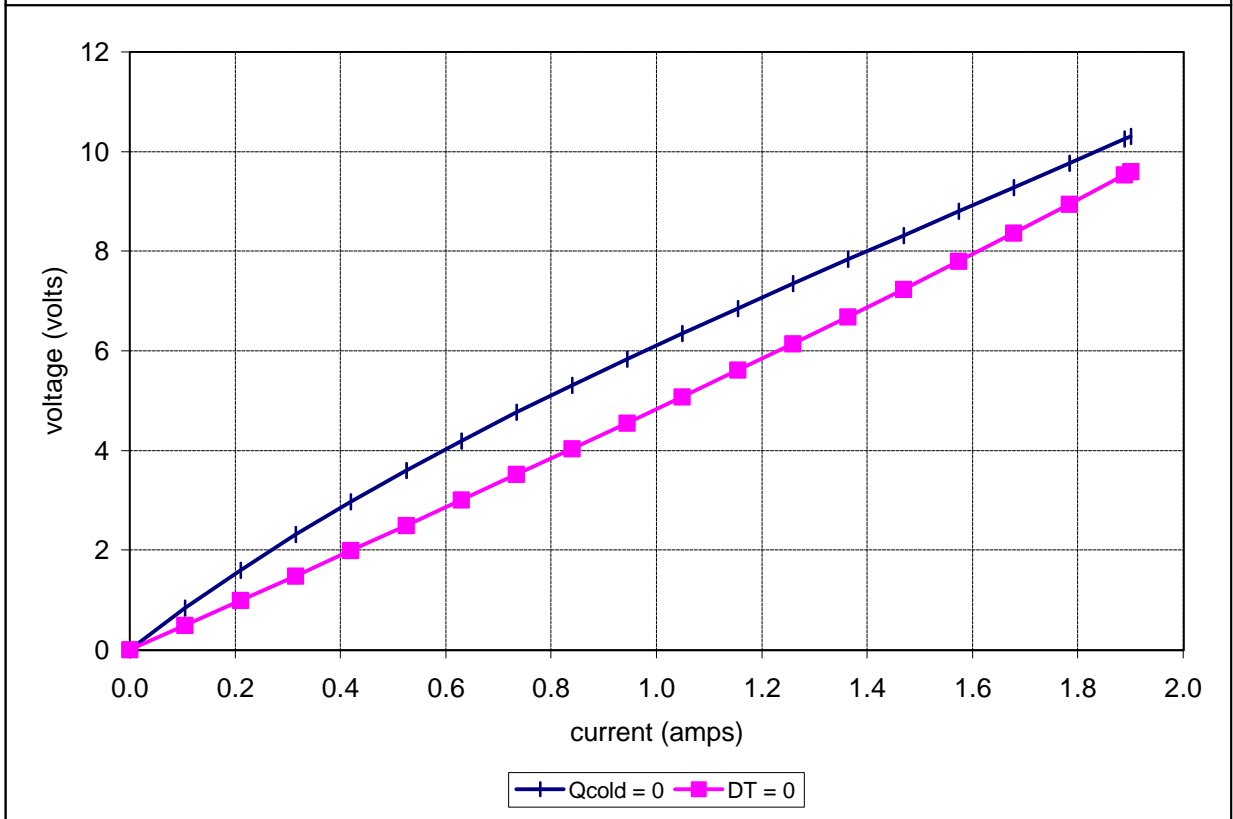
Potted TE-83-1.0-2.5 at a hot-side temperature of 25 °C
