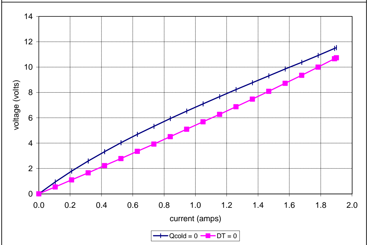
Unpotted TE-83-1.0-2.5 at a hot-side temperature of 50 °C
