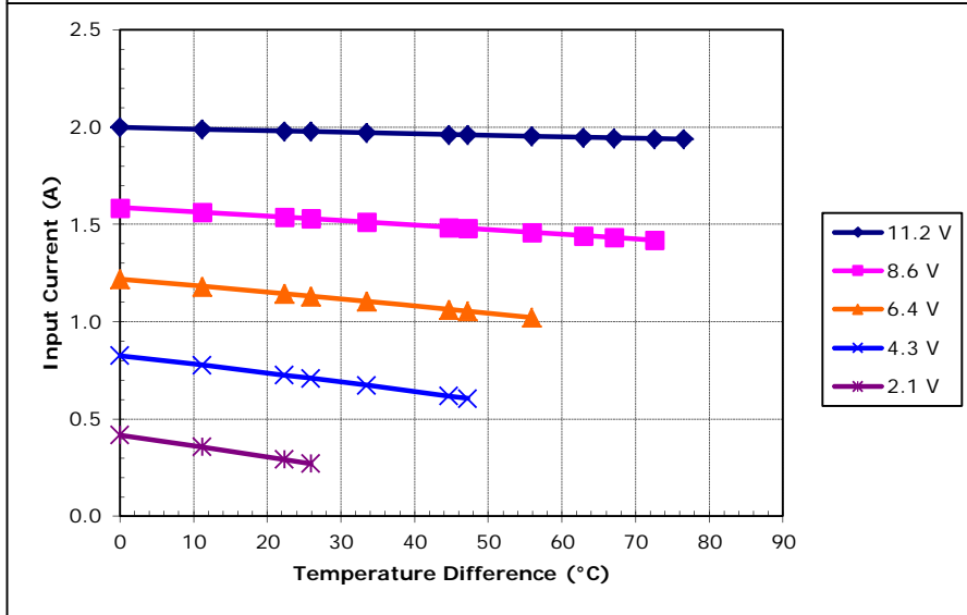
Potted TE-83-1.0-2.5 at a hot-side temperature of 50 °C
