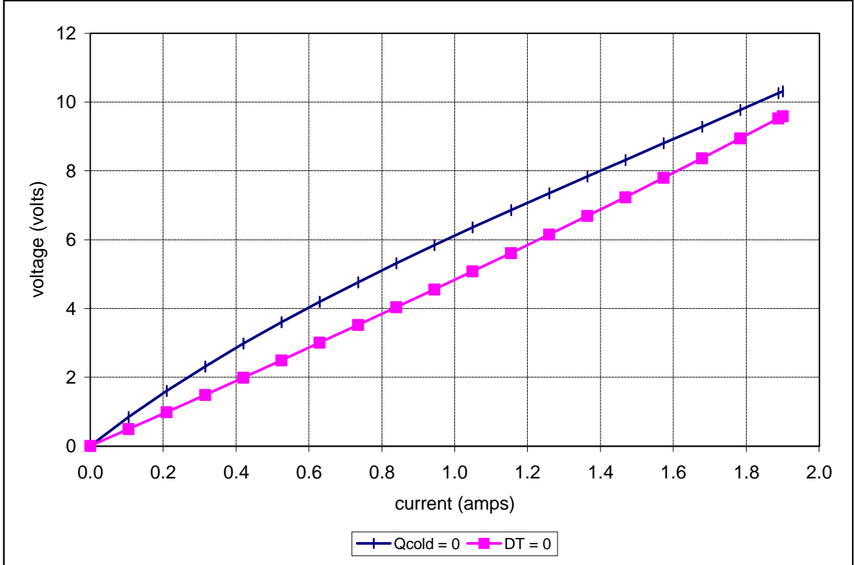
Unpotted TE-83-1.0-2.5 at a hot-side temperature of 25 °C
