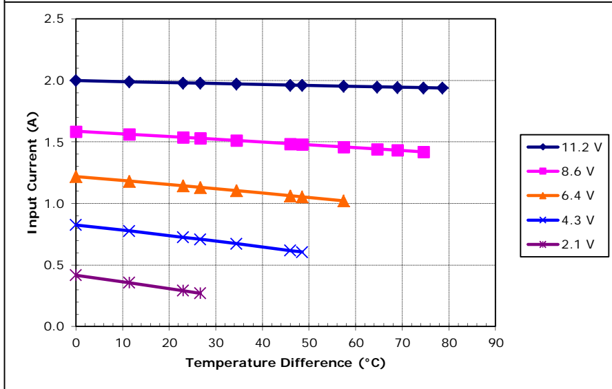
Unpotted TE-83-1.0-2.5 at a hot-side temperature of 50 °C
