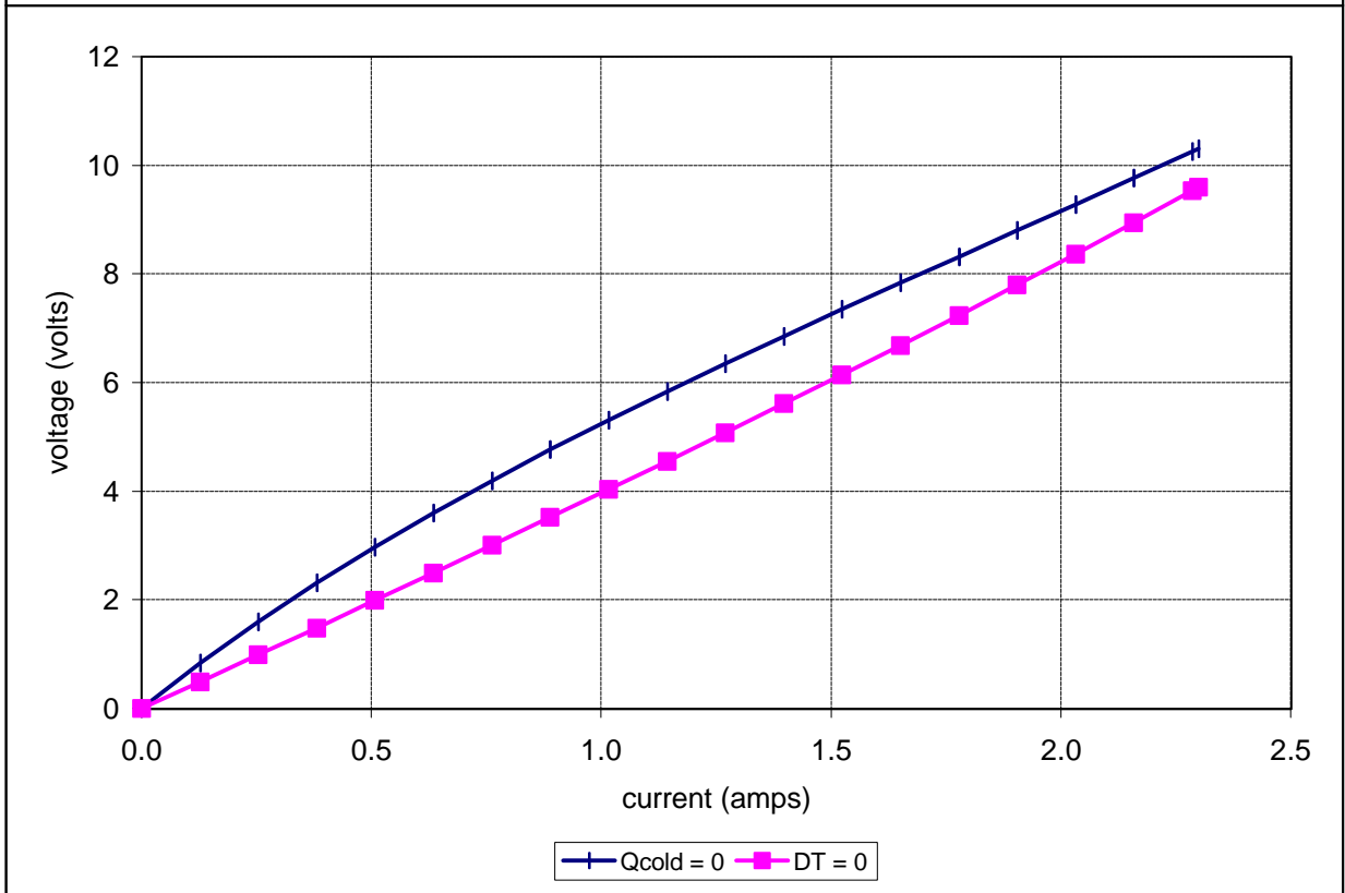
Potted TE-83-1.0-2.0 at a hot-side temperature of 25 °C
