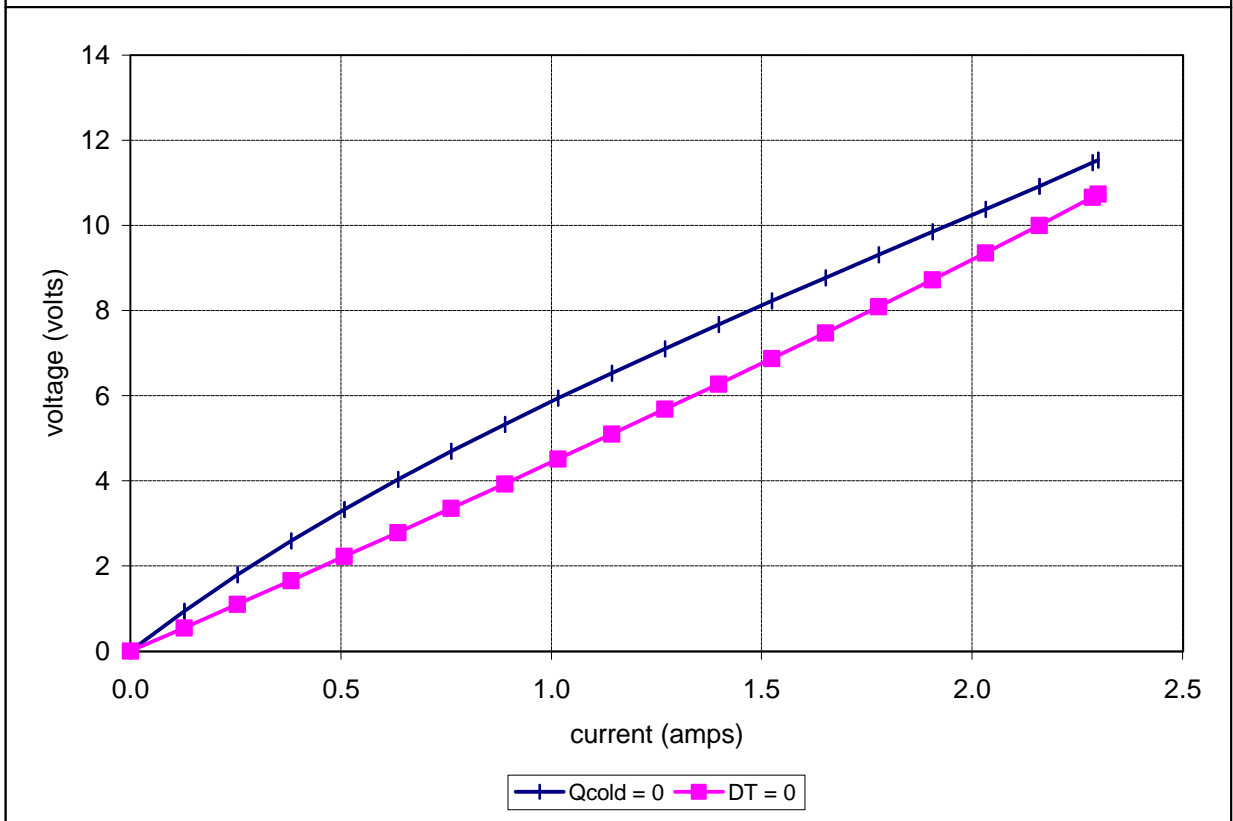
Unpotted TE-83-1.0-2.0 at a hot-side temperature of 50 °C
