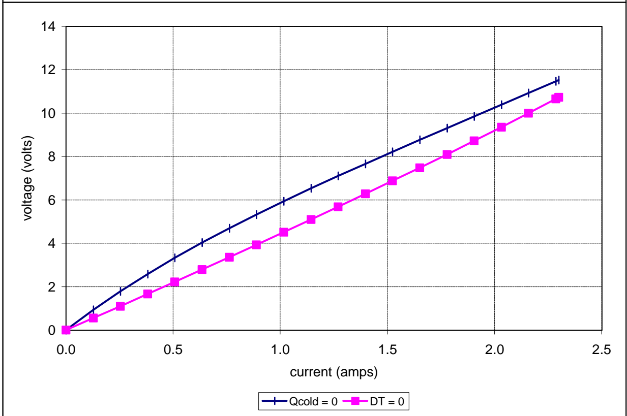
Potted TE-83-1.0-2.0 at a hot-side temperature of 50 °C
