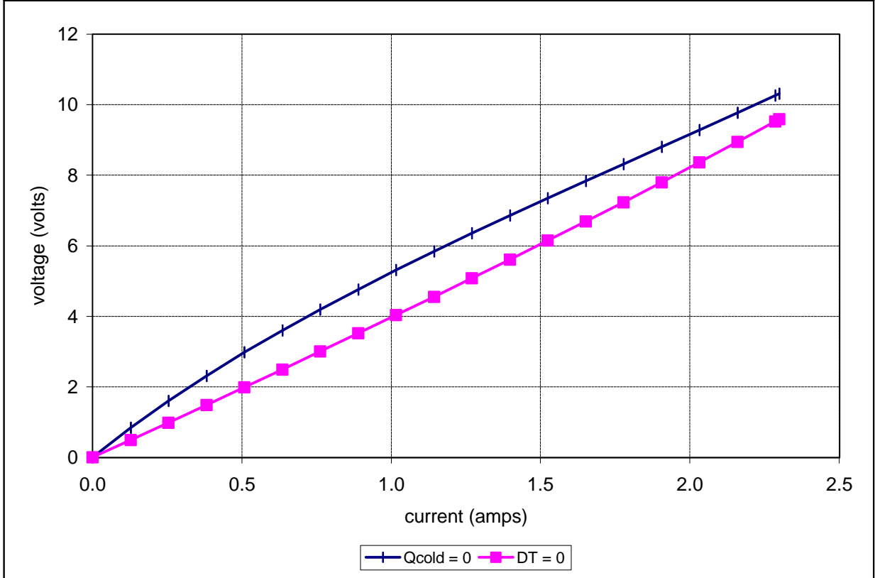
Unpotted TE-83-1.0-2.0 at a hot-side temperature of 25 °C
