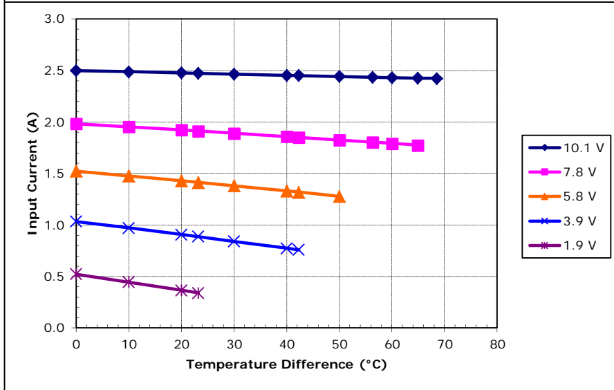
Potted TE-83-1.0-2.0 at a hot-side temperature of 30 °C
