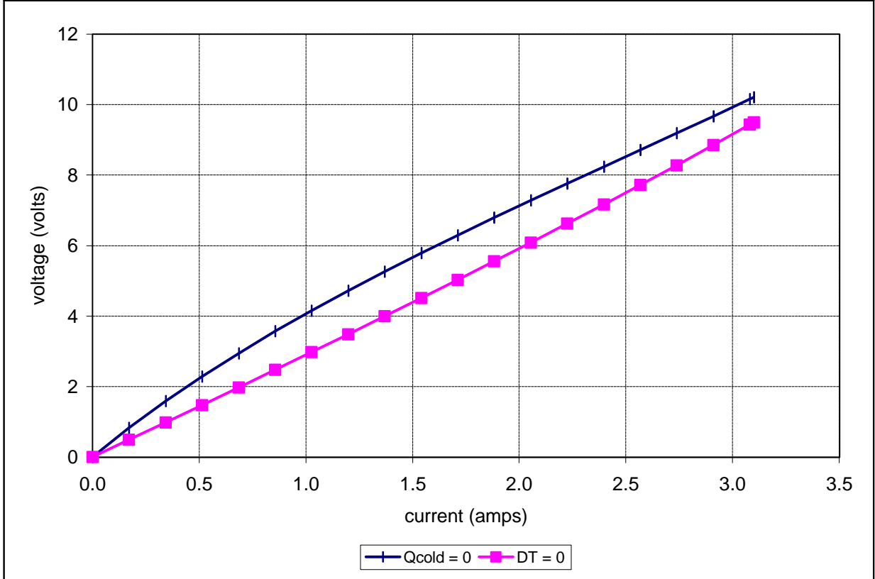
Unpotted TE-83-1.0-1.5 at a hot-side temperature of 25 °C
