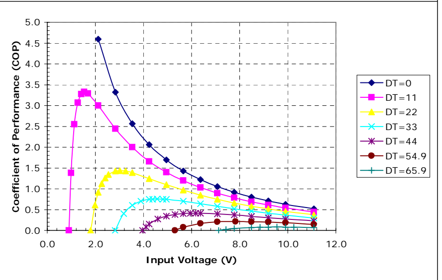
Potted TE-83-1.0-1.5 at a hot-side temperature of 50 °C
