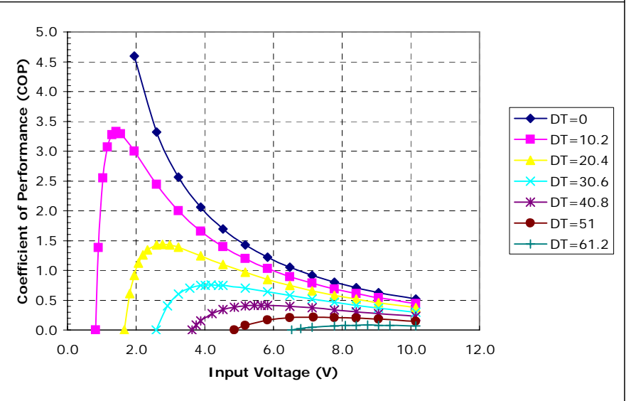
Unpotted TE-83-1.0-1.5 at a hot-side temperature of 30 °C
