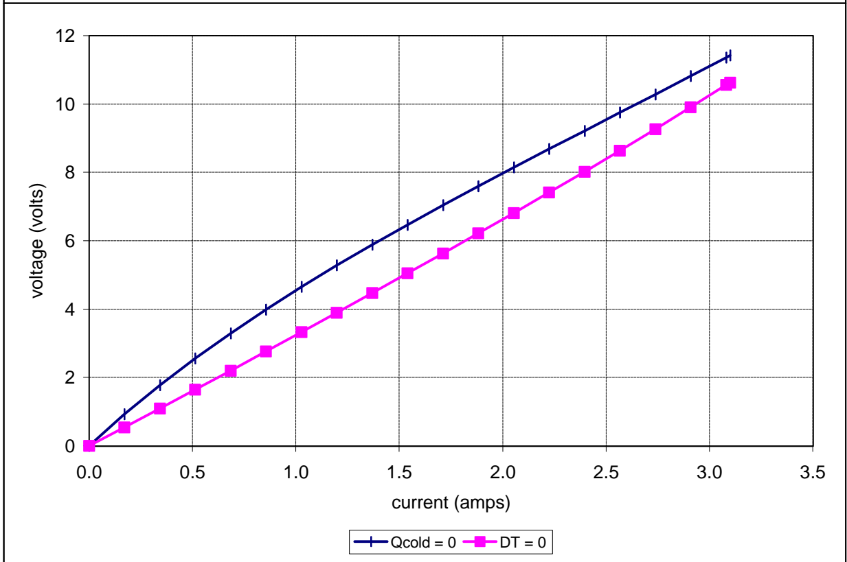
Potted TE-83-1.0-1.5 at a hot-side temperature of 50 °C
