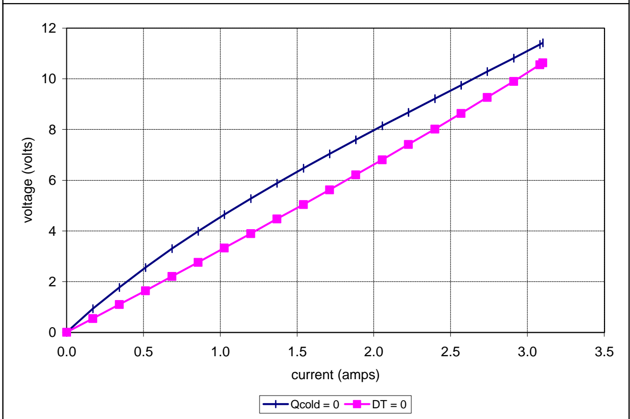
Unpotted TE-83-1.0-1.5 at a hot-side temperature of 50 °C
