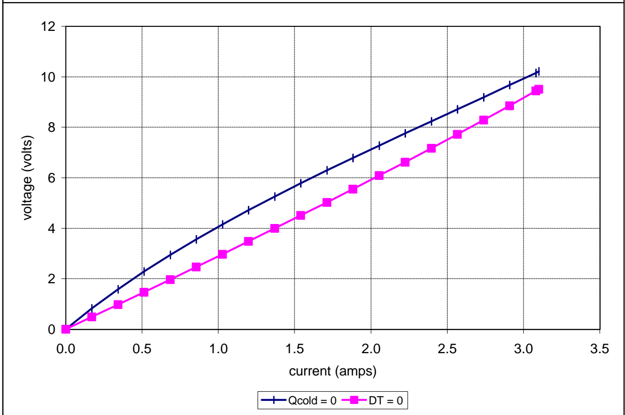
Potted TE-83-1.0-1.5 at a hot-side temperature of 25 °C
