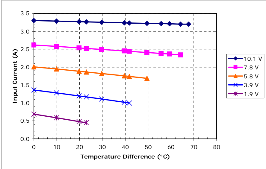
Potted TE-83-1.0-1.5 at a hot-side temperature of 30 °C
