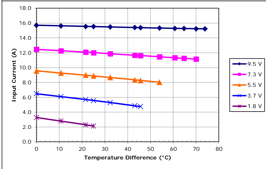
Unpotted TE-71-2.0-1.15 at a hot-side temperature of 50 °C
