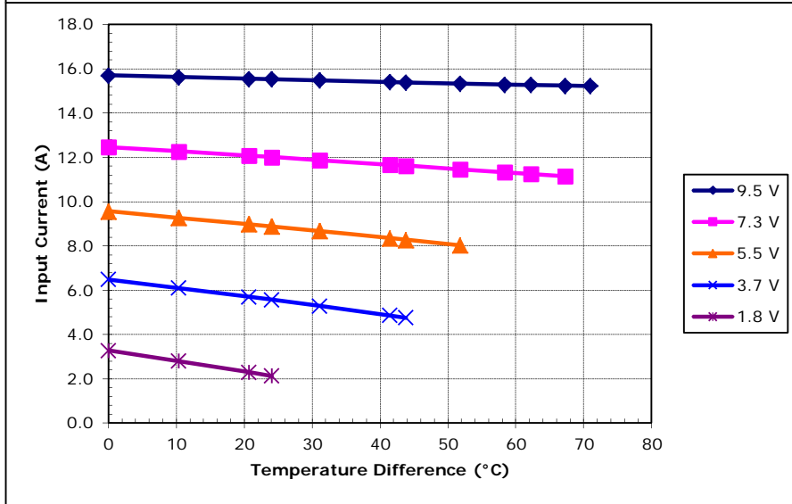
Potted TE-71-2.0-1.15 at a hot-side temperature of 50 °C
