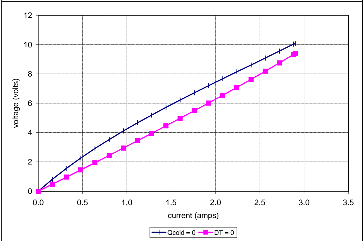
Potted TE-71-1.4-3.175 at a hot-side temperature of 50 °C
