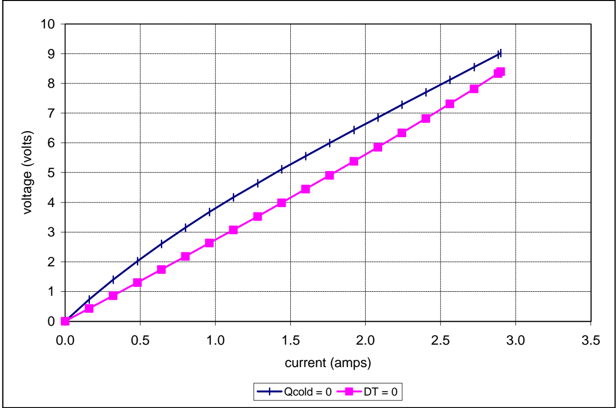
Unpotted TE-71-1.4-3.175 at a hot-side temperature of 25 °C
