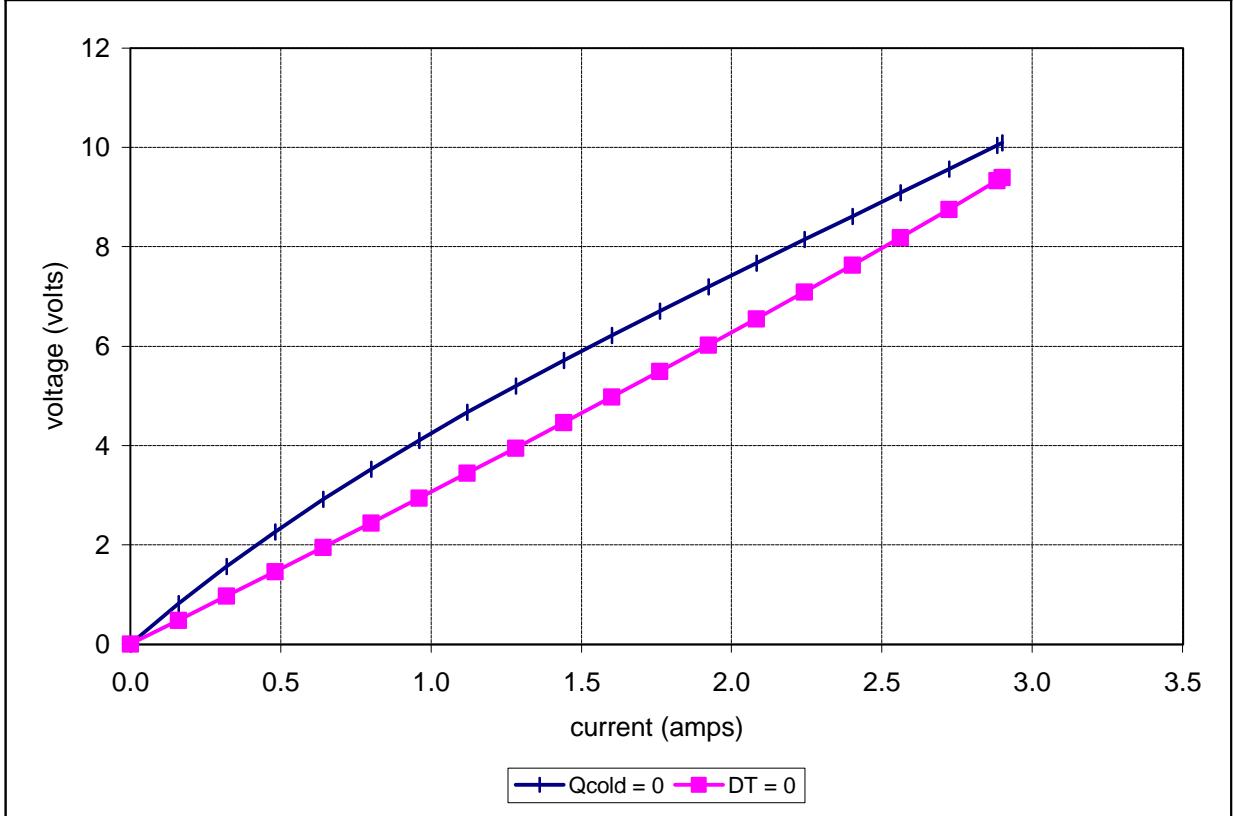
Unpotted TE-71-1.4-3.175 at a hot-side temperature of 50 °C
