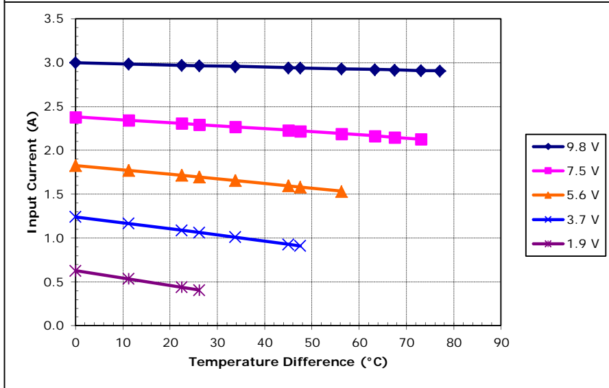
Unpotted TE-71-1.4-3.175 at a hot-side temperature of 50 °C
