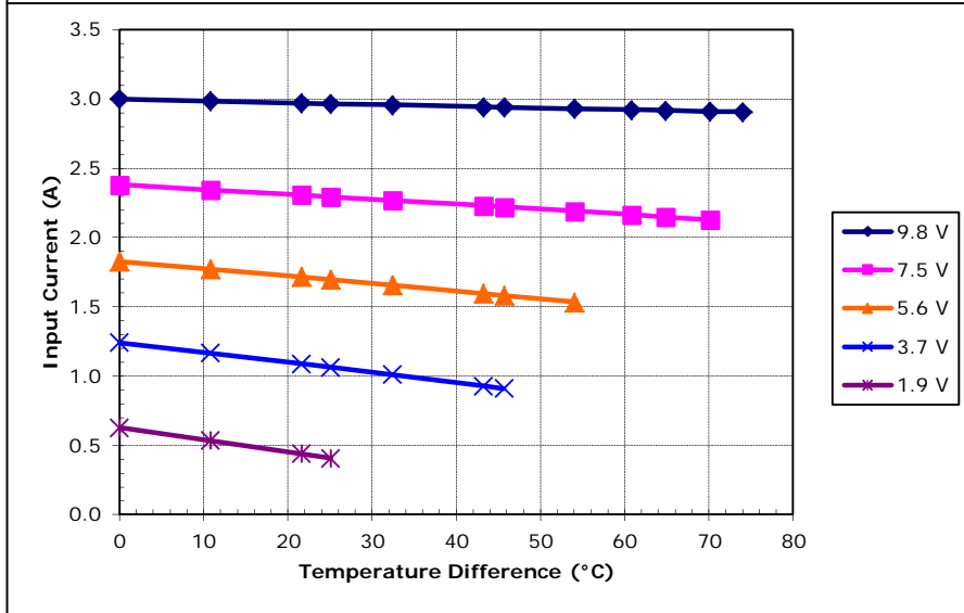
Potted TE-71-1.4-3.175 at a hot-side temperature of 50 °C
