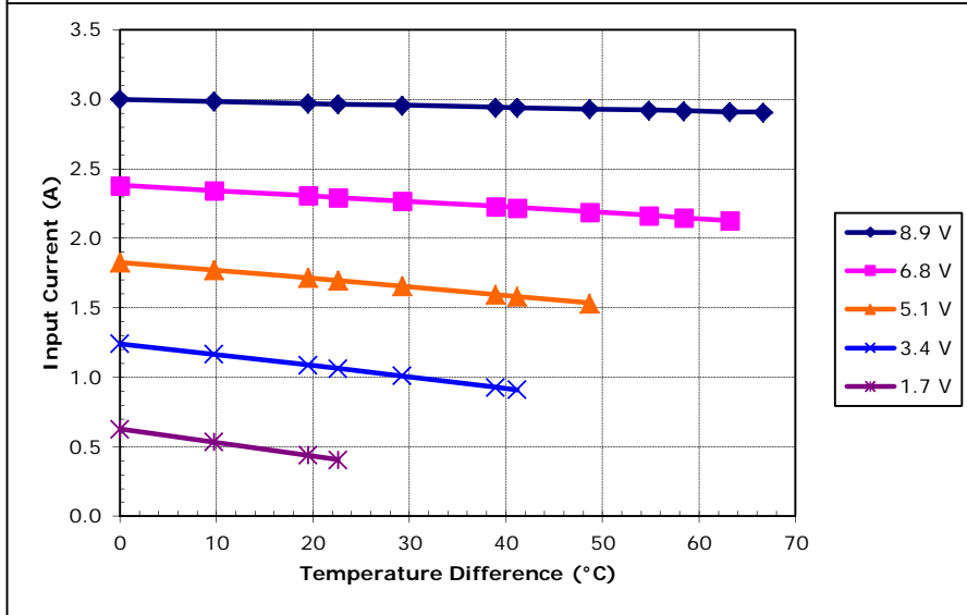
Potted TE-71-1.4-3.175 at a hot-side temperature of 30 °C
