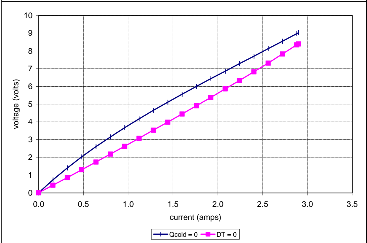
Potted TE-71-1.4-3.175 at a hot-side temperature of 25 °C
