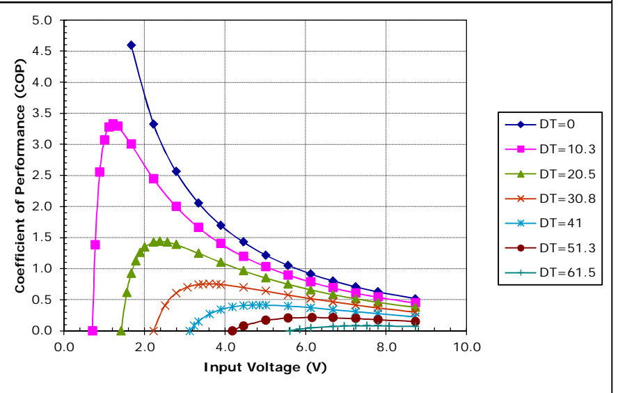
Unpotted TE-71-1.4-2.5 at a hot-side temperature of 30 °C
