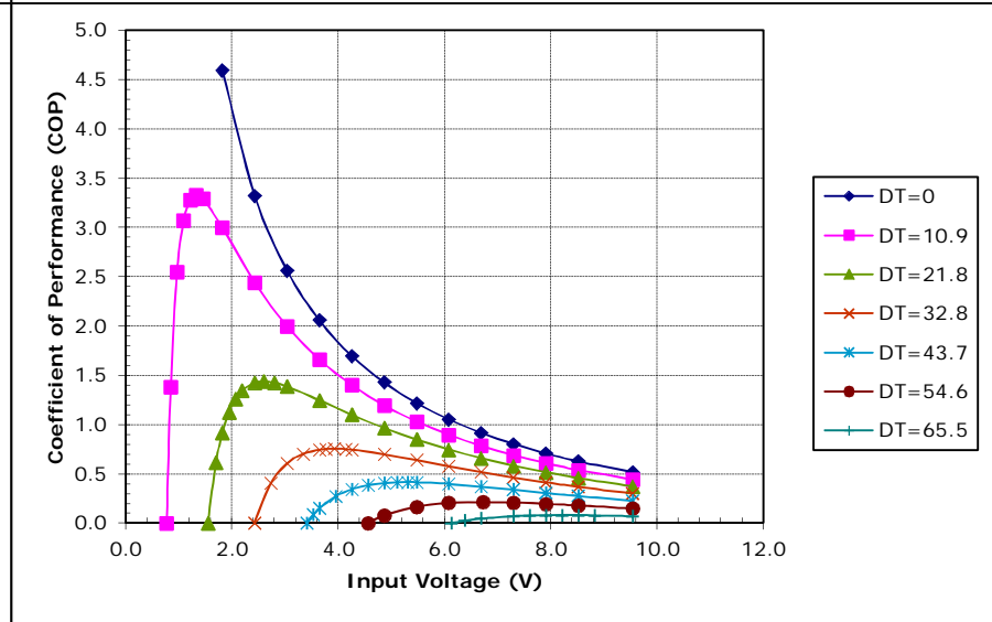
Potted TE-71-1.4-2.5 at a hot-side temperature of 50 °C
