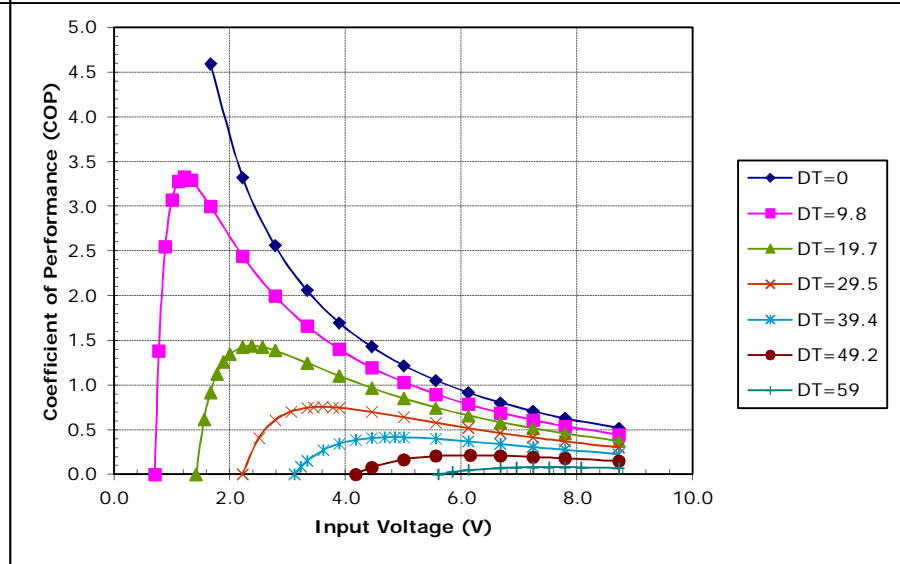
Potted TE-71-1.4-2.5 at a hot-side temperature of 30 °C
