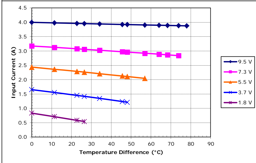
Unpotted TE-71-1.4-2.5 at a hot-side temperature of 50 °C
