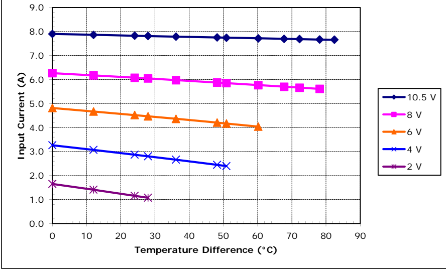
Unpotted TE-71-1.4-1.15 at a hot-side temperature of 70 °C
