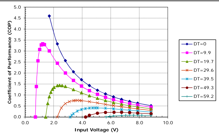
Unpotted TE-71-1.4-1.15 at a hot-side temperature of 30 °C
