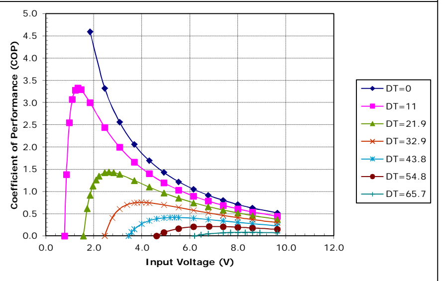
Unpotted TE-71-1.4-1.15 at a hot-side temperature of 50 °C
