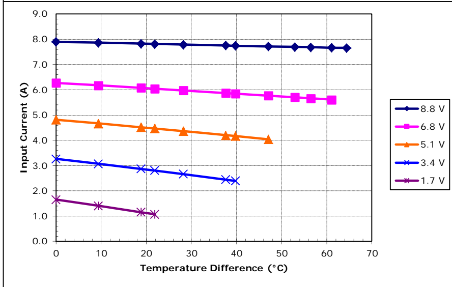
Potted TE-71-1.4-1.15 at a hot-side temperature of 30 °C
