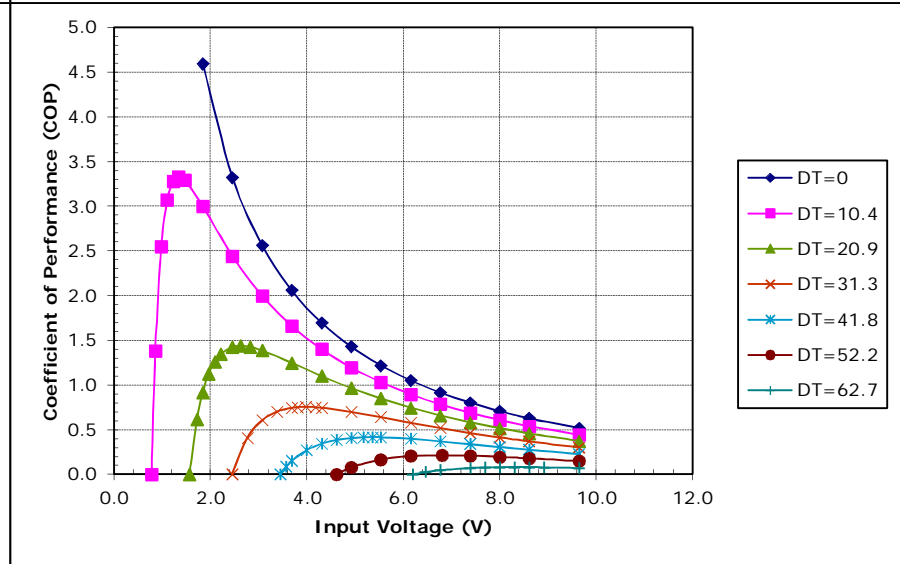
Potted TE-71-1.4-1.15 at a hot-side temperature of 50 °C
