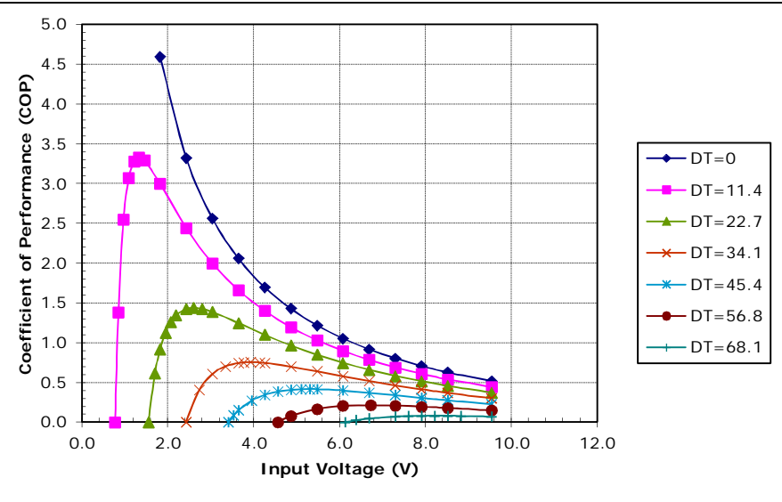
Unpotted TE-71-1.0-2.5 at a hot-side temperature of 50 °C
