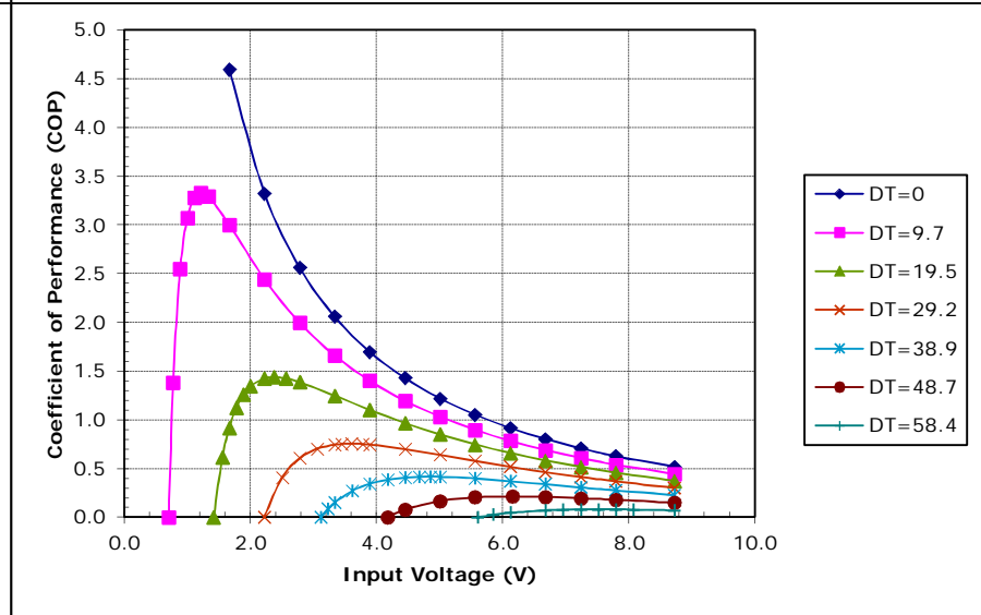
Potted TE-71-1.0-2.5 at a hot-side temperature of 30 °C
