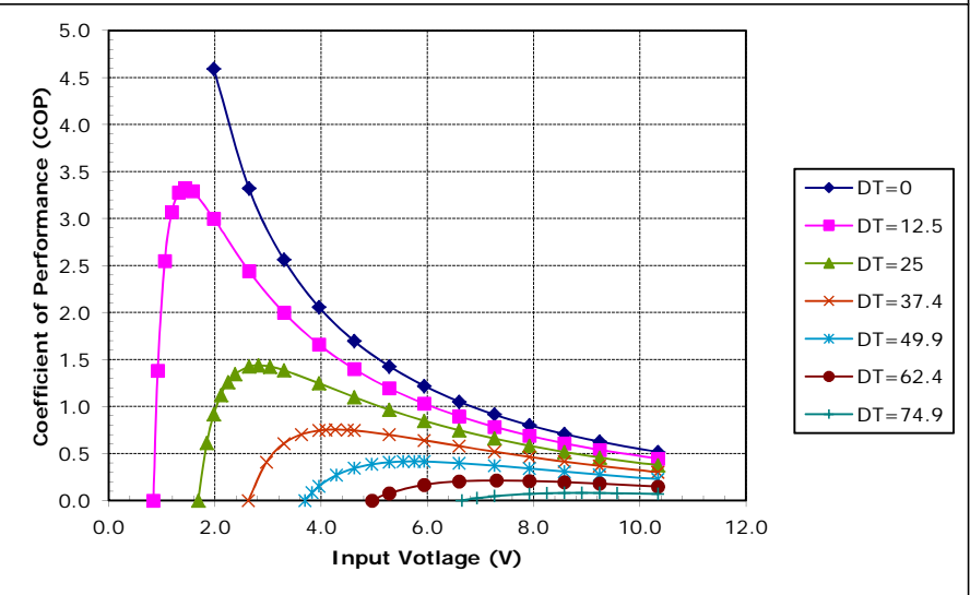
Unpoled TE-71-1.0-2.5 at a hot-side temperature of 70 °C
