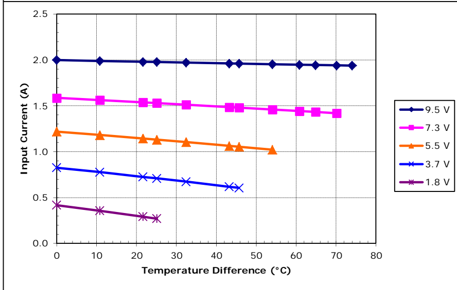
Potted TE-71-1.0-2.5 at a hot-side temperature of 50 °C
