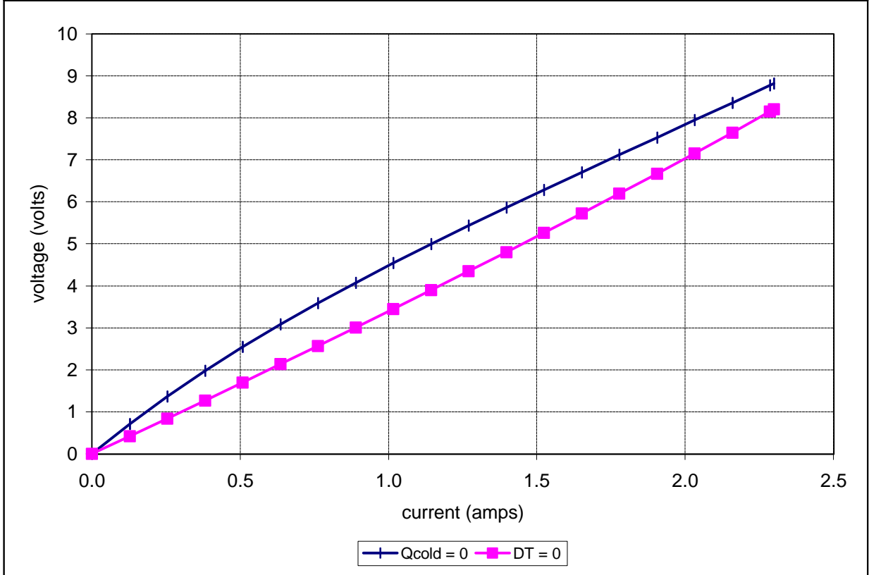
Unpotted TE-71-1.0-2.0 at a hot-side temperature of 25 °C
