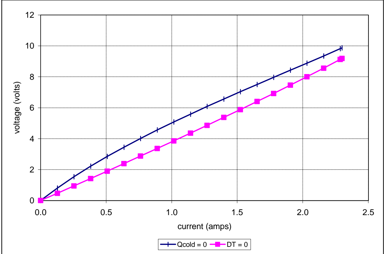
Unpotted TE-71-1.0-2.0 at a hot-side temperature of 50 °C
