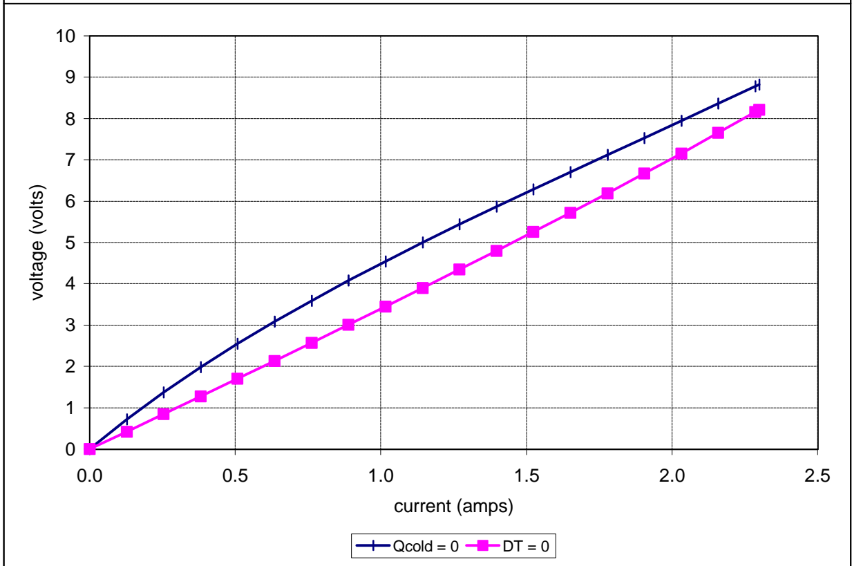
Potted TE-71-1.0-2.0 at a hot-side temperature of 25 °C
