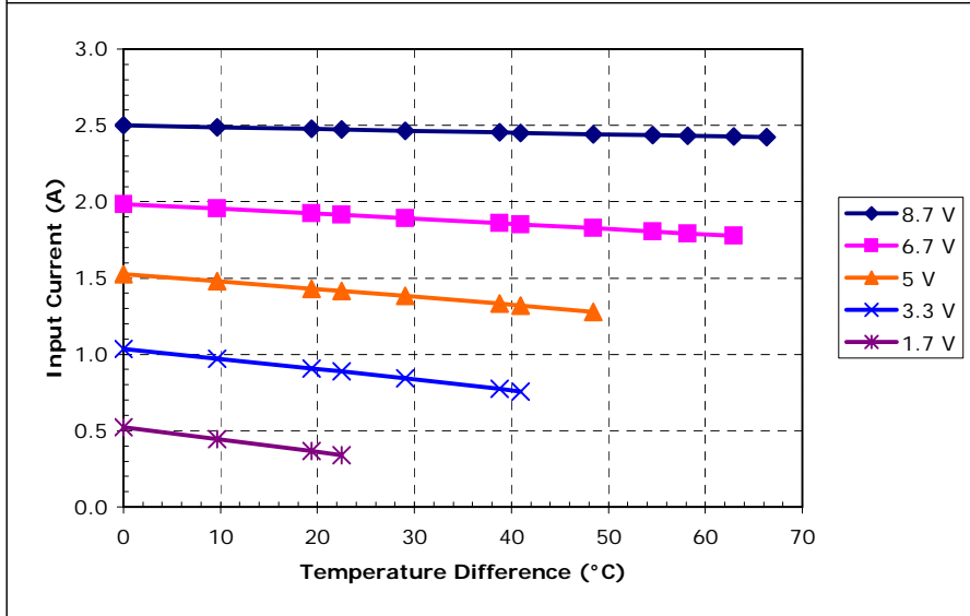
Potted TE-71-1.0-2.0 at a hot-side temperature of 30 °C
