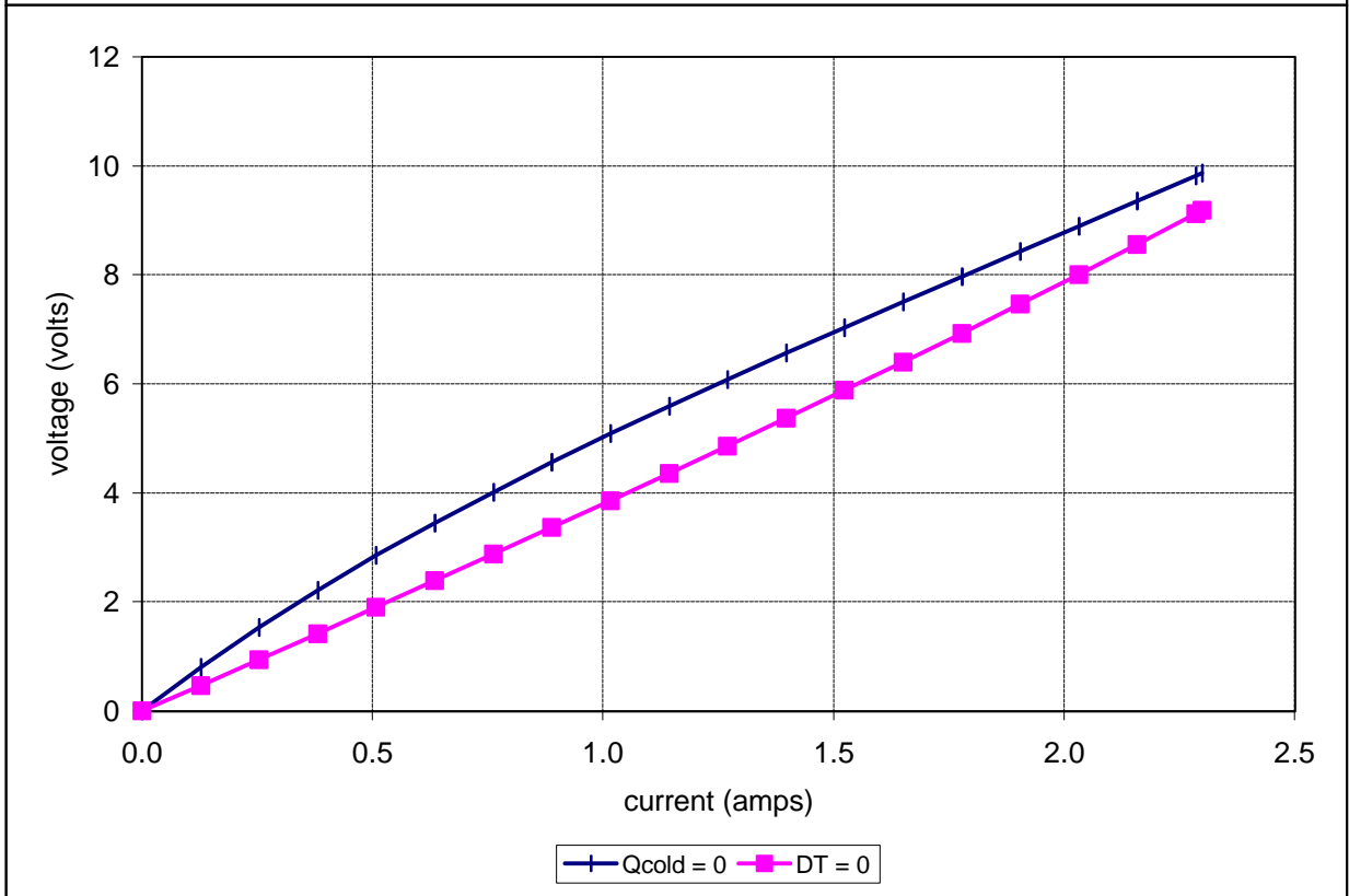
Potted TE-71-1.0-2.0 at a hot-side temperature of 50 °C
