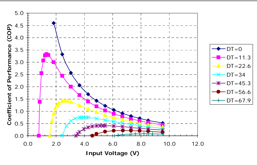
Unpotted TE-71-1.0-2.0 at a hot-side temperature of 50 °C
