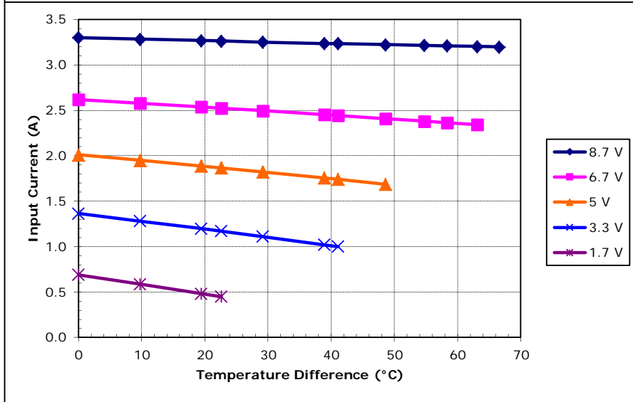
Potted TE-71-1.0-1.5 at a hot-side temperature of 30 °C
