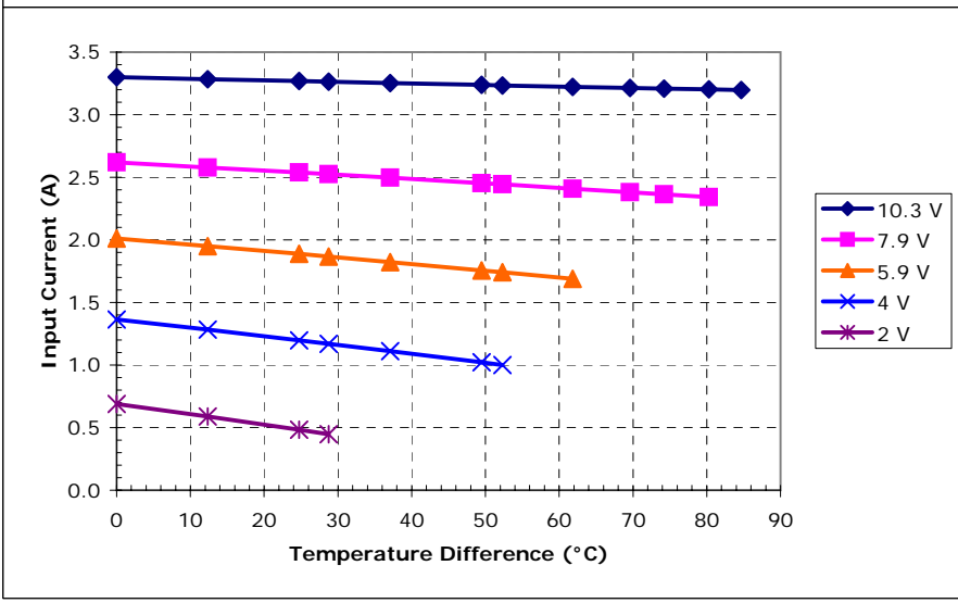
Unpotted TE-71-1.0-1.5 at a hot-side temperature of 70 °C
