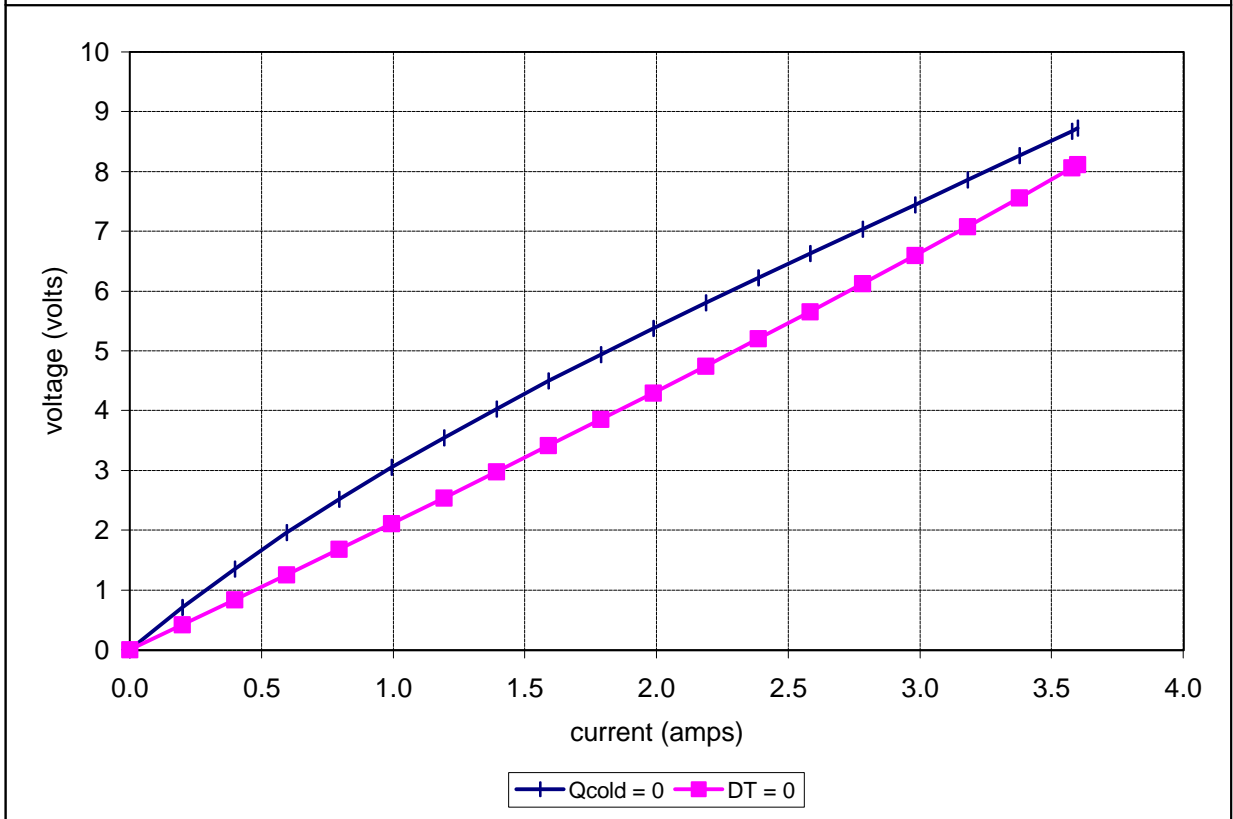
Potted TE-71-1.0-1.3 at a hot-side temperature of 25 °C
