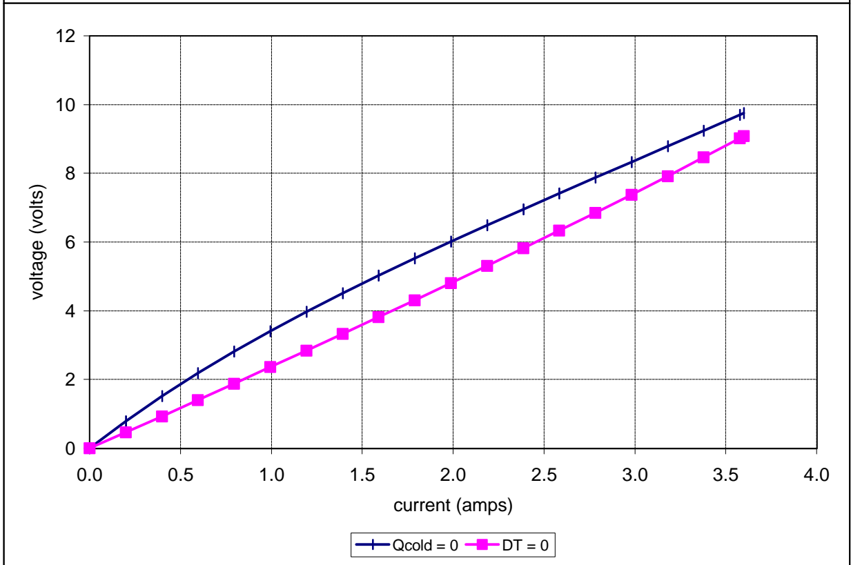
Potted TE-71-1.0-1.3 at a hot-side temperature of 50 °C
