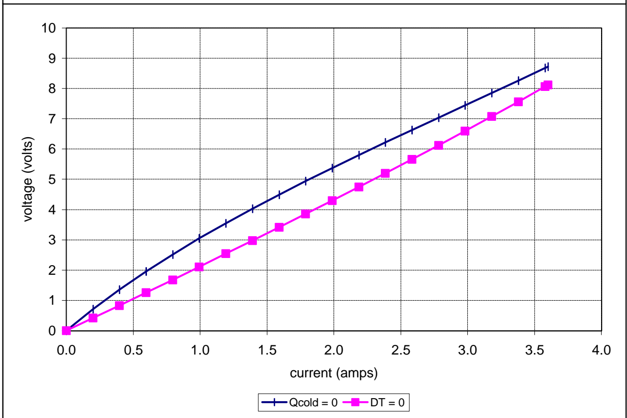
Unpotted TE-71-1.0-1.3 at a hot-side temperature of 25 °C
