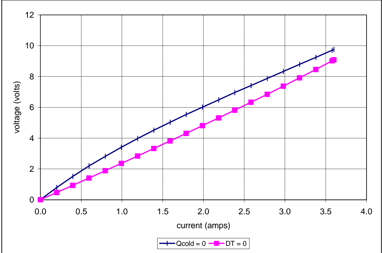
Unpotted TE-71-1.0-1.3 at a hot-side temperature of 50 °C
