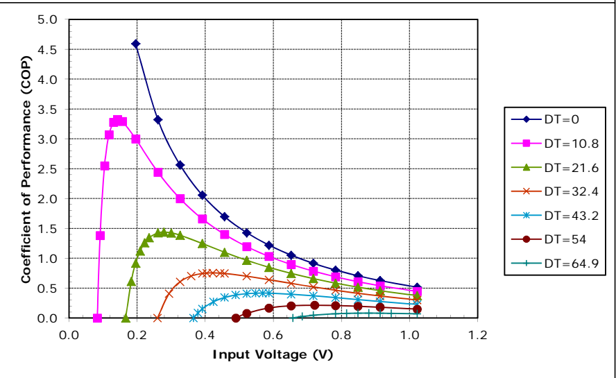
Potted TE-7-2.0-2.5 at a hot-side temperature of 70 °C
