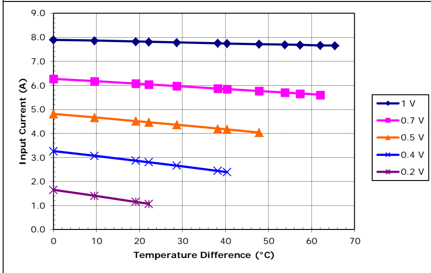
Potted TE-7-1.4-1.15 at a hot-side temperature of 50 °C
