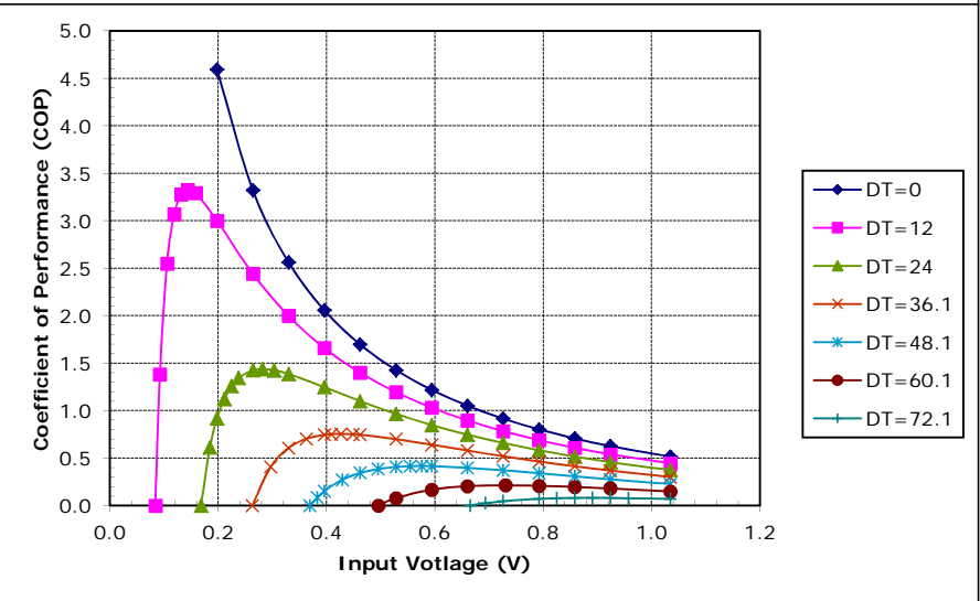
Unpotted TE-7-1.4-1.15 at a hot-side temperature of 70 °C
