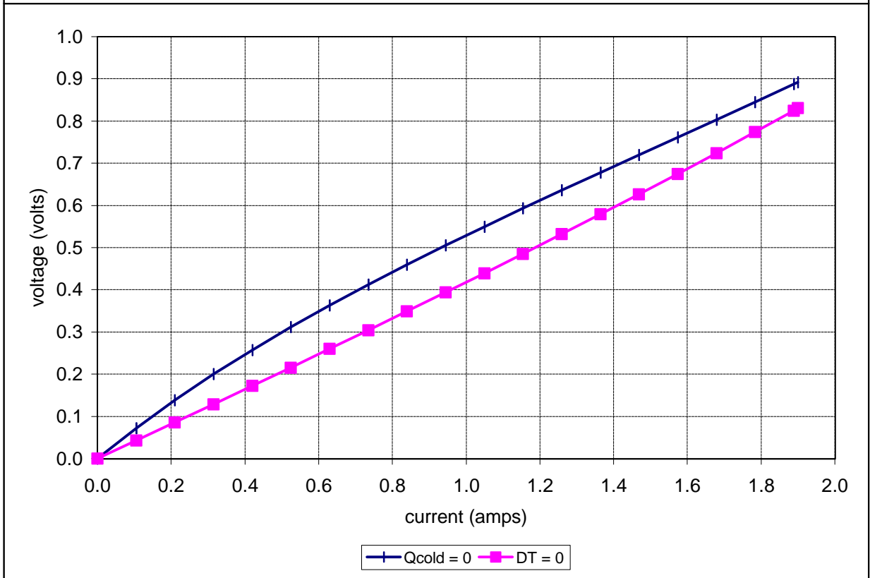
Potted TE-7-1.0-2.5 at a hot-side temperature of 25 °C
