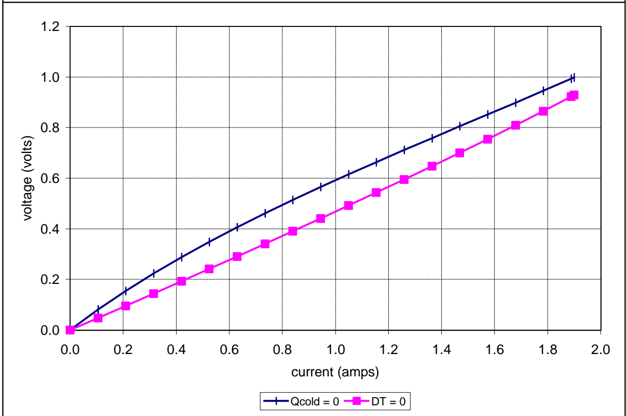
Potted TE-7-1.0-2.5 at a hot-side temperature of 50 °C
