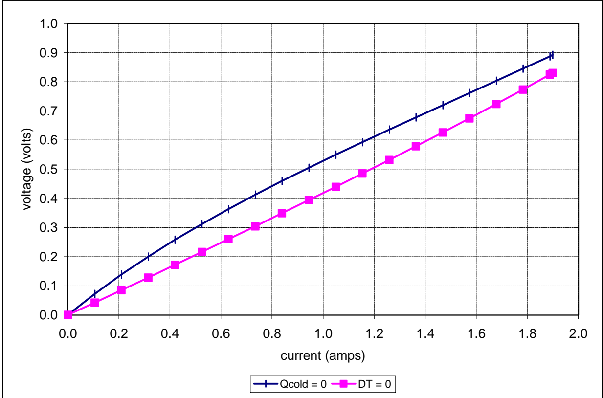
Unpotted TE-7-1.0-2.5 at a hot-side temperature of 25 °C
