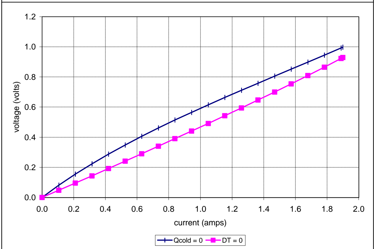
Unpotted TE-7-1.0-2.5 at a hot-side temperature of 50 °C
