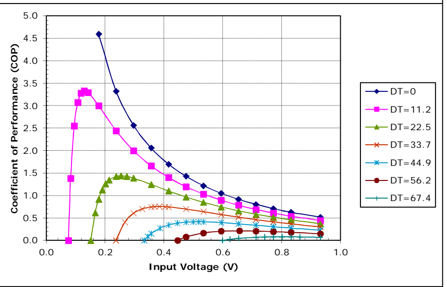
Unpotted TE-7-1.0-2.0 at a hot-side temperature of 50 °C
