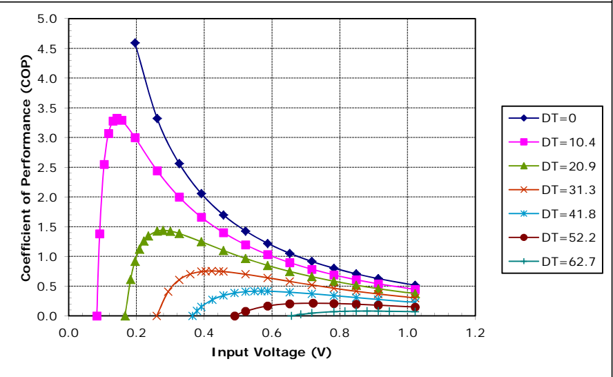
Potted TE-7-1.0-1.5 at a hot-side temperature of 70 °C
