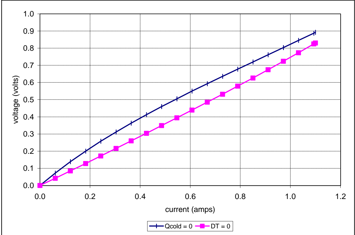
Unpotted TE-7-0.6-1.5 at a hot-side temperature of 25 °C
