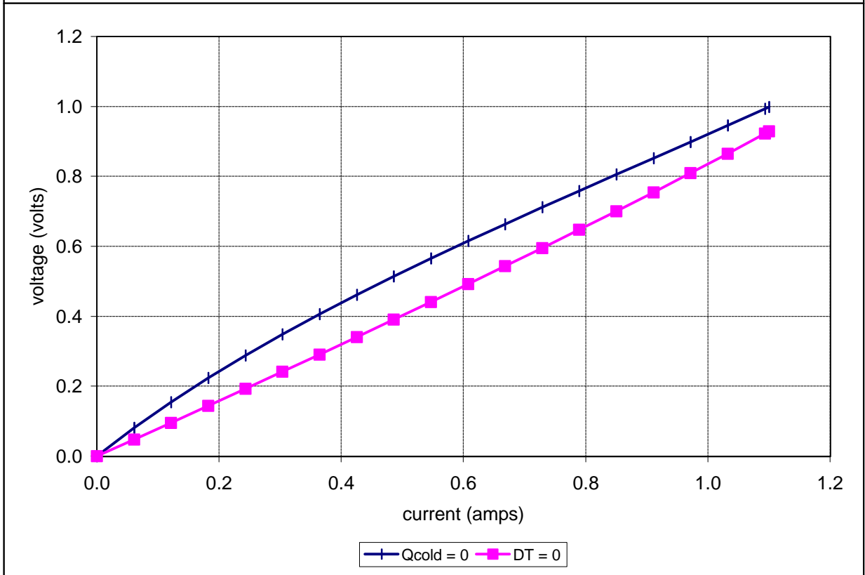
Potted TE-7-0-6-1.5 at a hot-side temperature of 50 °C
