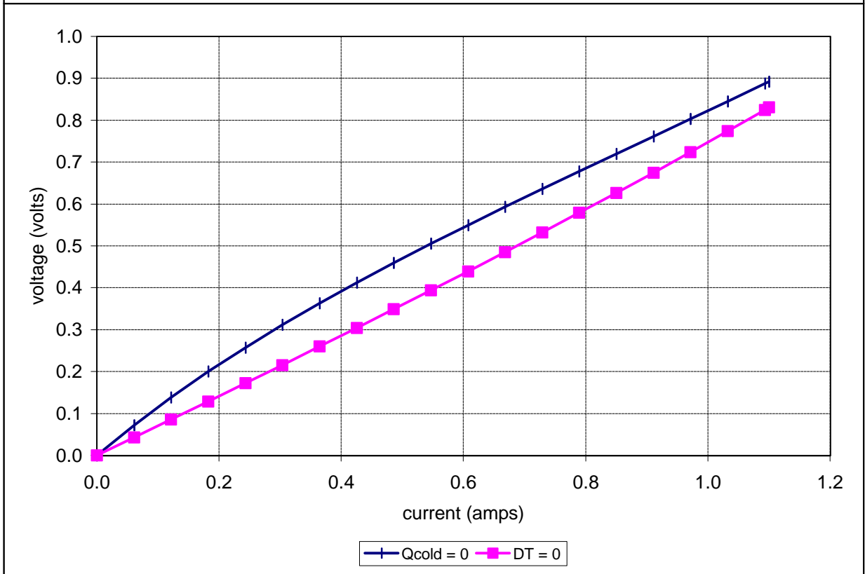
Potted TE-7-0-6-1.5 at a hot-side temperature of 25 °C
