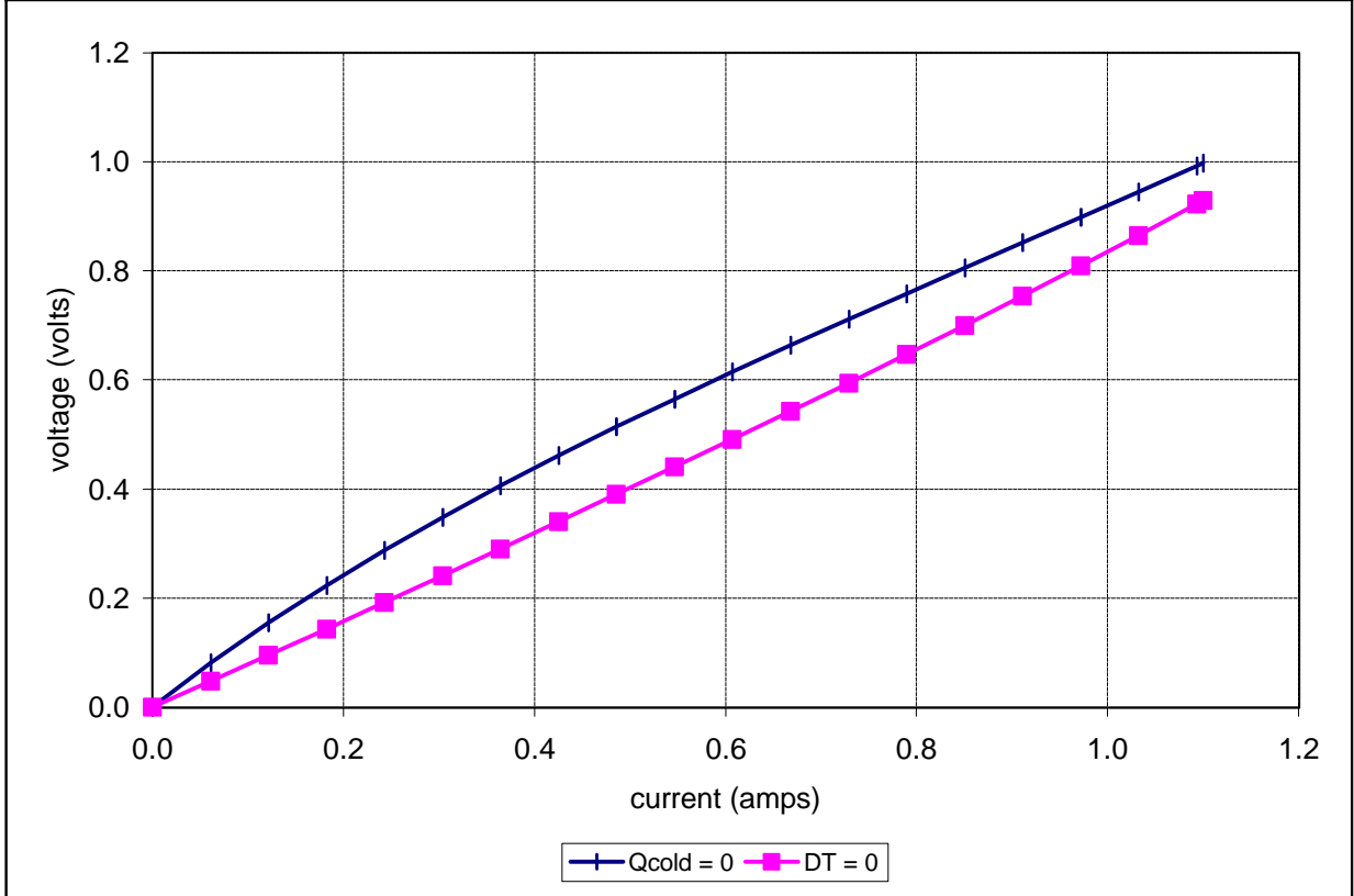
Unpotted TE-7-0.6-1.5 at a hot-side temperature of 50 °C
