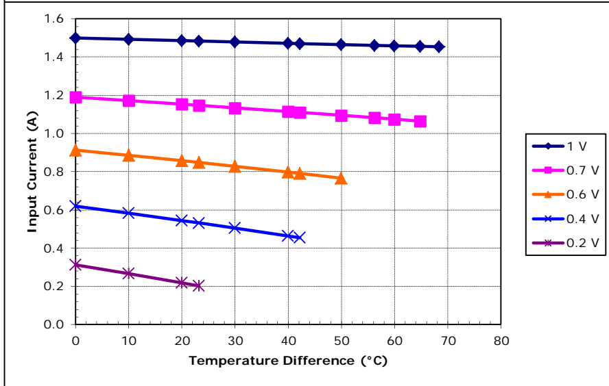
Potted TE-7-0.6-1.2 at a hot-side temperature of 50 °C
