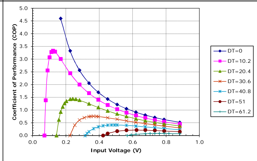
Unpotted TE-7-0.6-1.2 at a hot-side temperature of 30 °C
