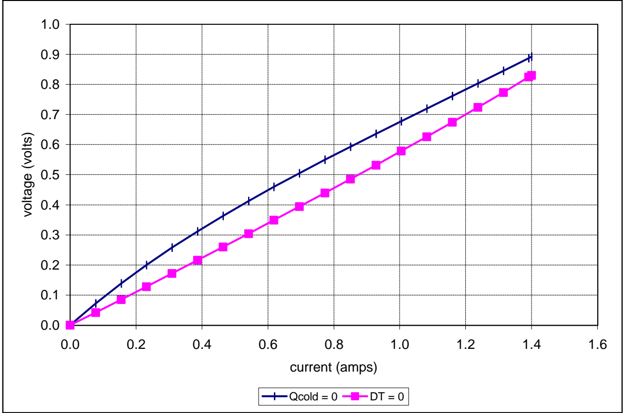
Unpotted TE-7-0.6-1.2 at a hot-side temperature of 25 °C
