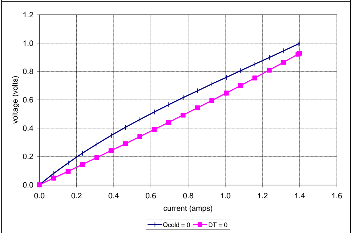
Potted TE-7-0-6-1.2 at a hot-side temperature of 50 °C
