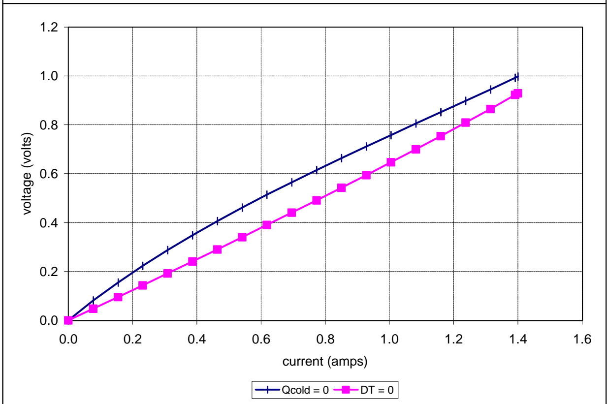
Unpotted TE-7-0.6-1.2 at a hot-side temperature of 50 °C
