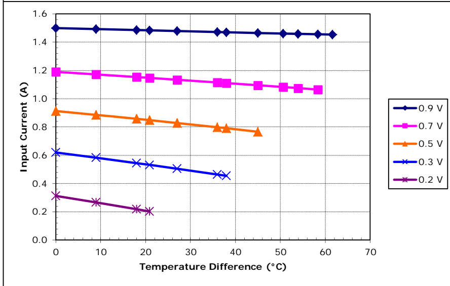
Potted TE-7-0.6-1.2 at a hot-side temperature of 30 °C
