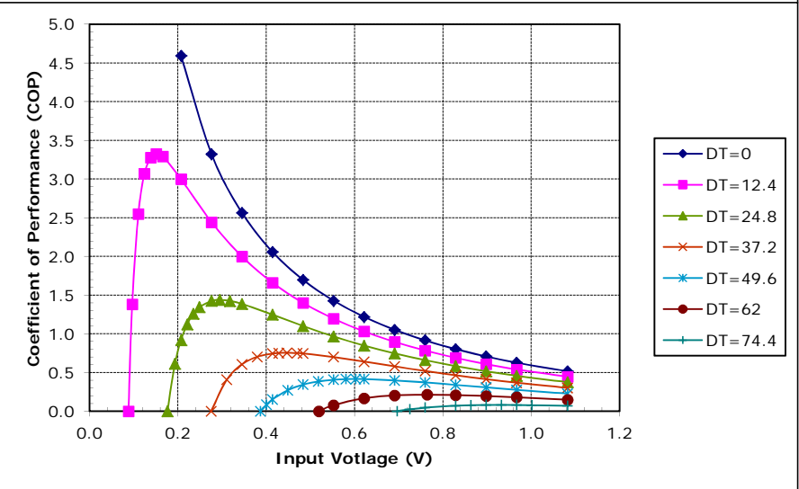
Unpotted TE-7-0.6-1.0 at a hot-side temperature of 70 °C
