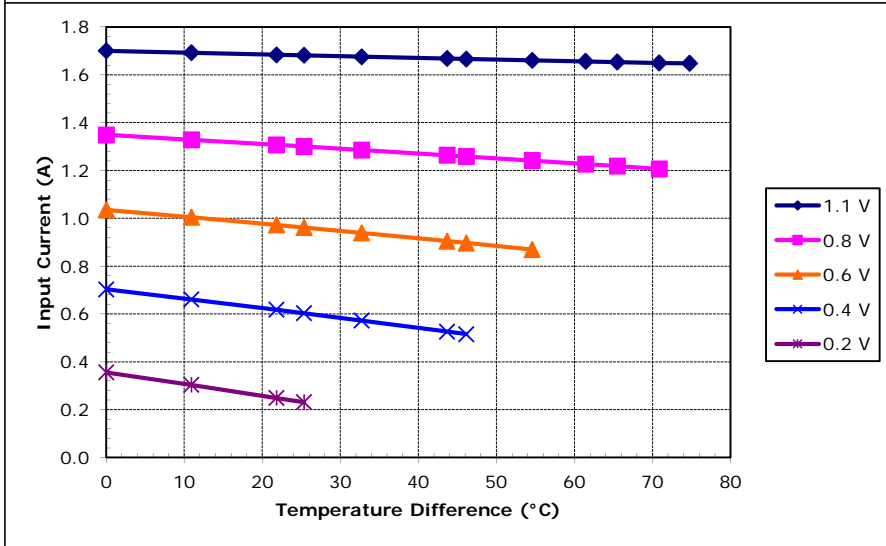
Potted TE-7-0.6-1.0 at a hot-side temperature of 70 °C
