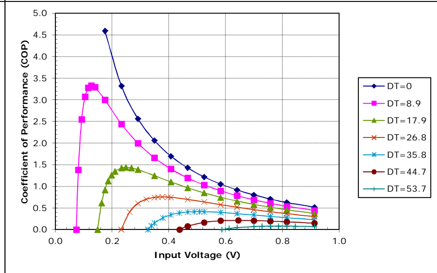
Potted TE-7-0.6-1.0 at a hot-side temperature of 30 °C
