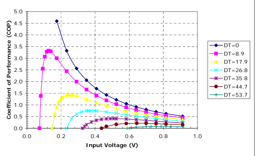
Potted TE-7-0.6-1.0 at a hot-side temperature of 30 °C
