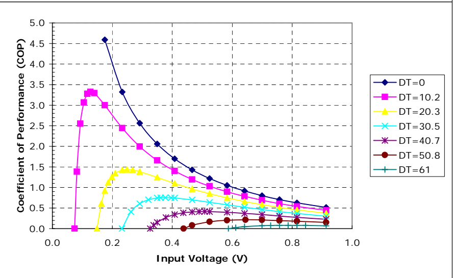
Unpotted TE-7-0.6-1.0 at a hot-side temperature of 30 °C
