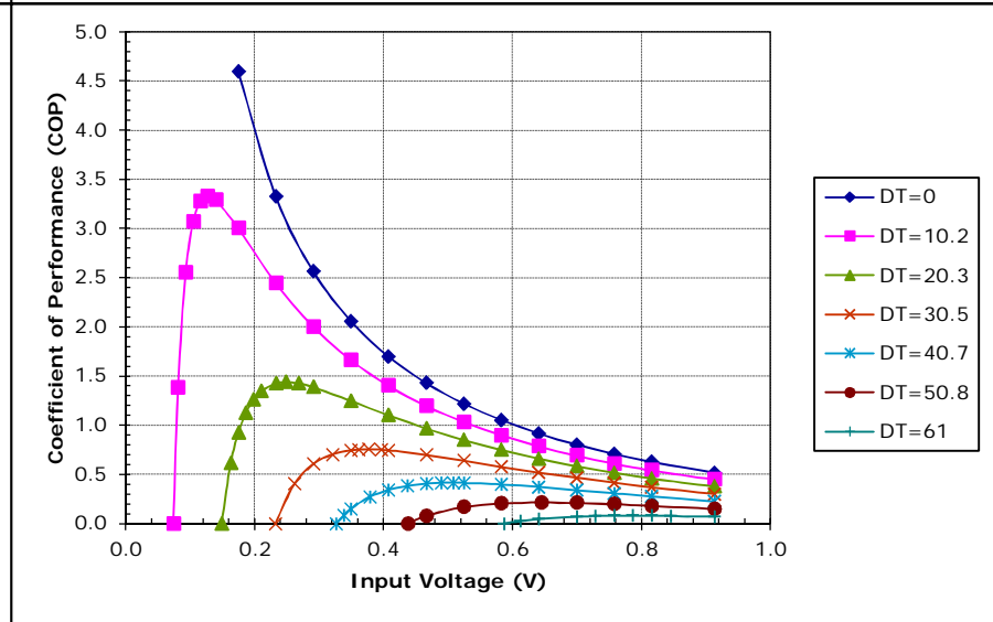
Unpotted TE-7-0.6-1.0 at a hot-side temperature of 30 °C
