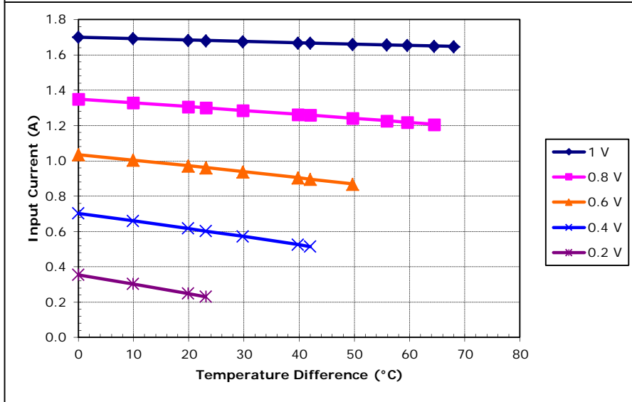
Potted TE-7-0.6-1.0 at a hot-side temperature of 50 °C
