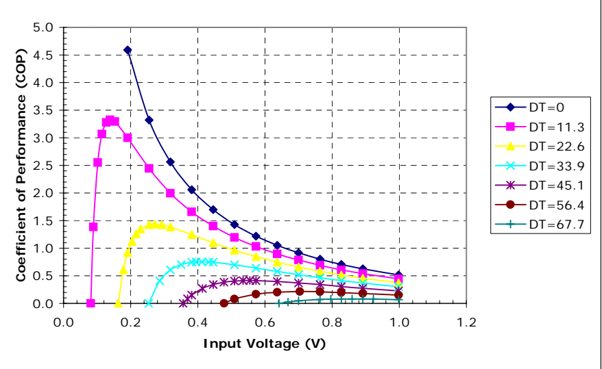
Unpotted TE-7-0.6-1.0 at a hot-side temperature of 50 °C
