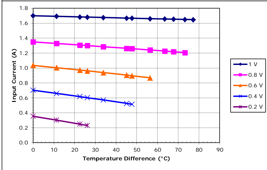
Unpotted TE-7-0.6-1.0 at a hot-side temperature of 50 °C
