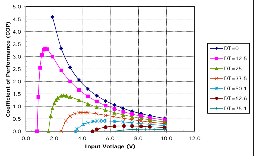
Unpotted TE-66-0.45-1.3 at a hot-side temperature of 70 °C
