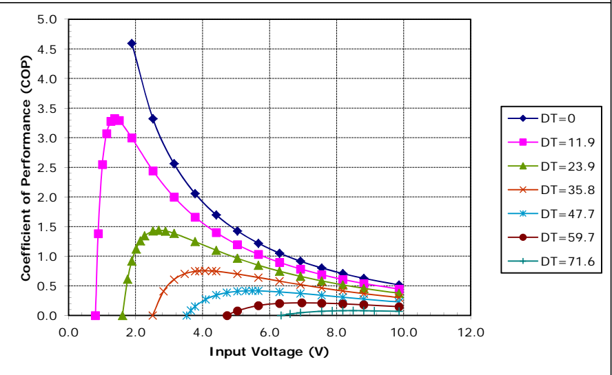
Potted TE-66-0.45-1.3 at a hot-side temperature of 70 °C
