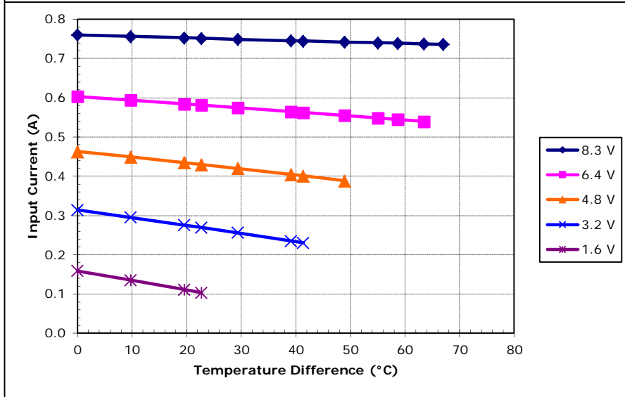
Potted TE-66-0.45-1.3 at a hot-side temperature of 30 °C
