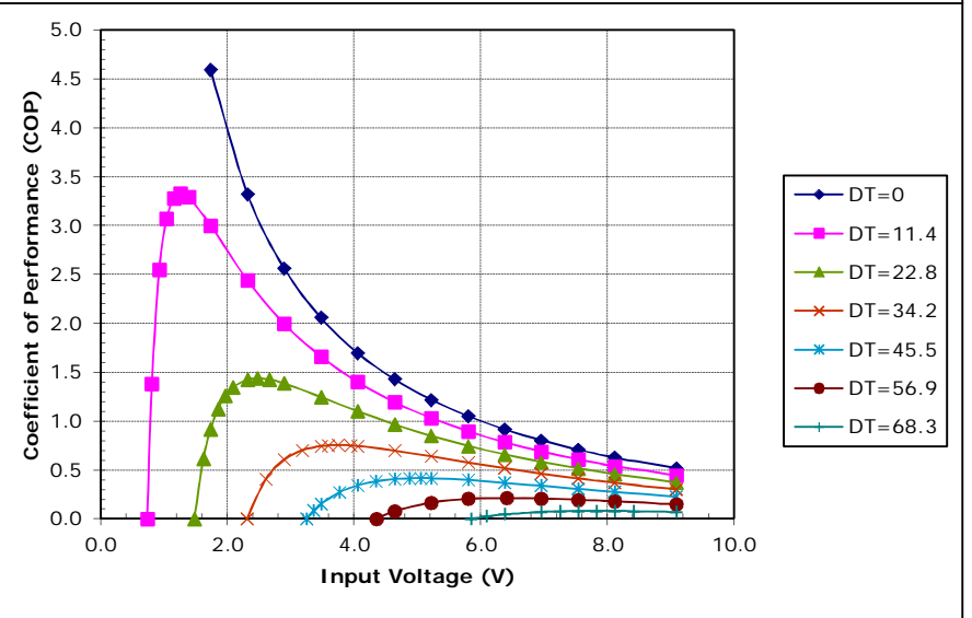
Unpotted TE-66-0.45-1.3 at a hot-side temperature of 50 °C
