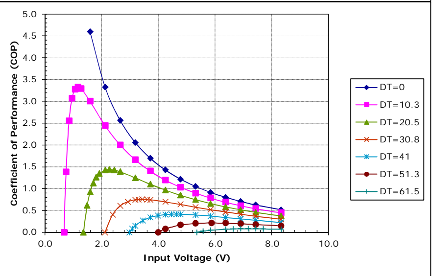
Unpotted TE-66-0.45-1.3 at a hot-side temperature of 30 °C
