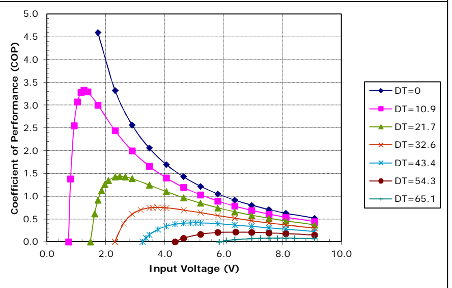
Potted TE-66-0.45-1.3 at a hot-side temperature of 50 °C
