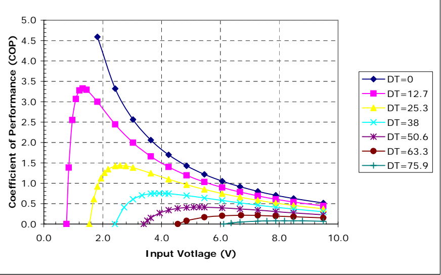
Unpotted TE-65-0.6-1.5 at a hot-side temperature of 70 °C
