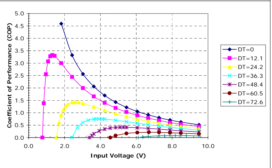
Potted TE-65-0.6-1.5 at a hot-side temperature of 70 °C
