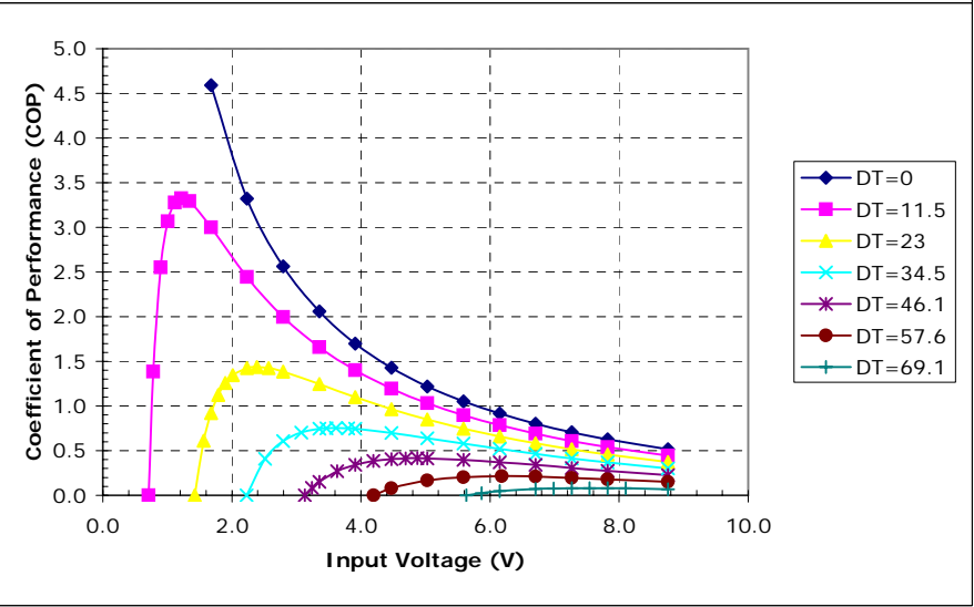
Unpotted TE-65-0.6-1.5 at a hot-side temperature of 50 °C
