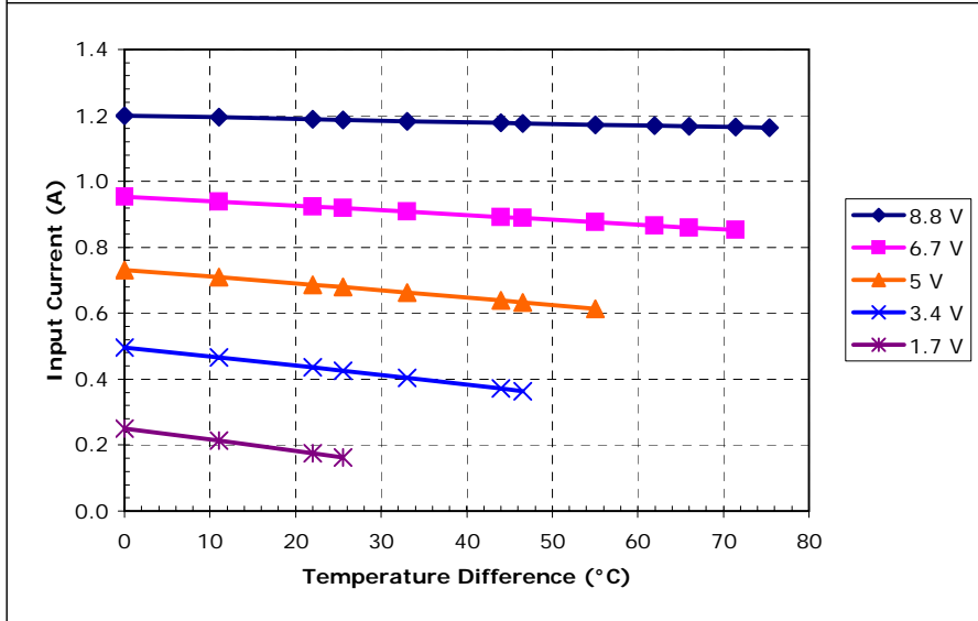
Potted TE-65-0.6-1.5 at a hot-side temperature of 50 °C
