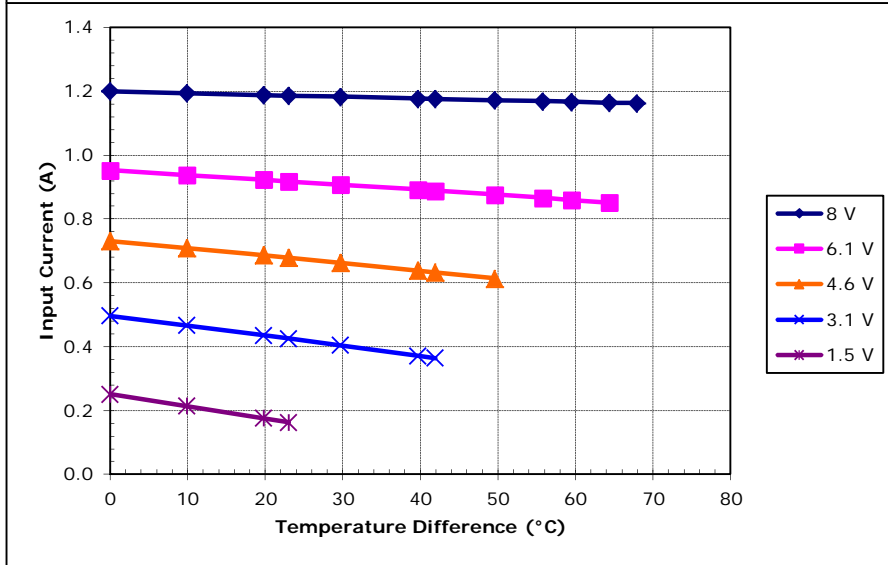
Potted TE-65-0.6-1.5 at a hot-side temperature of 30 °C
