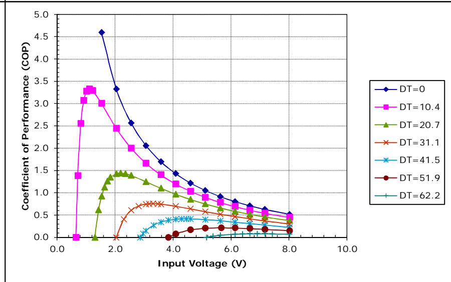
Unpotted TE-65-0.6-1.5 at a hot-side temperature of 30 °C
