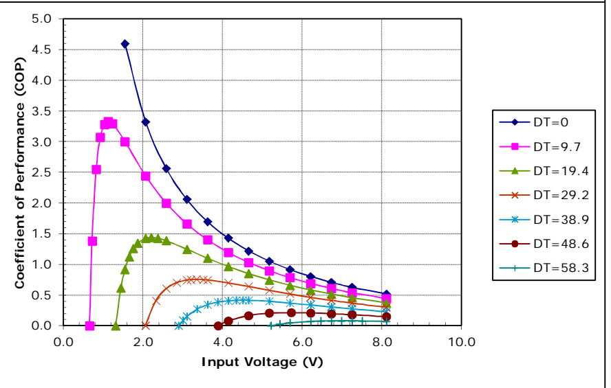
Potted TE-65-0.6-1.2 at a hot-side temperature of 30 °C
