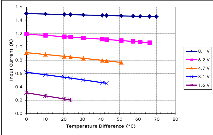
Unpotted TE-65-0.6-1.2 at a hot-side temperature of 30 °C
