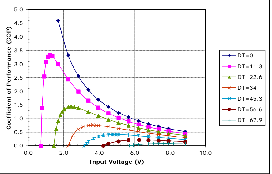
Unpotted TE-65-0.6-1.2 at a hot-side temperature of 50 °C
