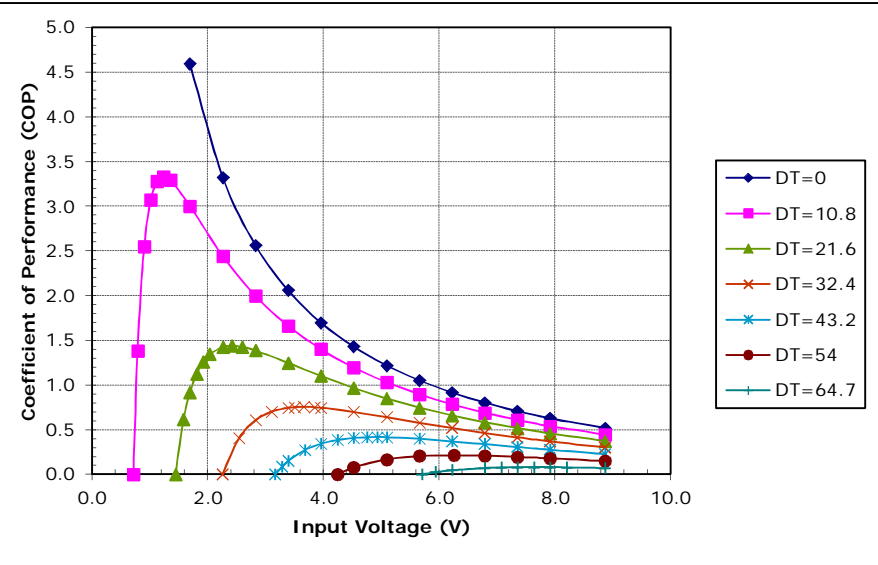
Potted TE-65-0.6-1.2 at a hot-side temperature of 50 °C
