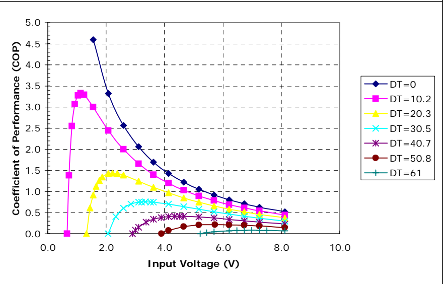
Unpotted TE-65-0.6-1.0 at a hot-side temperature of 30 °C
