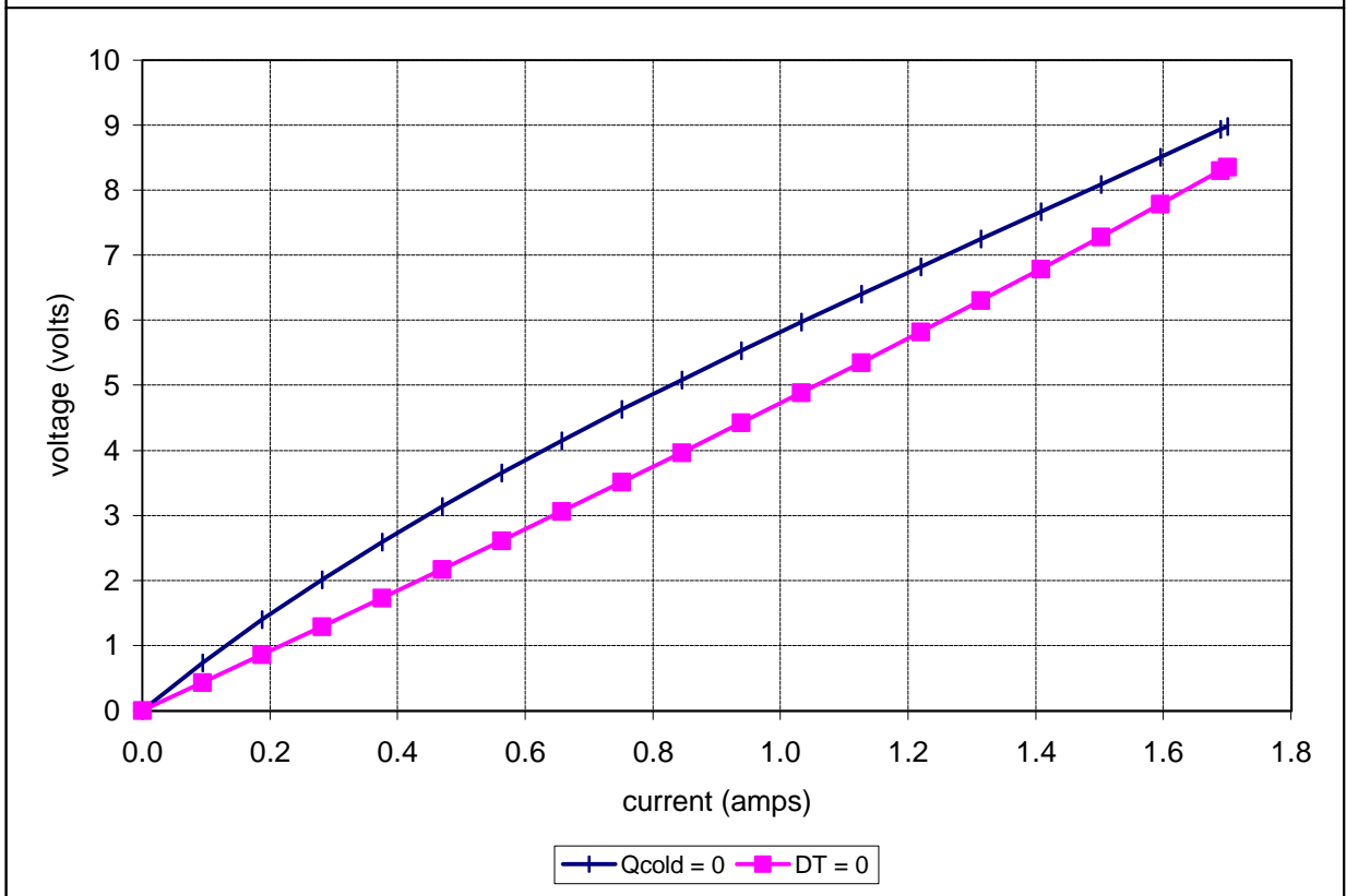
Unpotted TE-65-0.6-1.0 at a hot-side temperature of 50 °C
