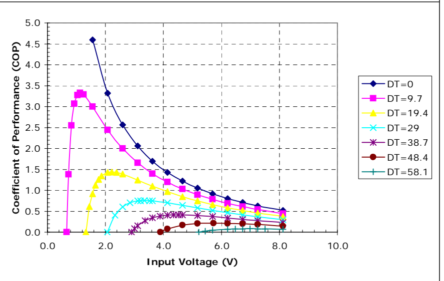
Potted TE-65-0.6-1.0 at a hot-side temperature of 30 °C
