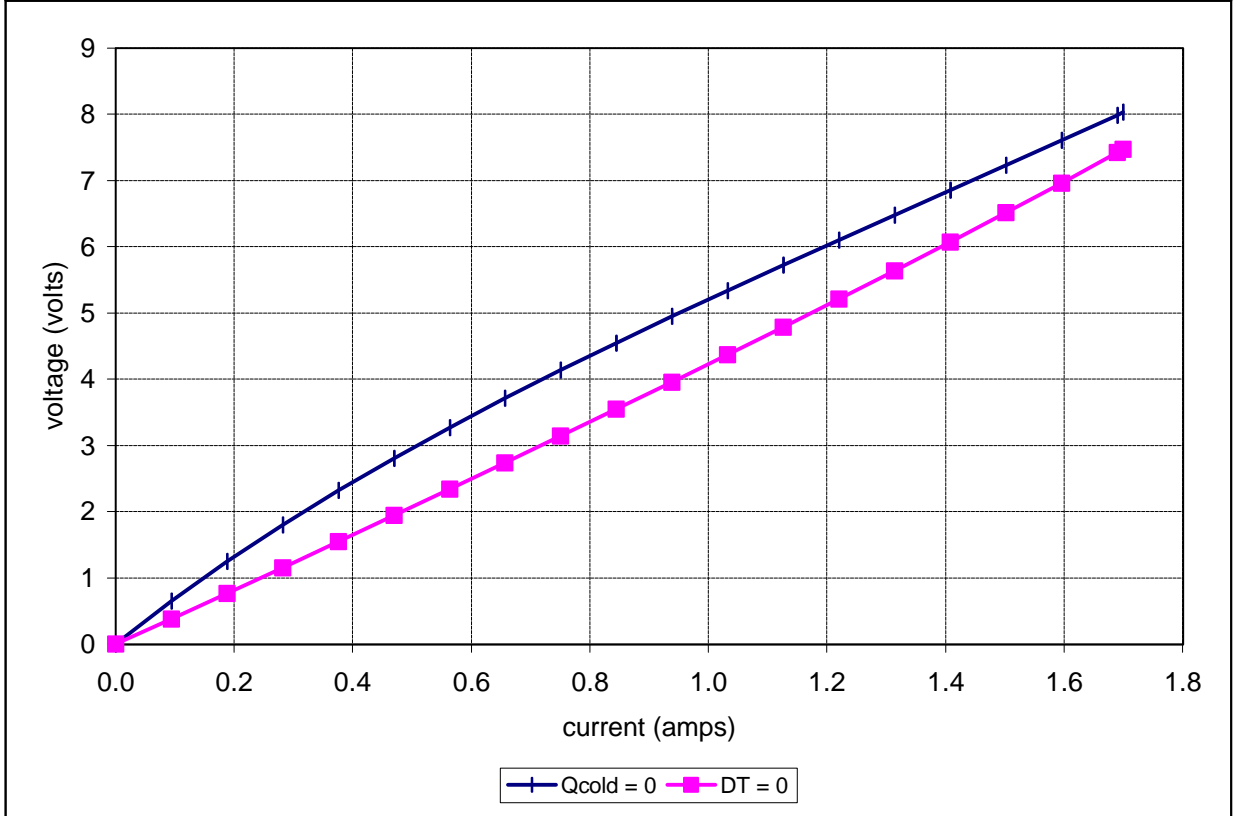
Unpotted TE-65-0.6-1.0 at a hot-side temperature of 25 °C
