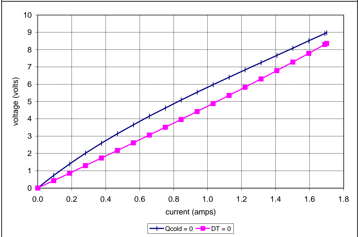
Potted TE-65-0.6-1.0 at a hot-side temperature of 50 °C
