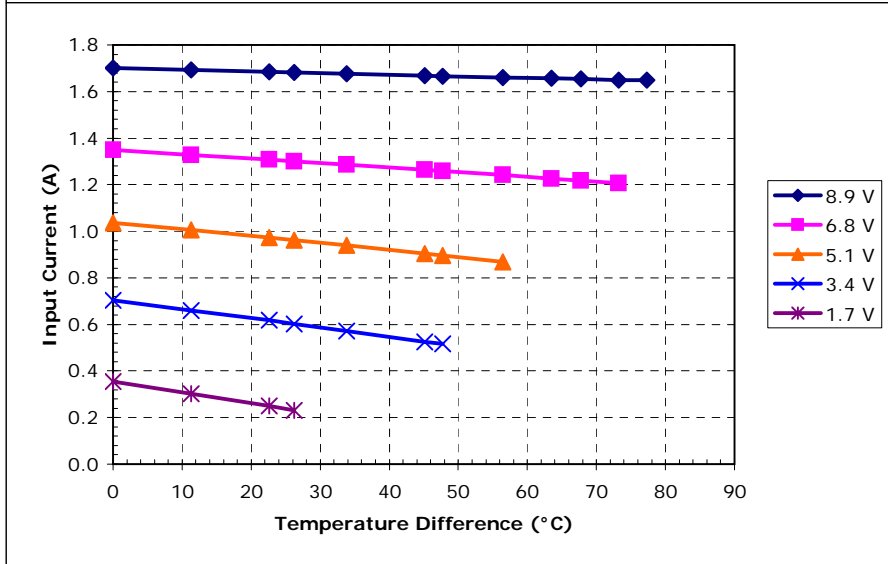
Unpotted TE-65-0.6-1.0 at a hot-side temperature of 50 °C
