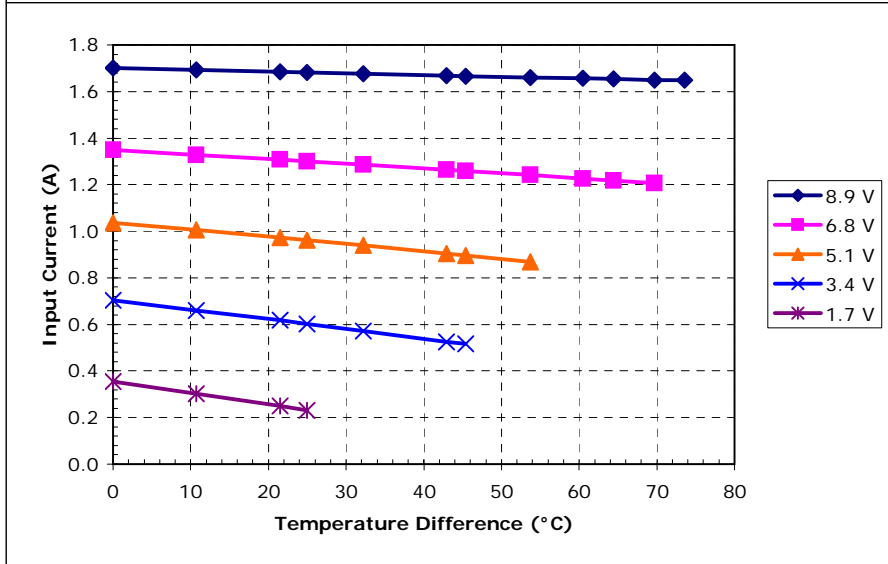
Potted TE-65-0.6-1.0 at a hot-side temperature of 50 °C
