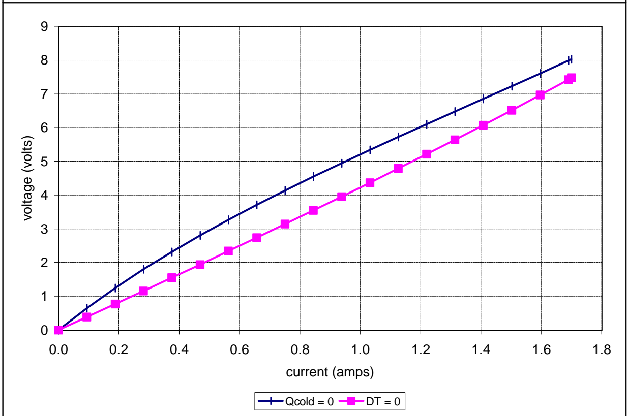
Potted TE-65-0.6-1.0 at a hot-side temperature of 25 °C
