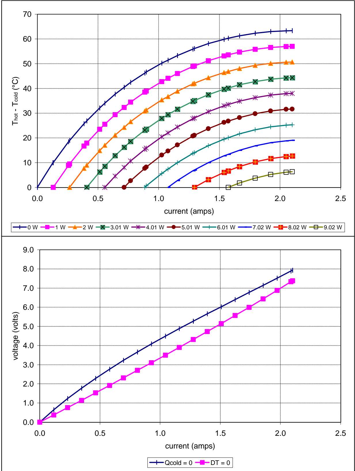
Potted TE-65-0.6-0.8 at a hot-side temperature of 25 °C
