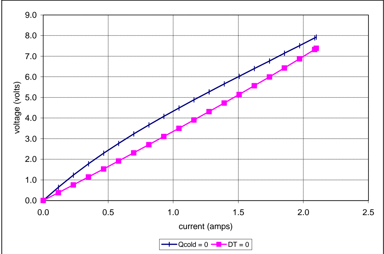
Unpotted TE-65-0.6-0.8 at a hot-side temperature of 25 °C
