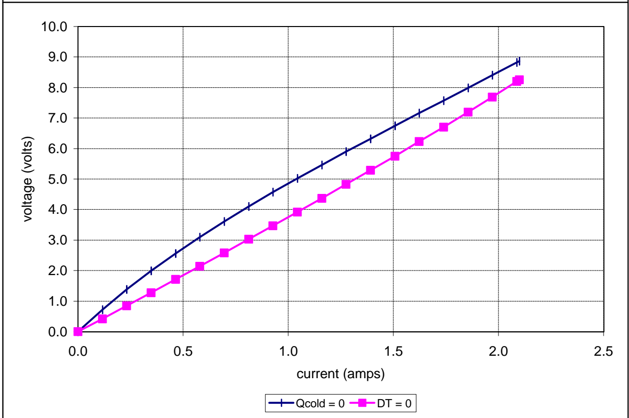
Potted TE-65-0.6-0.8 at a hot-side temperature of 50 °C
