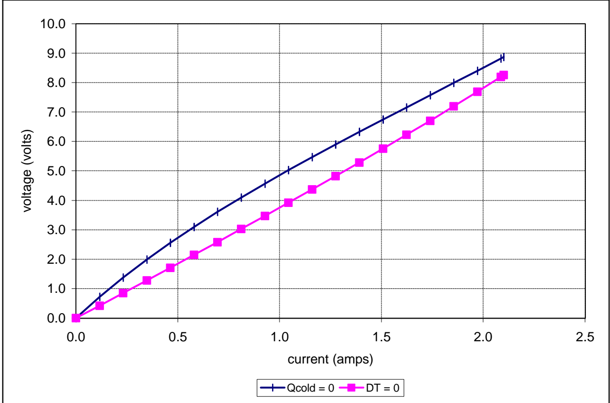
Unpotted TE-65-0.6-0.8 at a hot-side temperature of 50 °C
