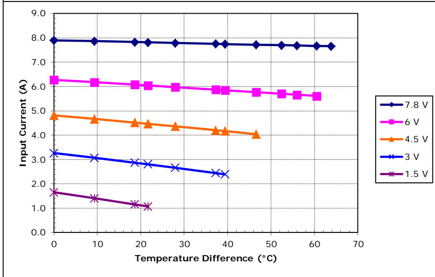
Potted TE-63-1.4-1.15 at a hot-side temperature of 30 °C
