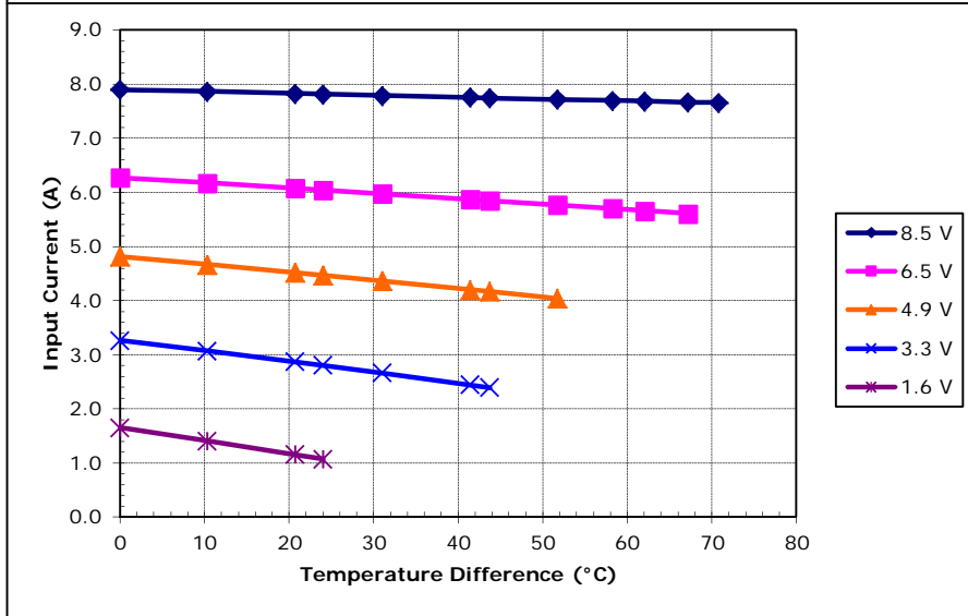
Potted TE-63-1.4-1.15 at a hot-side temperature of 50 °C
