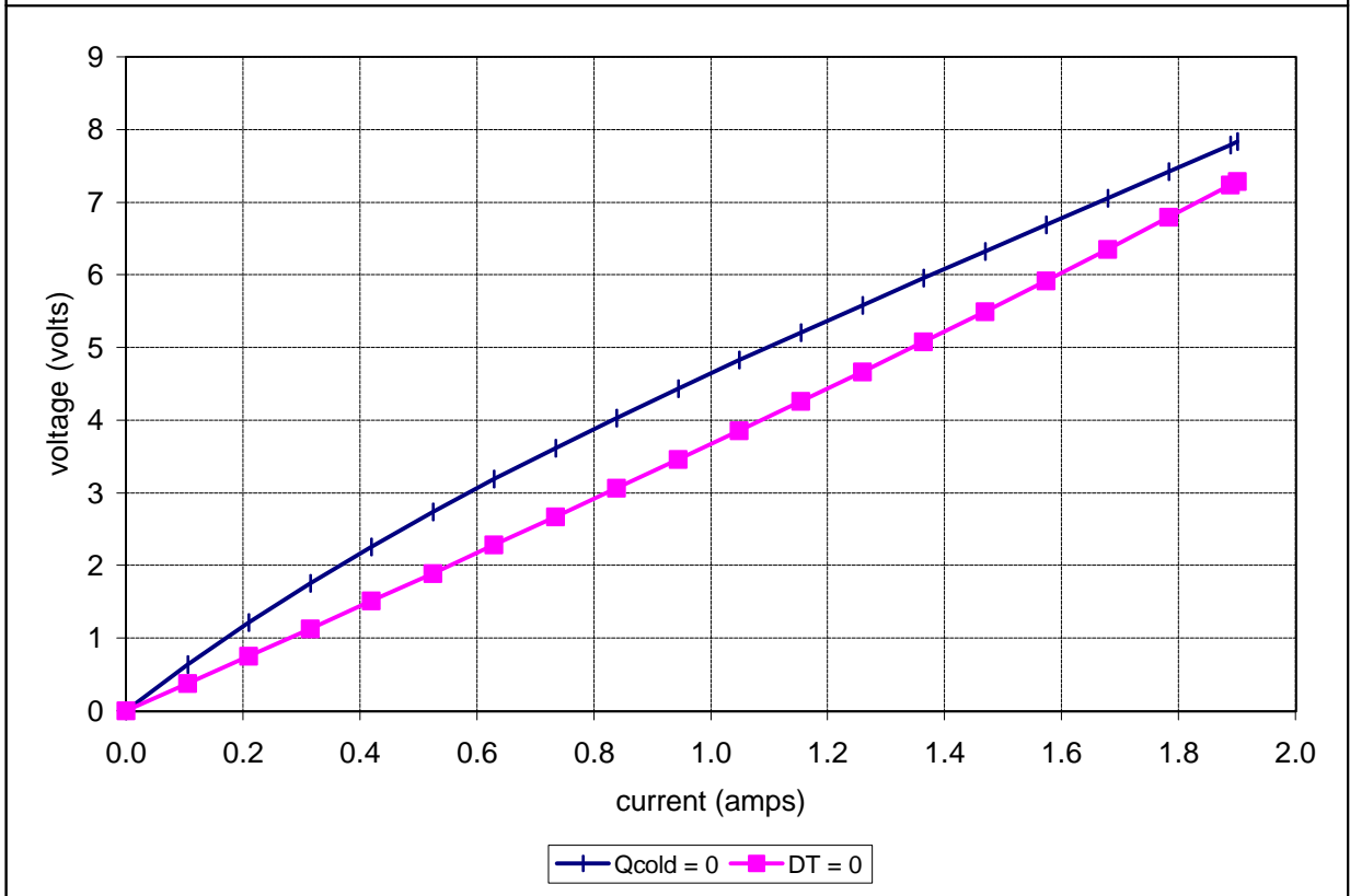
Potted TE-63-1.0-2.5 at a hot-side temperature of 25 °C
