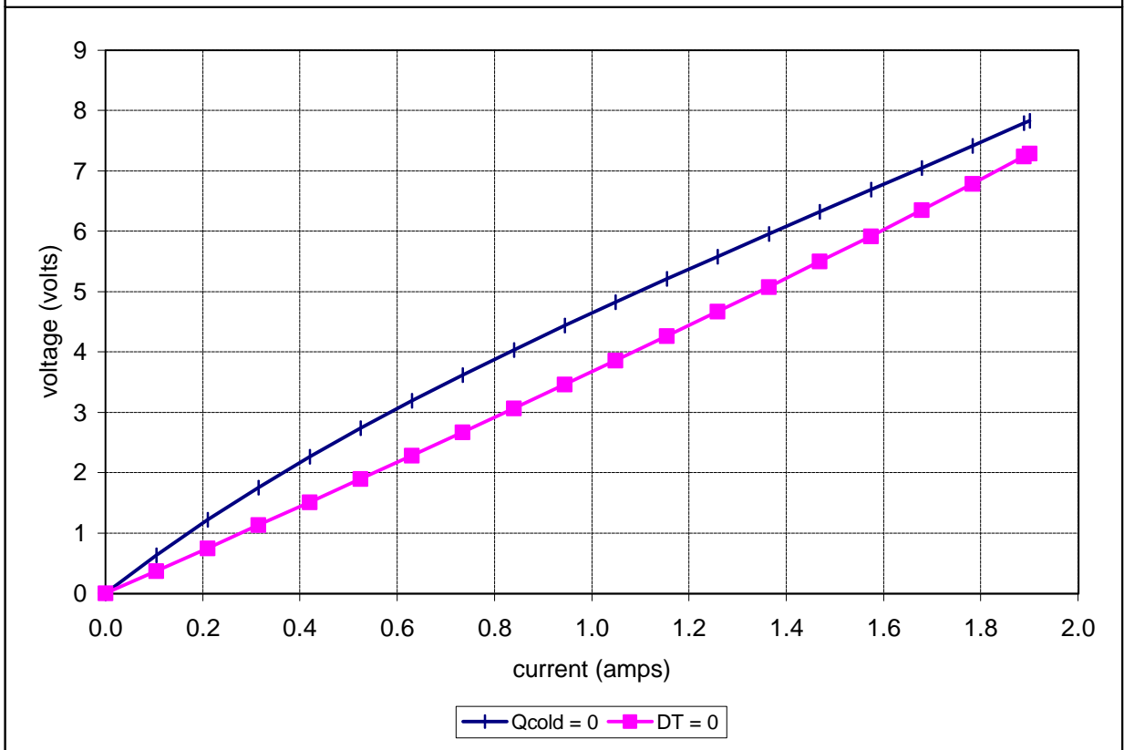
Unpotted TE-63-1.0-2.5 at a hot-side temperature of 25 °C
