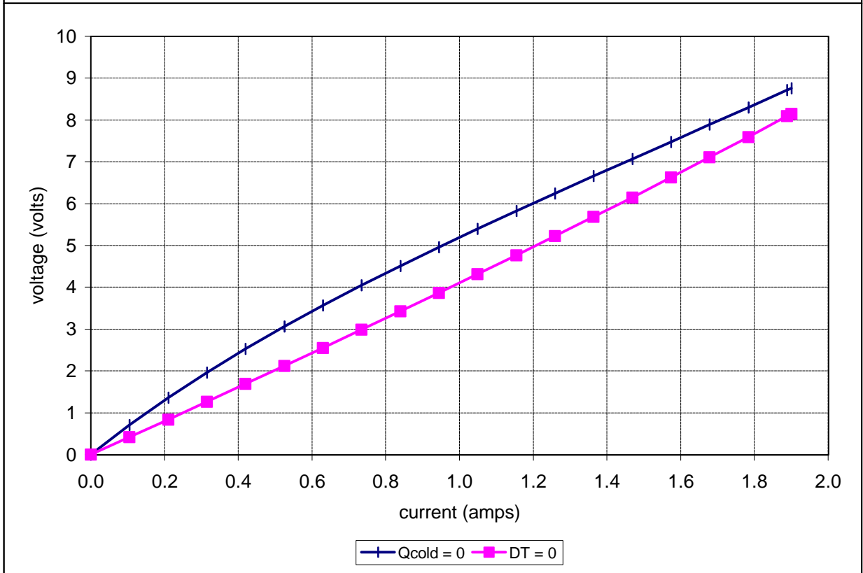
Potted TE-63-1.0-2.5 at a hot-side temperature of 50 °C
