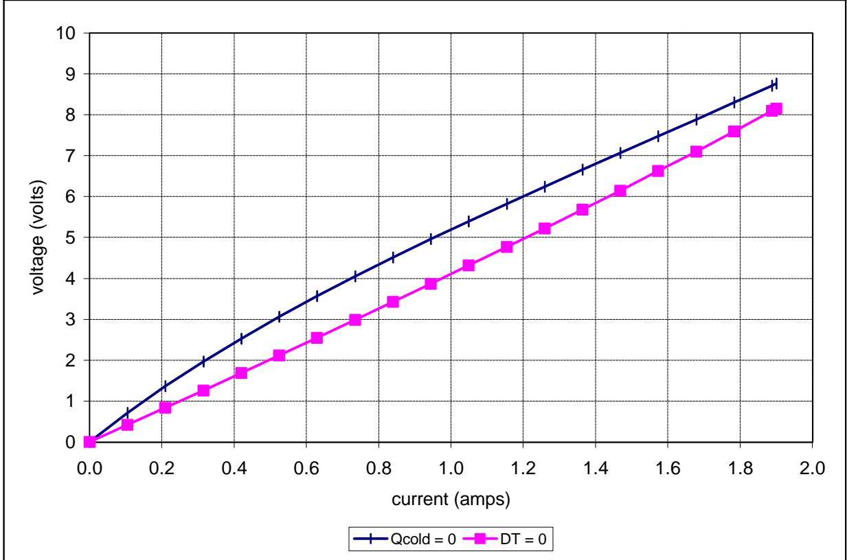
Unpotted TE-63-1.0-2.5 at a hot-side temperature of 50 °C
