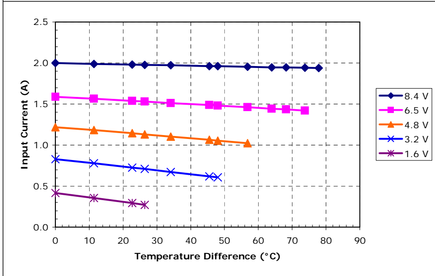
Unpotted TE-63-1.0-2.5 at a hot-side temperature of 50 °C
