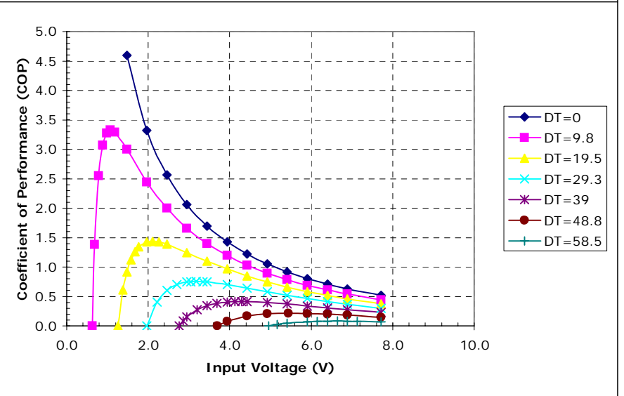
Potted TE-63-1.0-2.5 at a hot-side temperature of 30 °C
