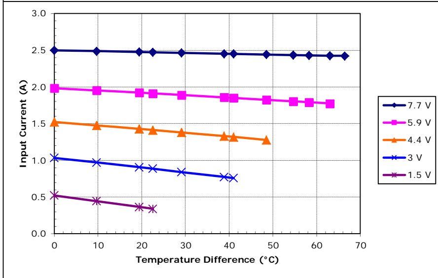
Potted TE-63-1.0-2.0 at a hot-side temperature of 30 °C
