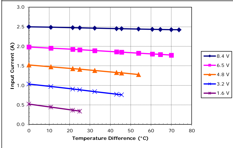
Potted TE-63-1.0-2.0 at a hot-side temperature of 50 °C
