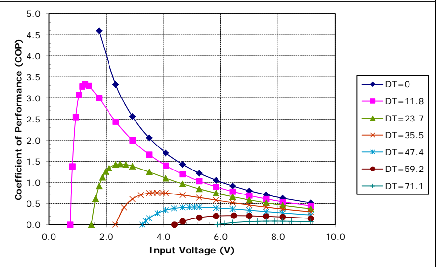
Potted TE-63-1.0-2.0 at a hot-side temperature of 70 °C
