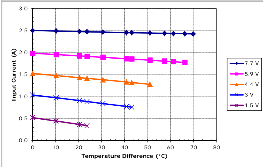
Unpotted TE-63-1.0-2.0 at a hot-side temperature of 30 °C
