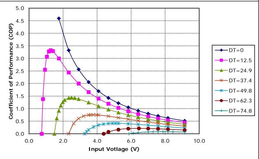
Unpotted TE-63-1.0-2.0 at a hot-side temperature of 70 °C
