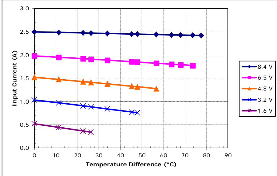
Unpotted TE-63-1.0-2.0 at a hot-side temperature of 50 °C
