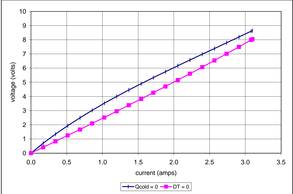
Unpotted TE-63-1.0-1.5 at a hot-side temperature of 50 °C
