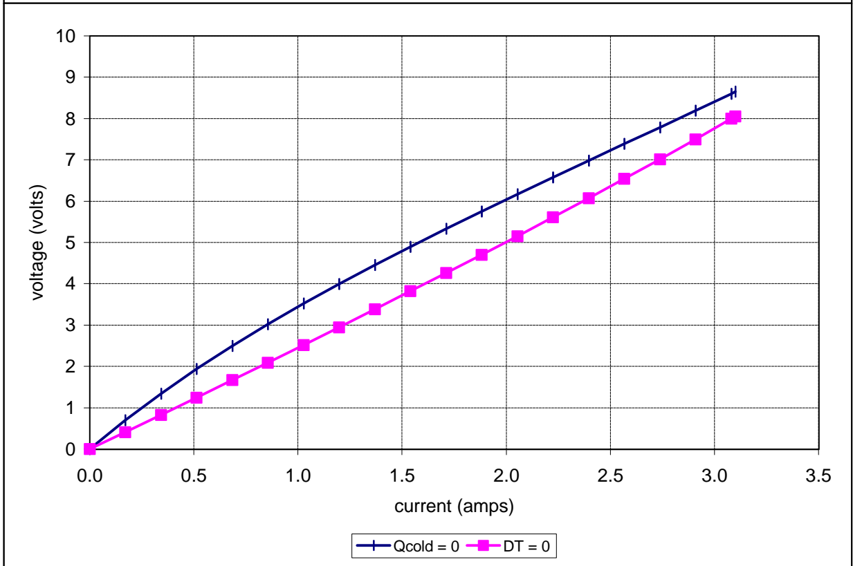
Potted TE-63-1.0-1.5 at a hot-side temperature of 50 °C
