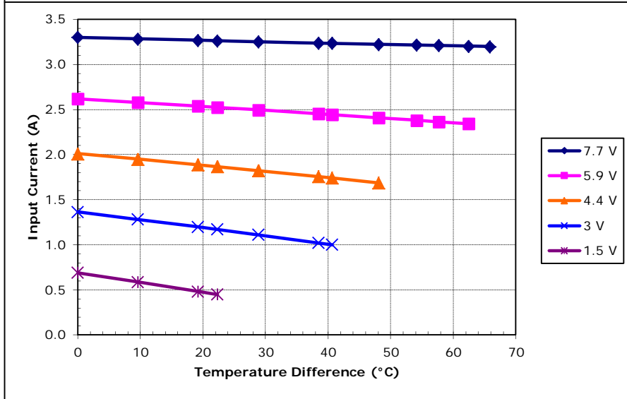
Potted TE-63-1.0-1.5 at a hot-side temperature of 30 °C
