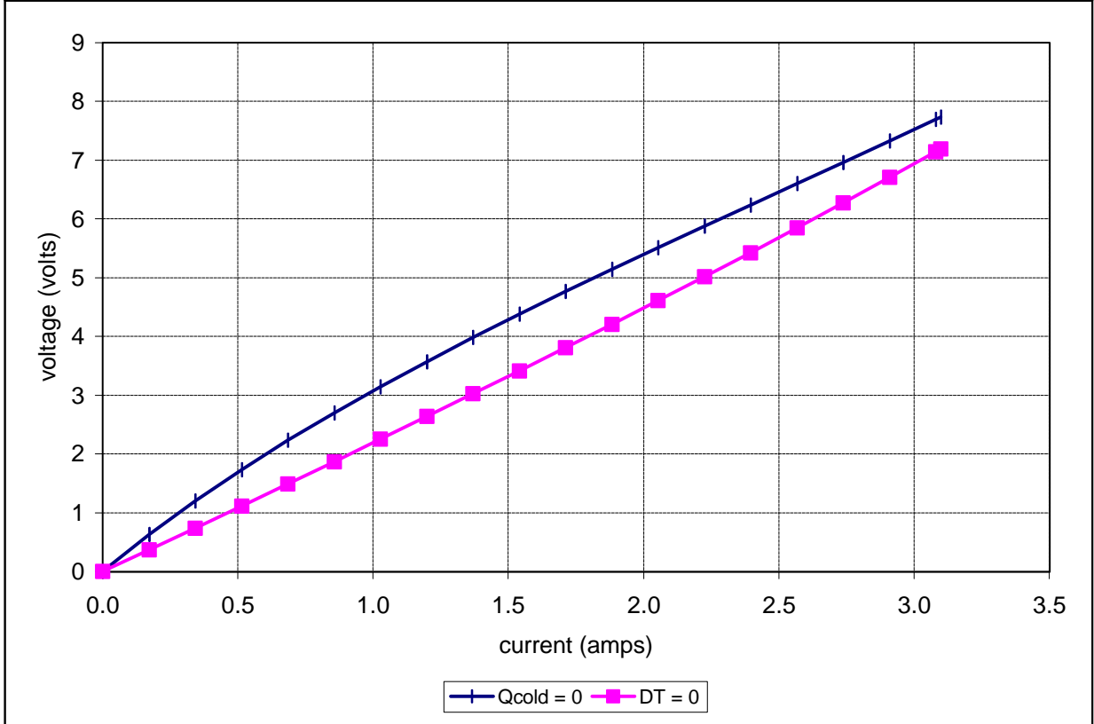
Unpotted TE-63-1.0-1.5 at a hot-side temperature of 25 °C
