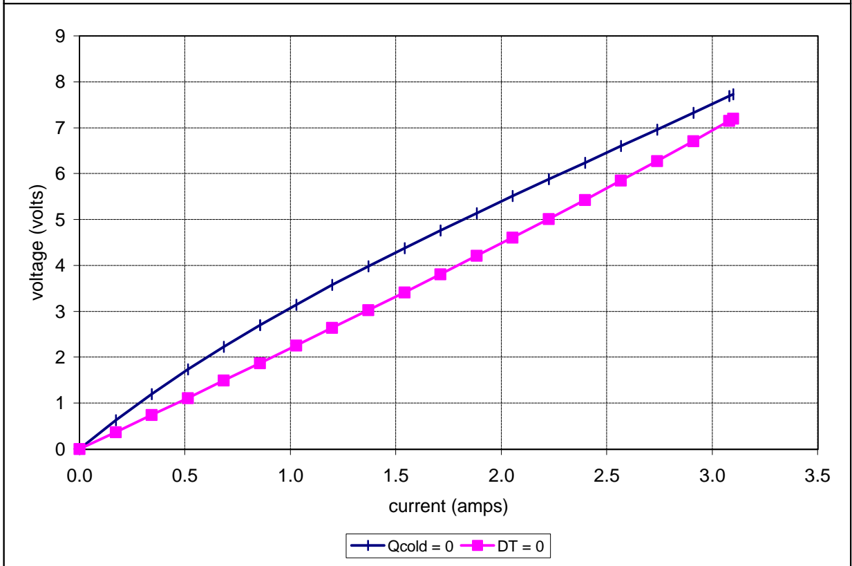
Potted TE-63-1.0-1.5 at a hot-side temperature of 25 °C
