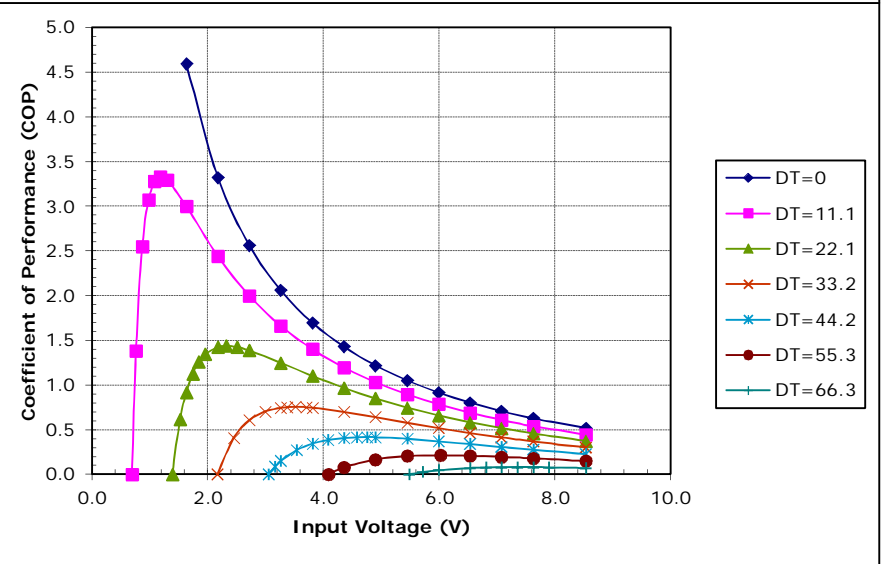
Unpotted TE-63-1.0-1.3 at a hot-side temperature of 50 °C
