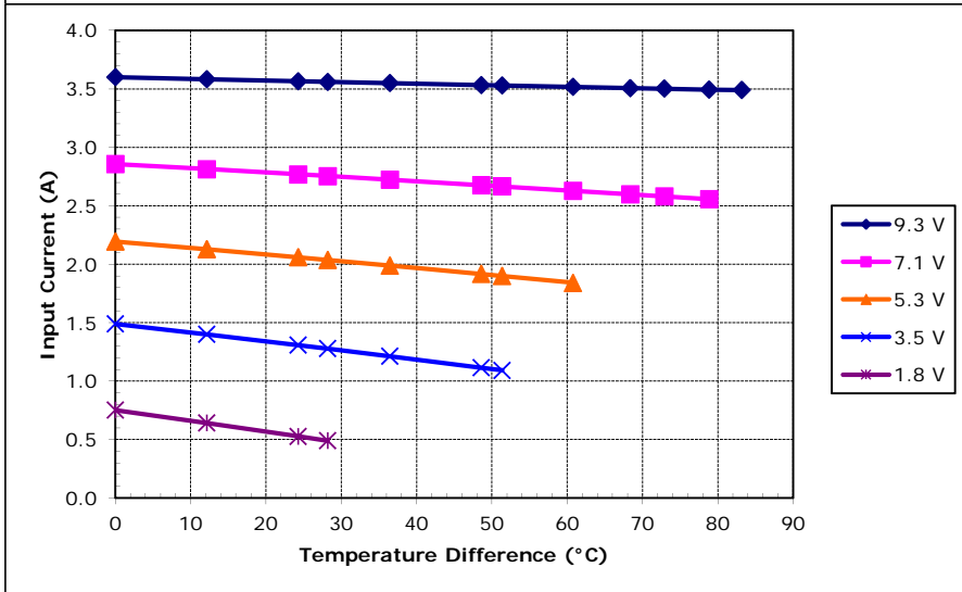
Unpotted TE-63-1.0-1.3 at a hot-side temperature of 70 °C
