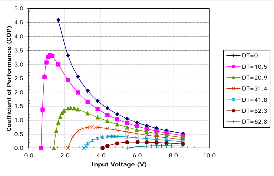
Potted TE-63-1.0-1.3 at a hot-side temperature of 50 °C
