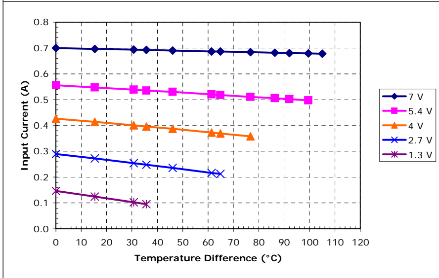
Potted TE-4-(59-31-11-4)-1.5 at a hot-side temperature of 30 °C
