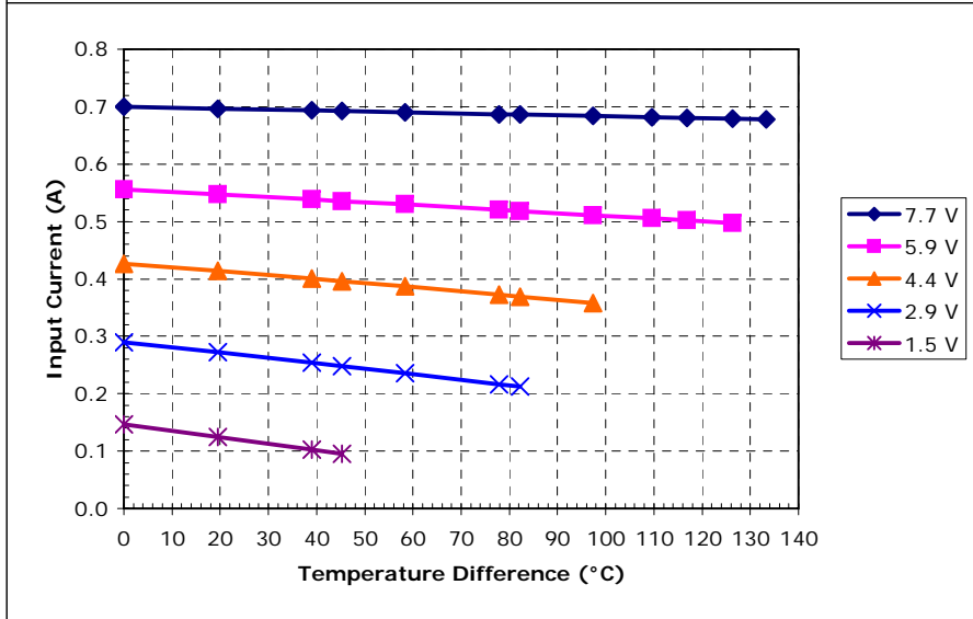
Unpotted TE-4-(59-31-11-4)-1.5 at a hot-side temperature of 50 °C
