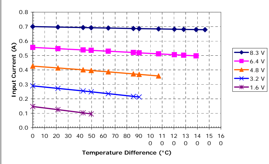
Unpotted TE-4-(59-31-11-4)-1.5 at a hot-side temperature of 70 °C
