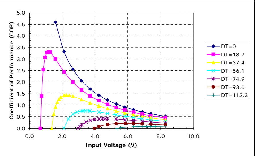
Potted TE-4-(59-31-11-4)-1.5 at a hot-side temperature of 70 °C
