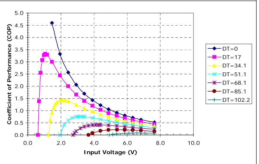
Potted TE-4-(59-31-11-4)-1.5 at a hot-side temperature of 50 °C
