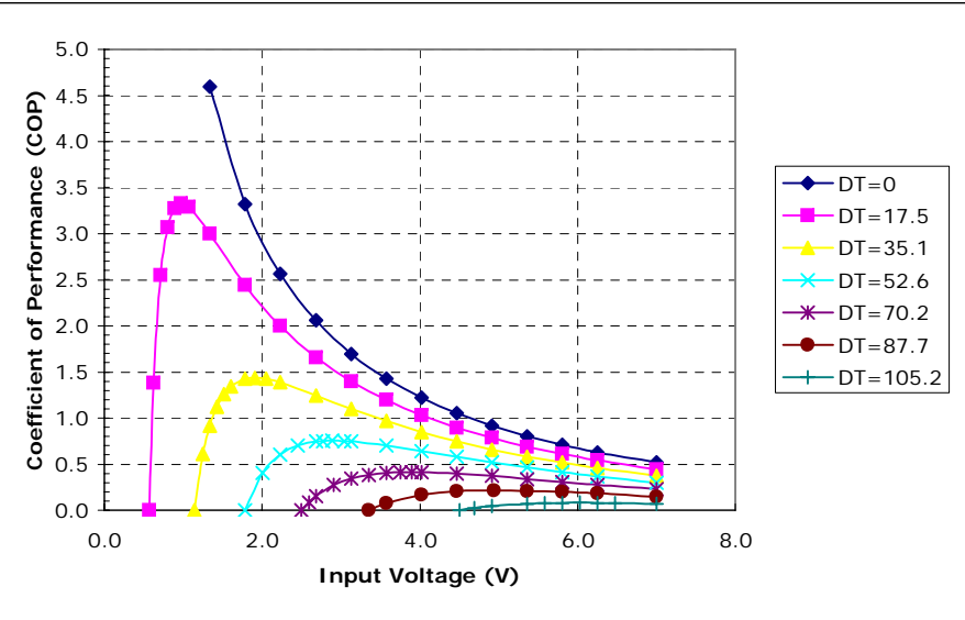
Unpotted TE-4-(59-31-11-4)-1.5 at a hot-side temperature of 30 °C
