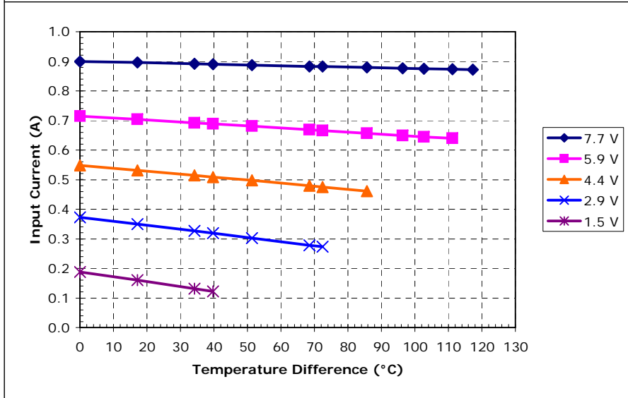
Potted TE-4-(59-31-11-4)-1.2 at a hot-side temperature of 50 °C
