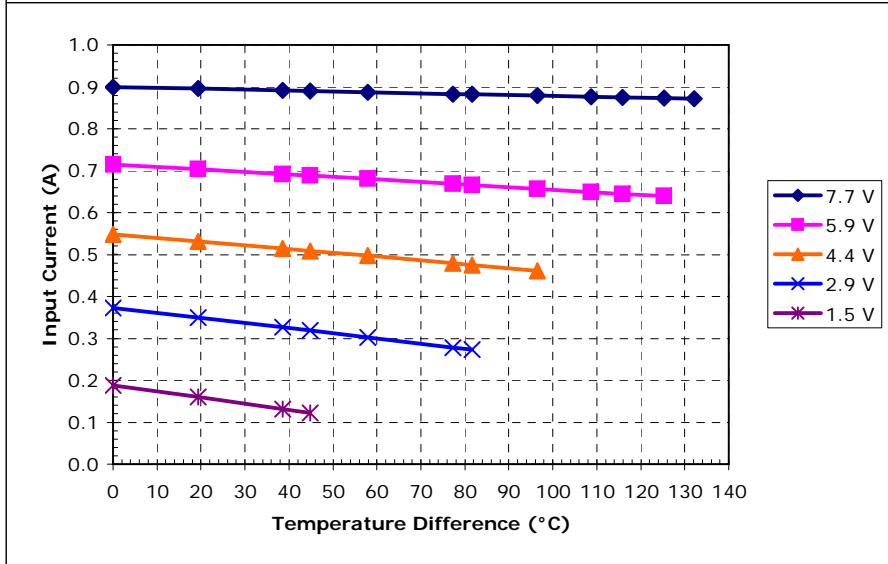
Unpotted TE-4-(59-31-11-4)-1.2 at a hot-side temperature of 50 °C
