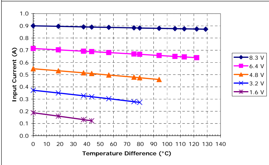
Potted TE-4-(59-31-11-4)-1.2 at a hot-side temperature of 70 °C
