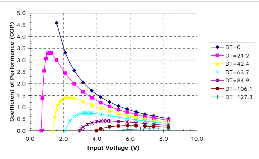
Unpotted TE-4-(59-31-11-4)-1.2 at a hot-side temperature of 70 °C
