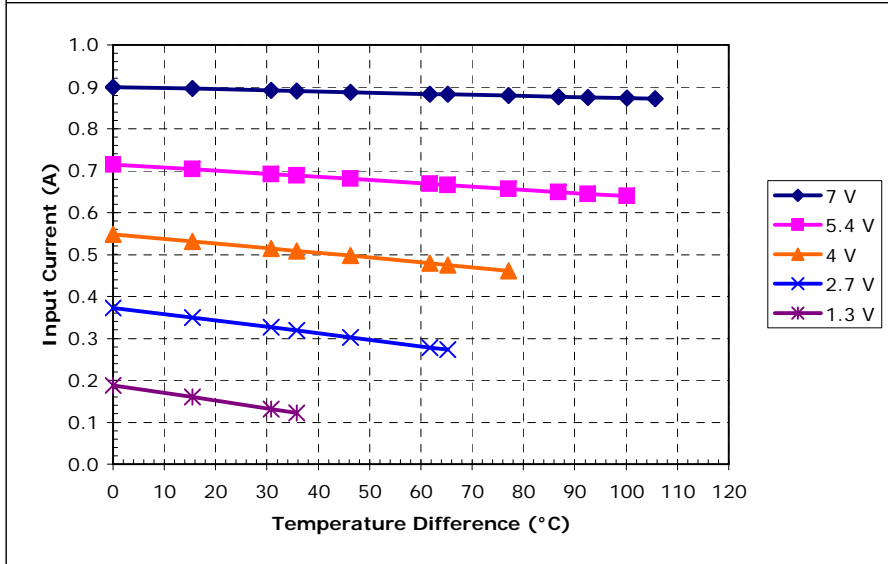
Potted TE-4-(59-31-11-4)-1.2 at a hot-side temperature of 30 °C
