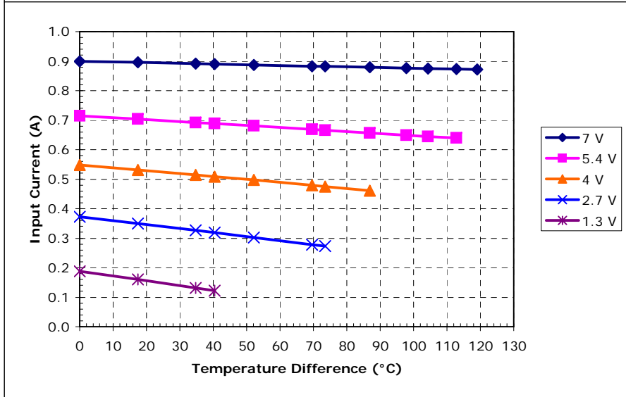
Unpotted TE-4-(59-31-11-4)-1.2 at a hot-side temperature of 30 °C
