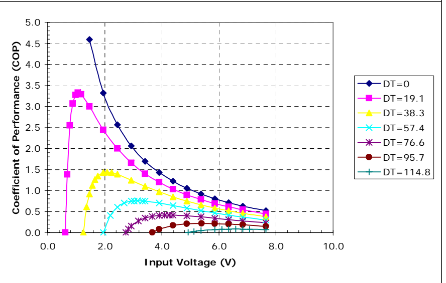
Unpotted TE-4-(59-31-11-4)-1.0 at a hot-side temperature of 50 °C
