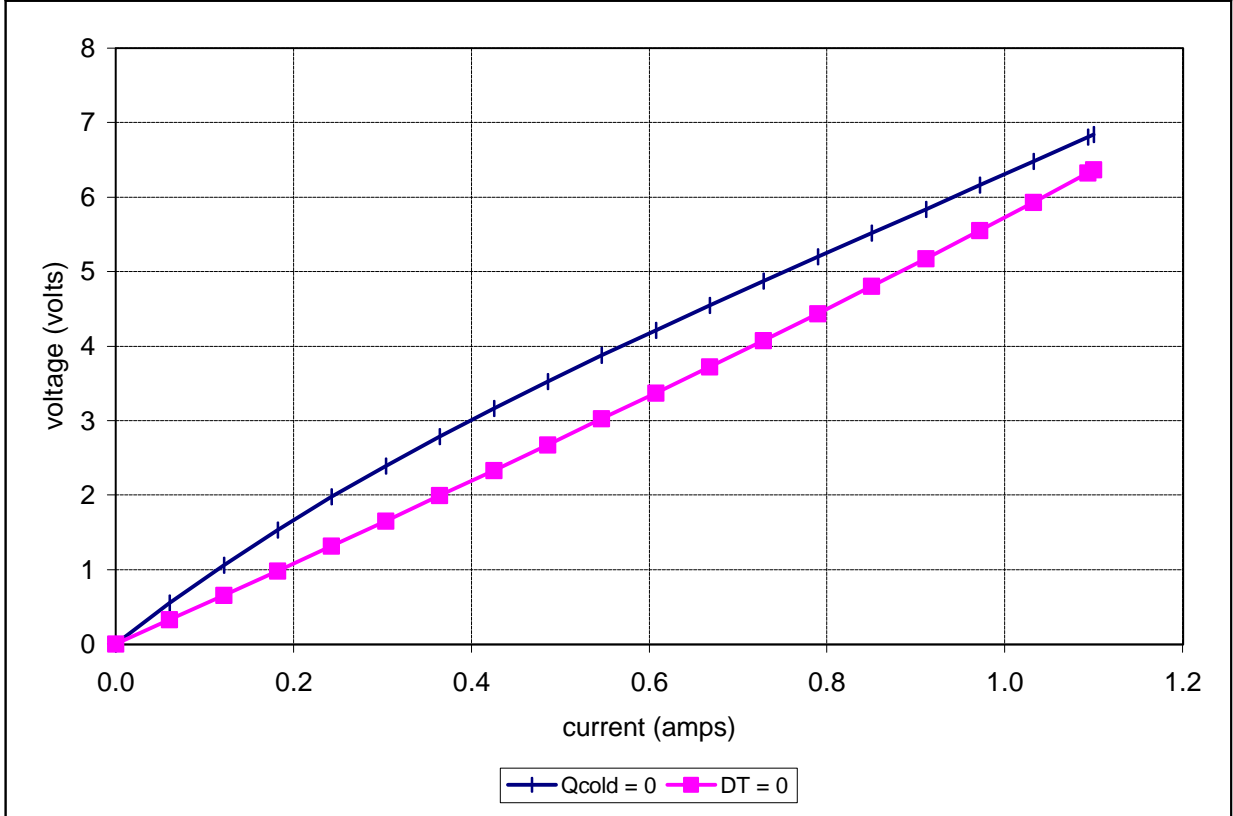
Unpotted TE-4-(59-31-11-4)-1.0 at a hot-side temperature of 25 °C
