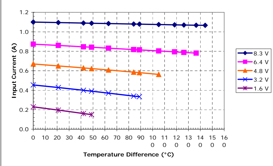
Unpotted TE-4-(59-31-11-4)-1.0 at a hot-side temperature of 70 °C
