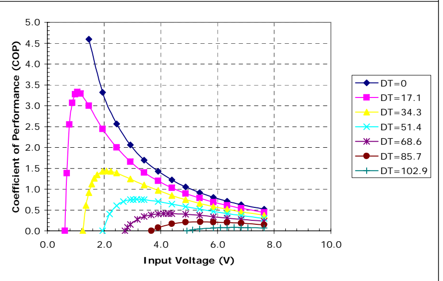
Potted TE-4-(59-31-11-4)-1.0 at a hot-side temperature of 50 °C
