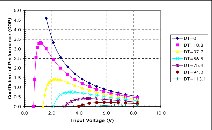
Potted TE-4-(59-31-11-4)-1.0 at a hot-side temperature of 70 °C
