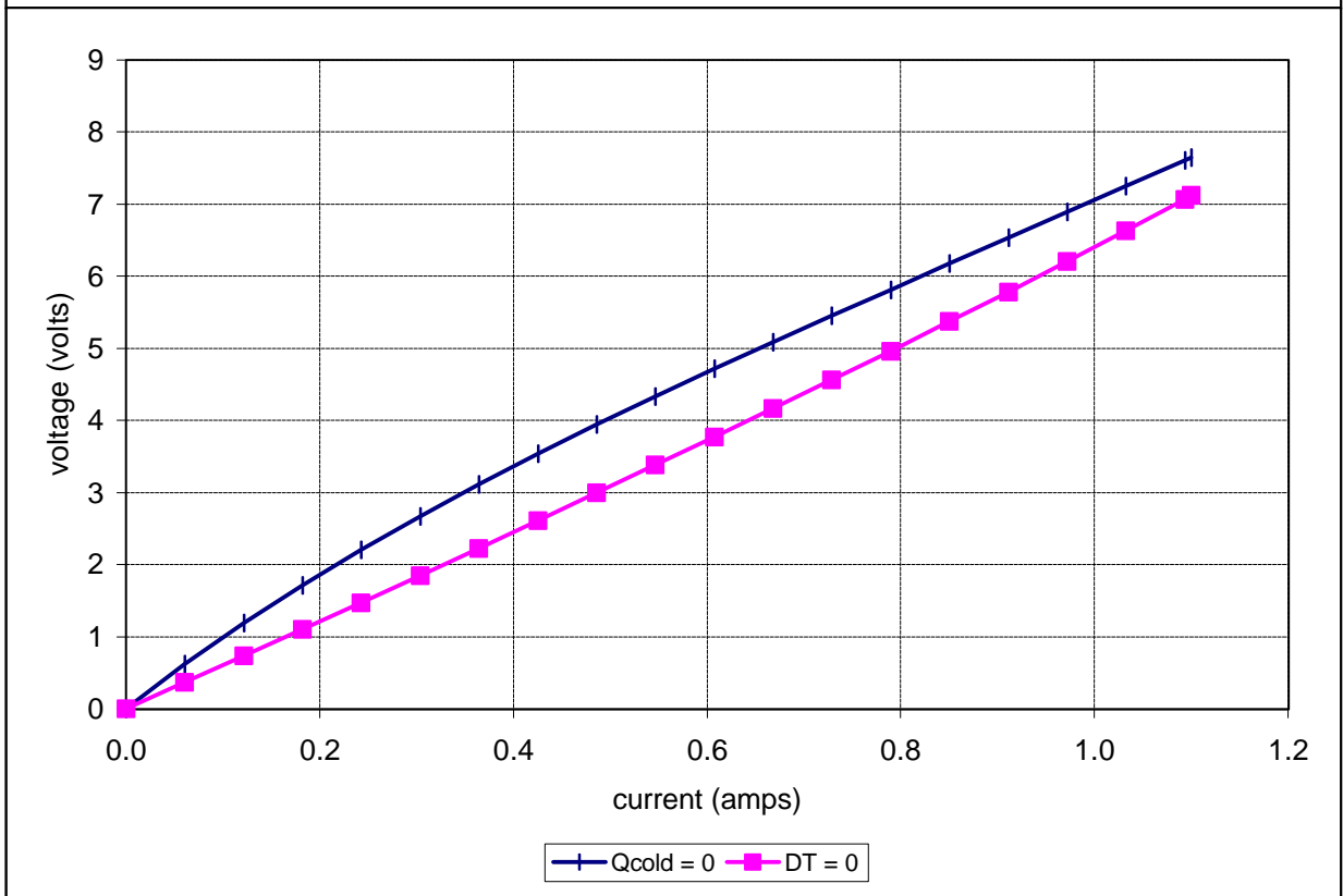
Unpotted TE-4-(59-31-11-4)-1.0 at a hot-side temperature of 50 °C
