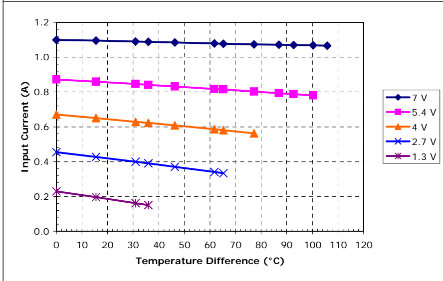
Potted TE-4-(59-31-11-4)-1.0 at a hot-side temperature of 30 °C
