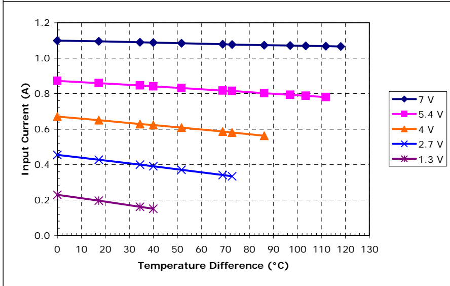
Unpotted TE-4-(59-31-11-4)-1.0 at a hot-side temperature of 30 °C
