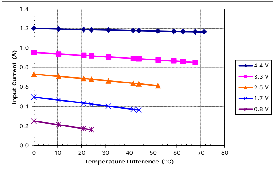
Unpotted TE-35-0.6-1.5 at a hot-side temperature of 30 °C
