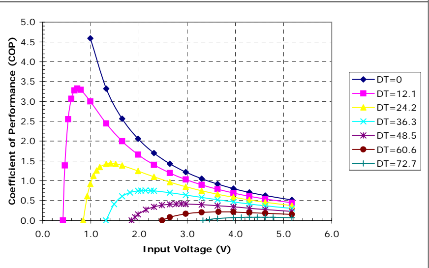
Potted TE-35-0.6-1.5 at a hot-side temperature of 70 °C
