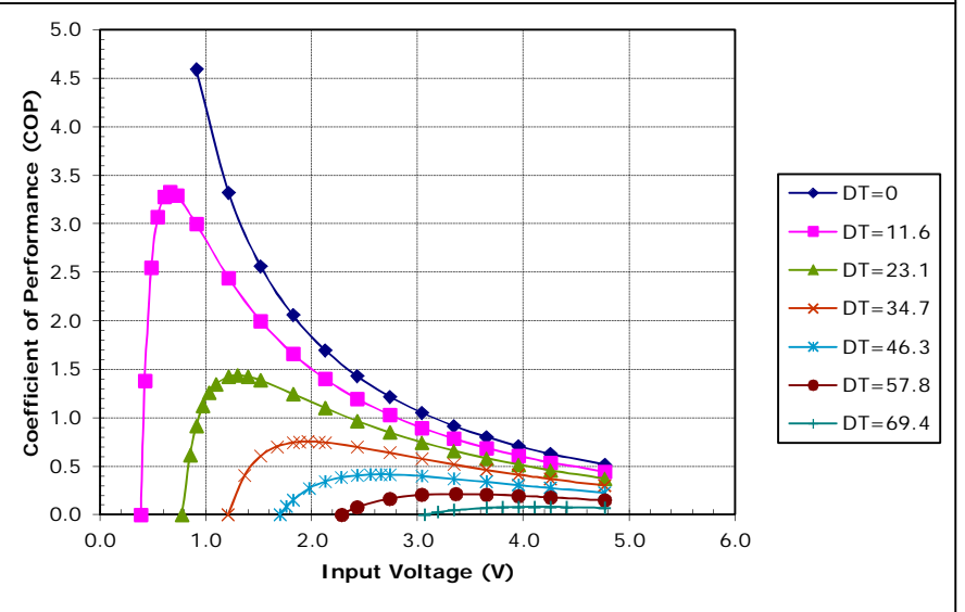
Unpotted TE-35-0.6-1.5 at a hot-side temperature of 50 °C
