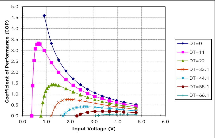
Potted TE-35-0.6-1.5 at a hot-side temperature of 50 °C
