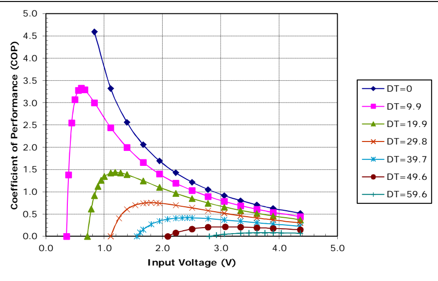
Potted TE-35-0.6-1.5 at a hot-side temperature of 30 °C
