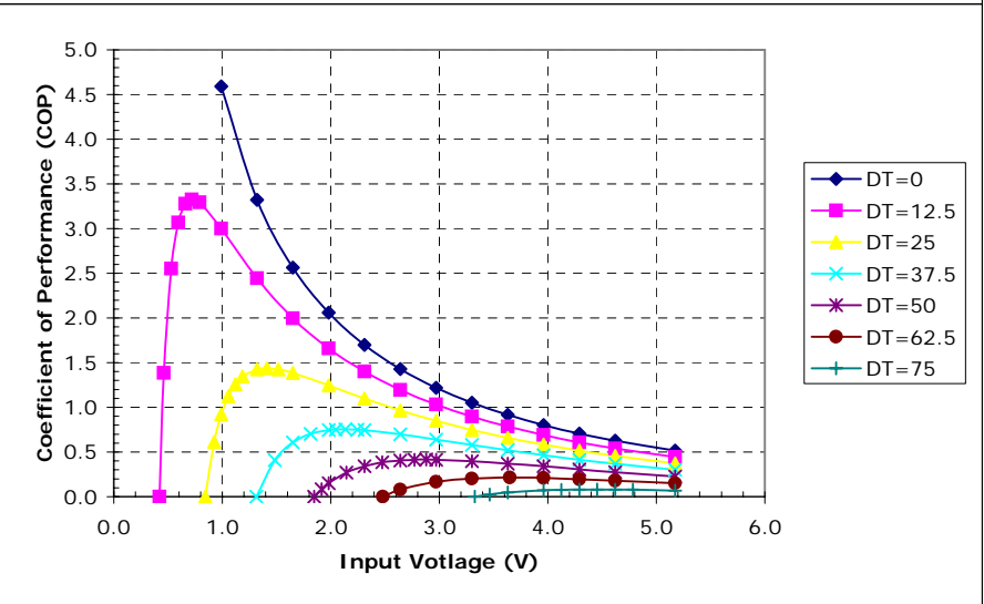
Unpotted TE-35-0.6-1.2 at a hot-side temperature of 70 °C
