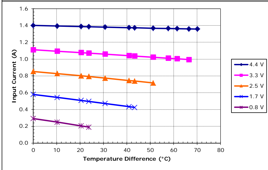
Unpotted TE-35-0.6-1.2 at a hot-side temperature of 30 °C
