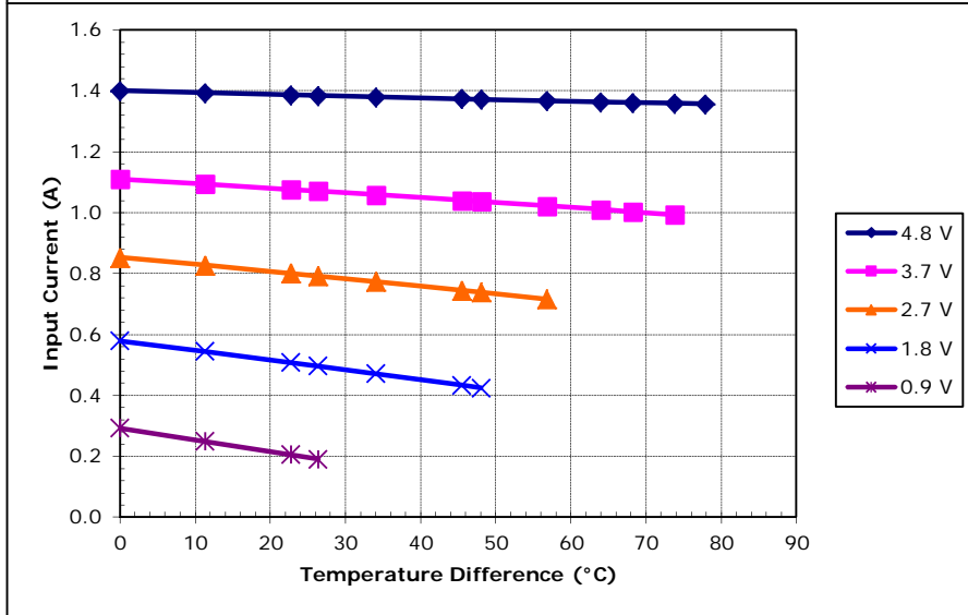
Unpotted TE-35-0.6-1.2 at a hot-side temperature of 50 °C
