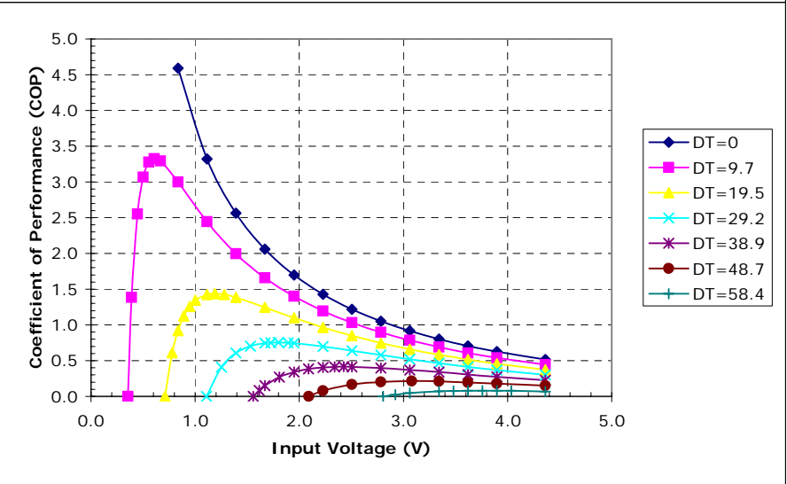
Potted TE-35-0.6-1.2 at a hot-side temperature of 30 °C
