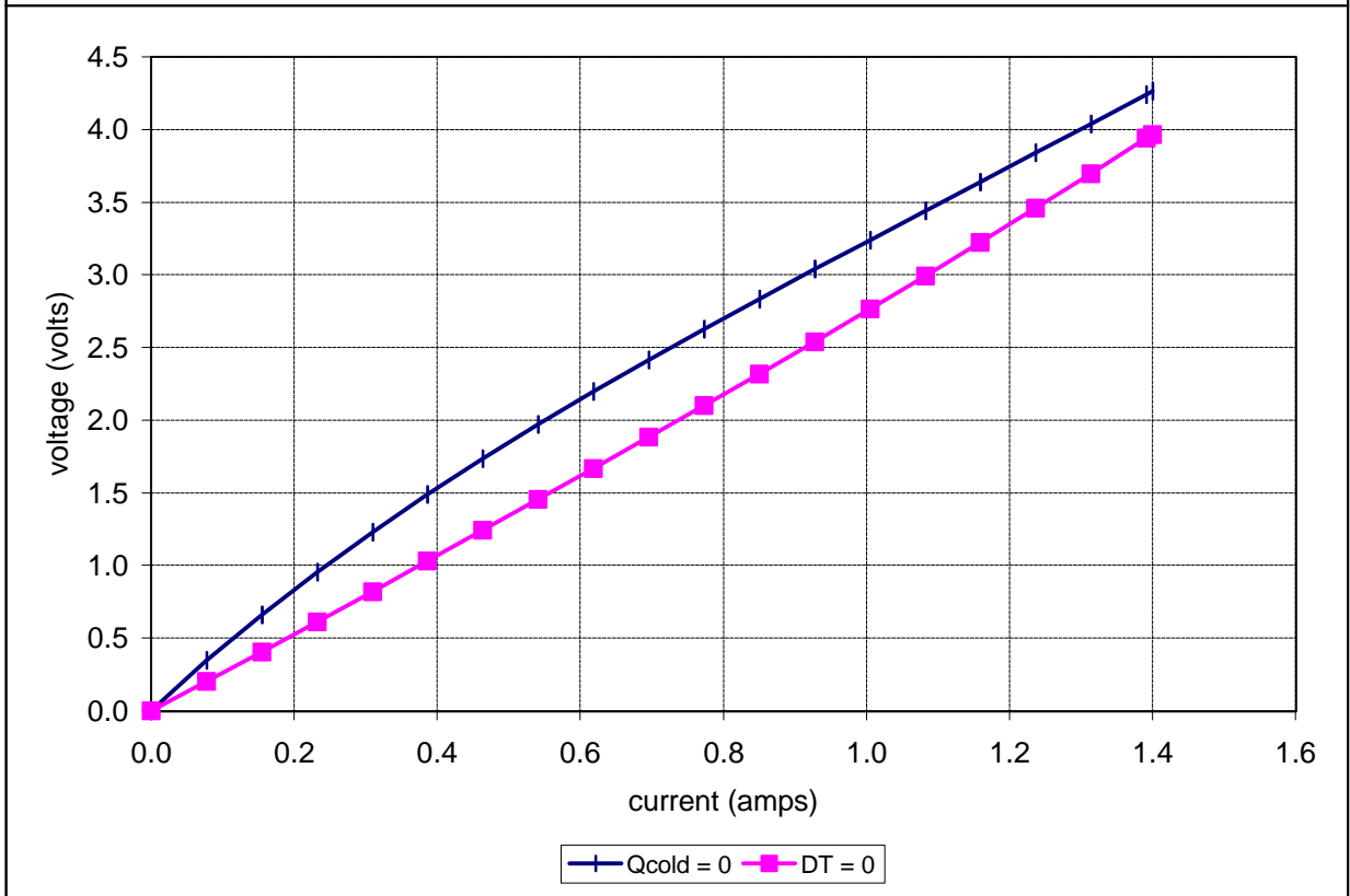
Potted TE-35-0.6-1.2 at a hot-side temperature of 25 °C
