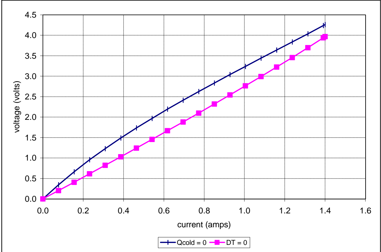
Unpotted TE-35-0.6-1.2 at a hot-side temperature of 25 °C
