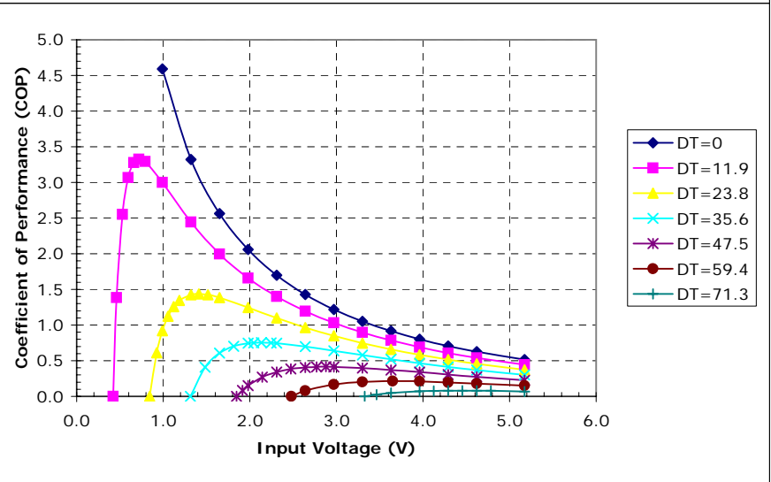
Potted TE-35-0.6-1.2 at a hot-side temperature of 70 °C
