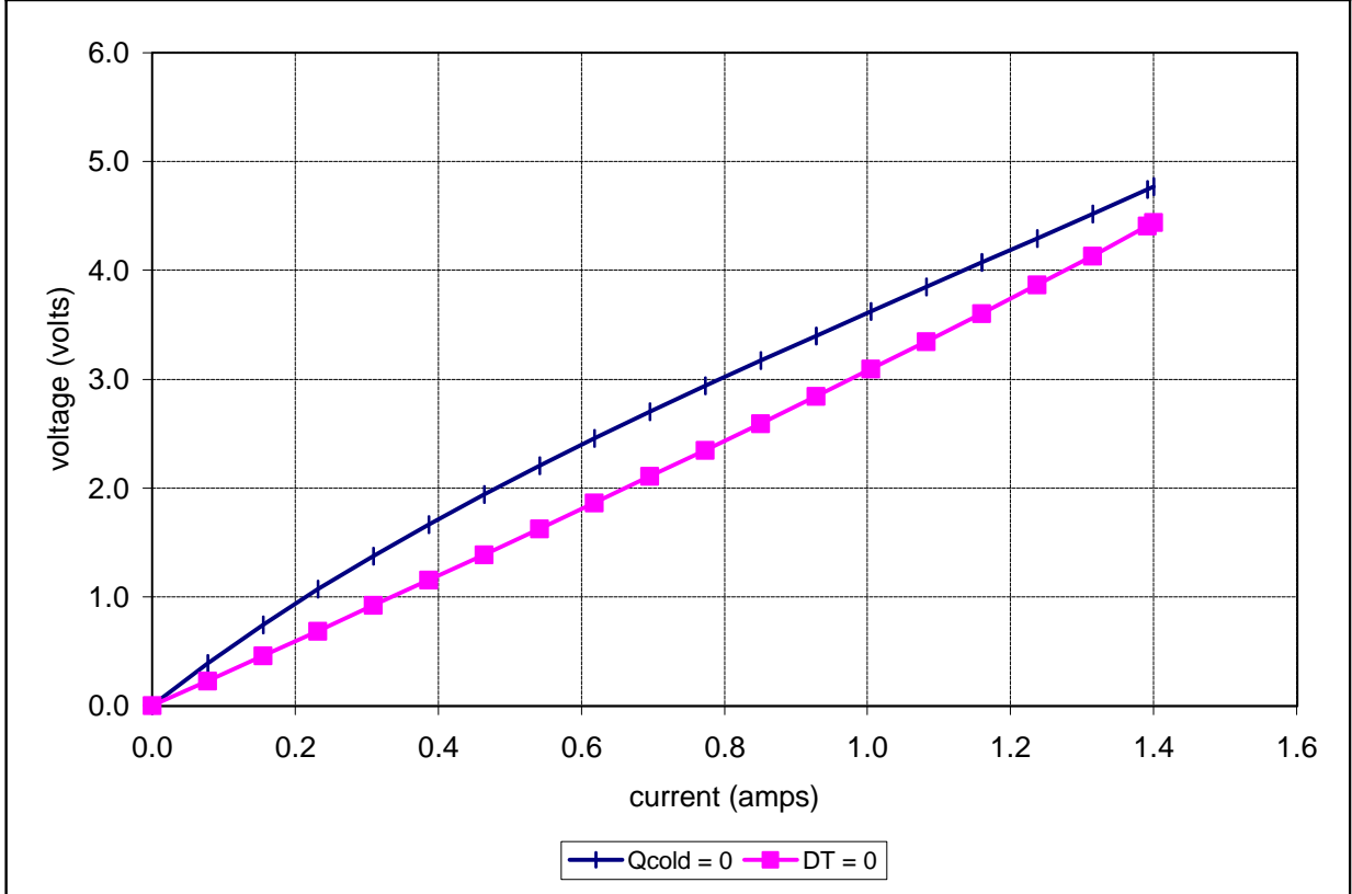
Unpotted TE-35-0.6-1.2 at a hot-side temperature of 50 °C
