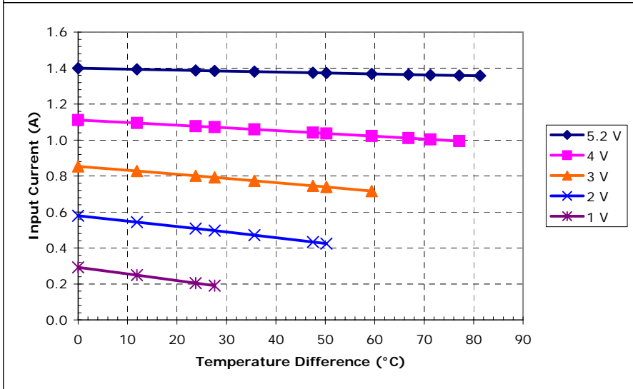
Potted TE-35-0.6-1.2 at a hot-side temperature of 70 °C
