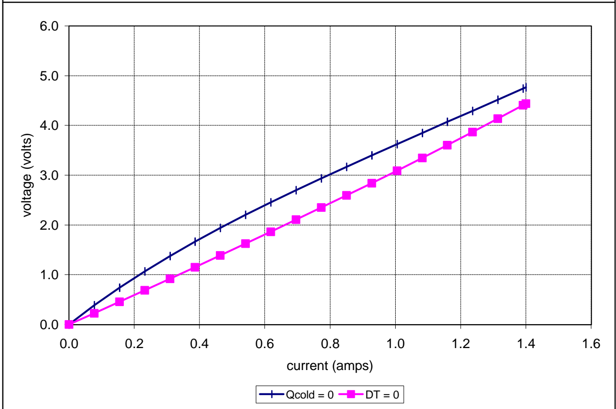
Potted TE-35-0.6-1.2 at a hot-side temperature of 50 °C
