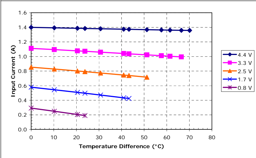
Unpotted TE-35-0.6-1.2 at a hot-side temperature of 30 °C
