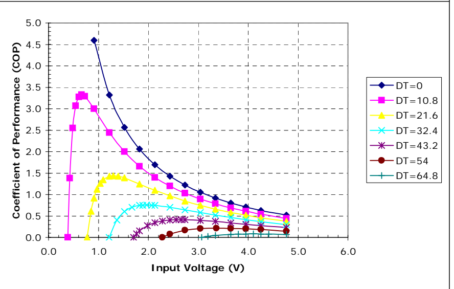
Potted TE-35-0.6-1.2 at a hot-side temperature of 50 °C
