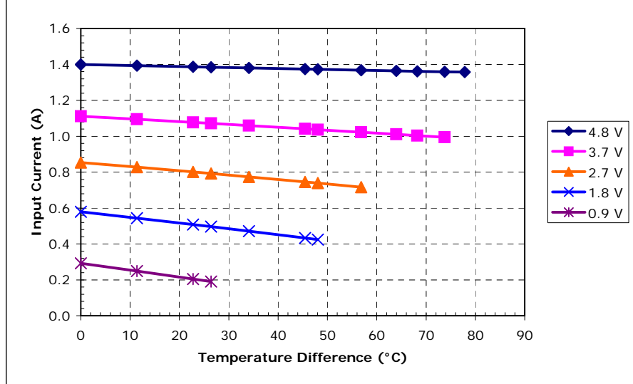
Unpotted TE-35-0.6-1.2 at a hot-side temperature of 50 °C
