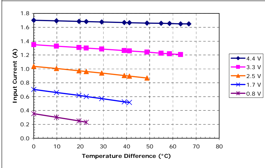
Potted TE-35-0.6-1.0 at a hot-side temperature of 30 °C
