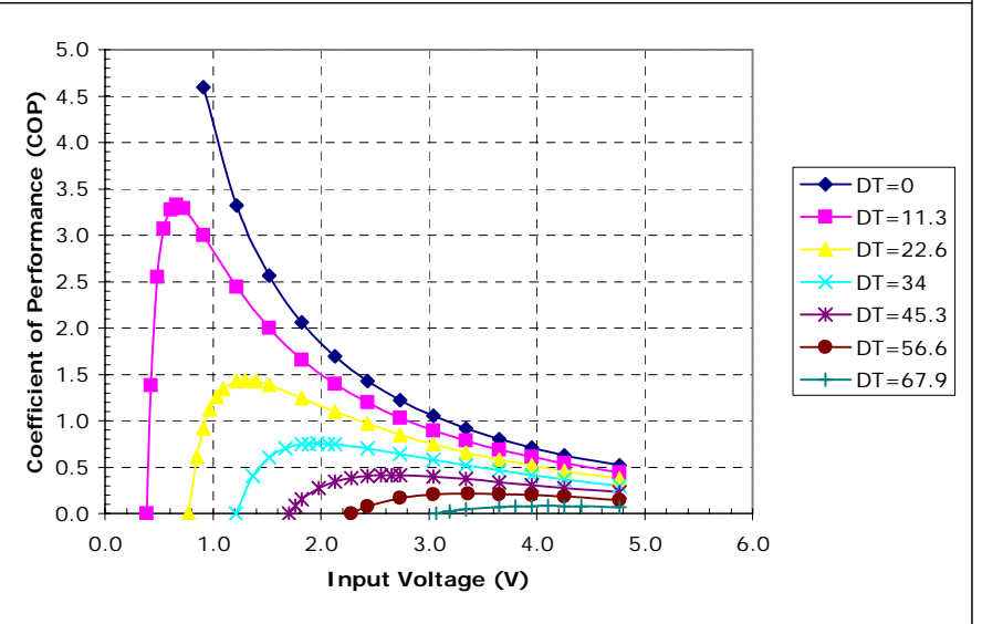
Unpotted TE-35-0.6-1.0 at a hot-side temperature of 50 °C
