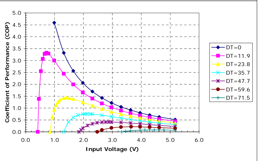
Potted TE-35-0.6-1.0 at a hot-side temperature of 70 °C
