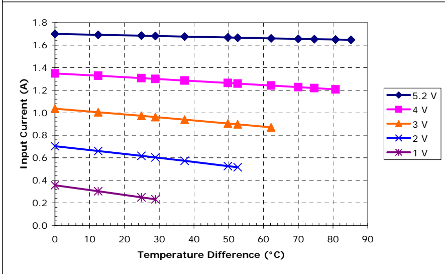
Unpotted TE-35-0.6-1.0 at a hot-side temperature of 70 °C
