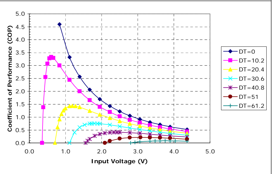
Unpotted TE-35-0.6-1.0 at a hot-side temperature of 30 °C
