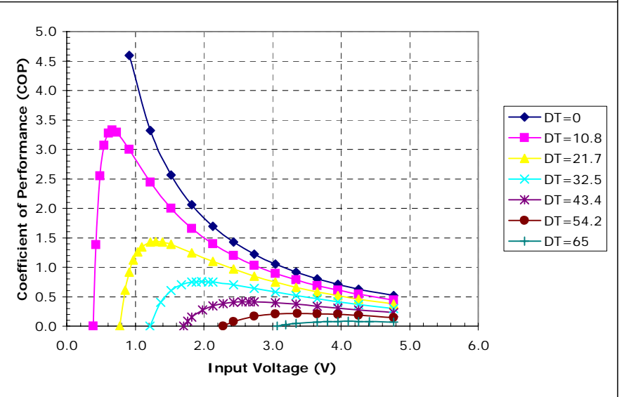
Potted TE-35-0.6-1.0 at a hot-side temperature of 50 °C
