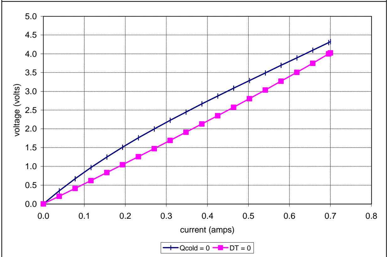
Potted TE-32-0.45-1.3 at a hot-side temperature of 50 °C
