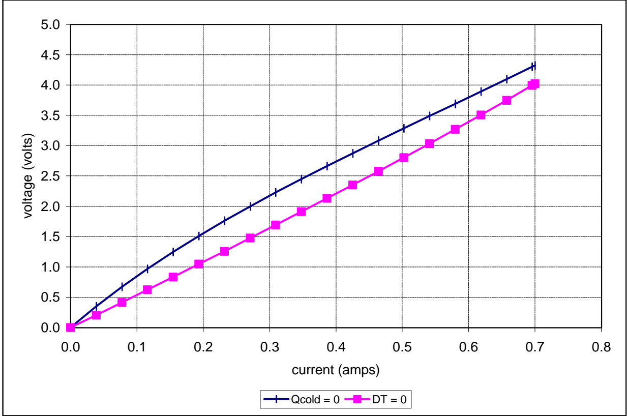
Unpotted TE-32-0.45-1.3 at a hot-side temperature of 50 °C
