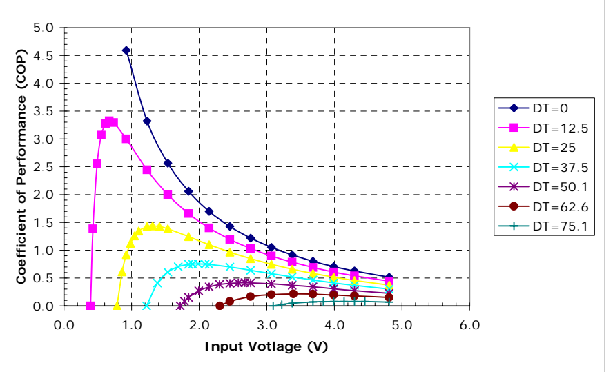
Unpotted TE-32-0.45-1.3 at a hot-side temperature of 70 °C
