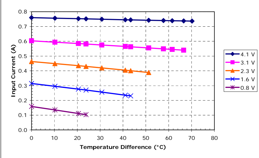
Unpotted TE-32-0.45-1.3 at a hot-side temperature of 30 °C
