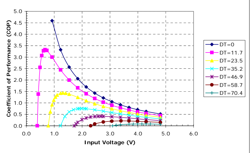
Potted TE-32-0.45-1.3 at a hot-side temperature of 70 °C
