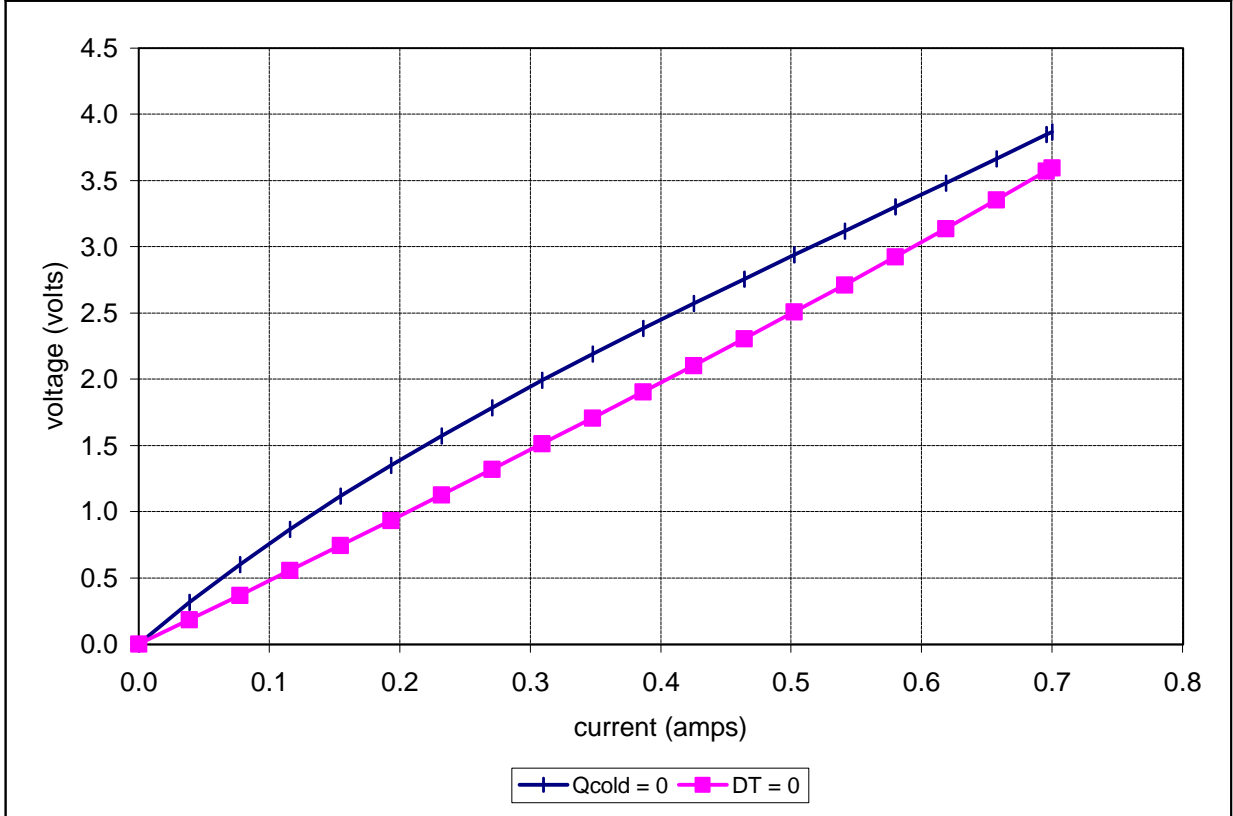
Unpotted TE-32-0.45-1.3 at a hot-side temperature of 25 °C
