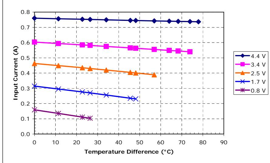
Unpotted TE-32-0.45-1.3 at a hot-side temperature of 50 °C
