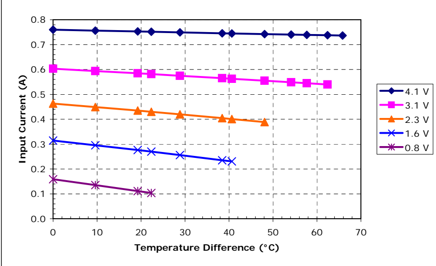
Potted TE-32-0.45-1.3 at a hot-side temperature of 30 °C
