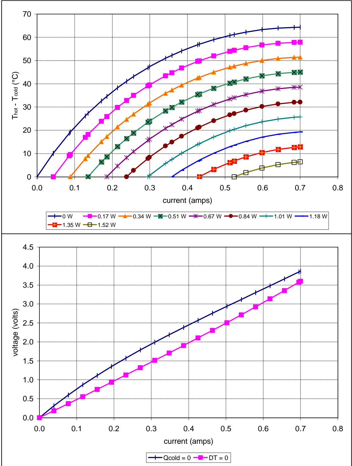
Potted TE-32-0.45-1.3 at a hot-side temperature of 25 °C
