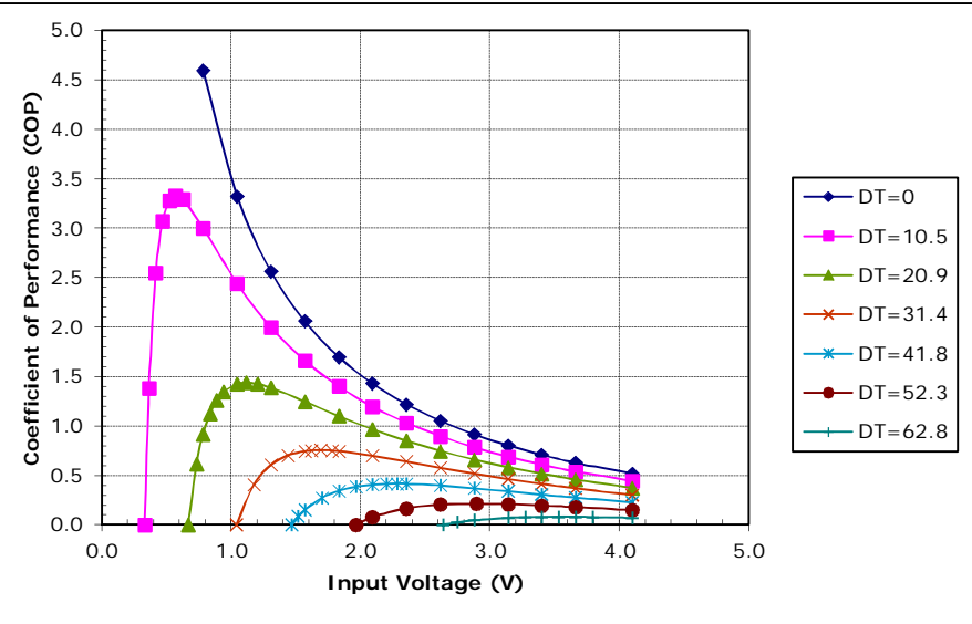
Potted TE-31-2.0-2.5 at a hot-side temperature of 50 °C
