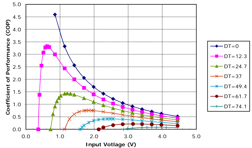
Unpotted TE-31-2.0-2.5 at a hot-side temperature of 70 °C
