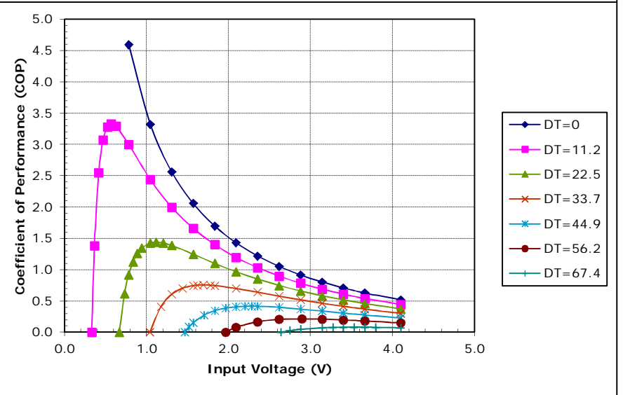
Unpotted TE-31-2.0-2.5 at a hot-side temperature of 50 °C
