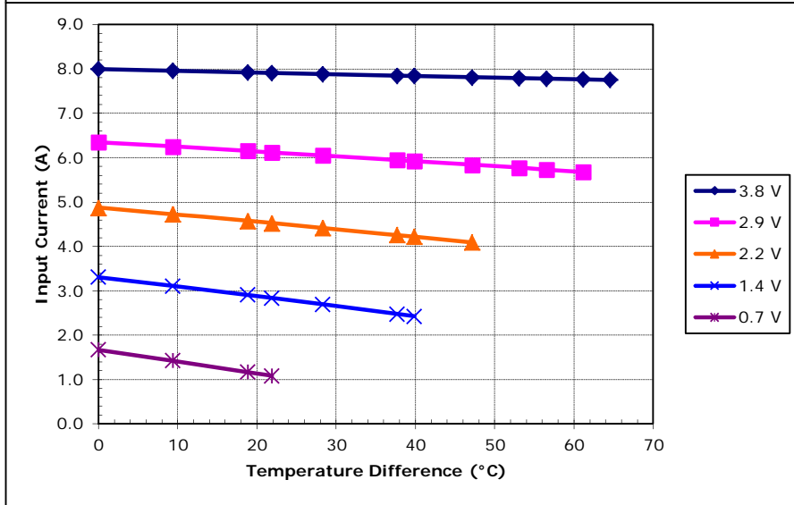
Potted TE-31-2.0-2.5 at a hot-side temperature of 30 °C
