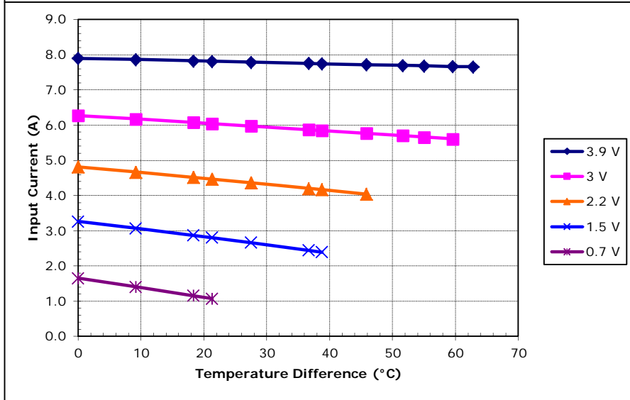
Potted TE-31-1.4-1.15 at a hot-side temperature of 30 °C
