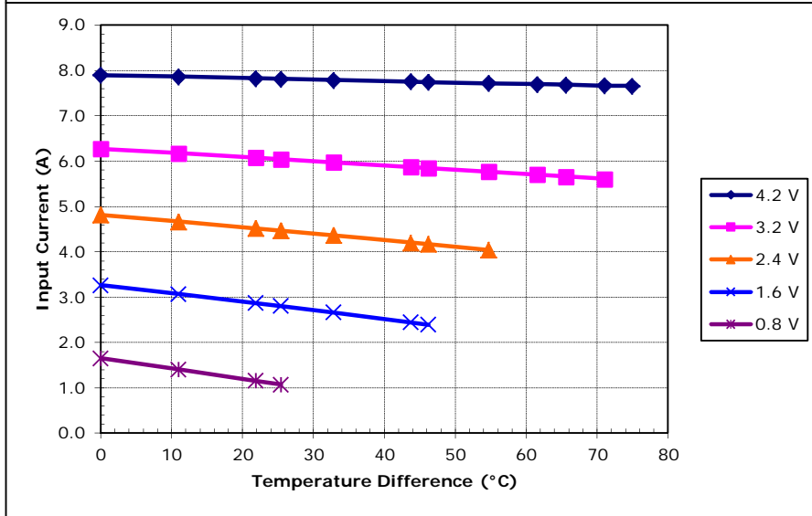
Unpotted TE-31-1.4-1.15 at a hot-side temperature of 50 °C
