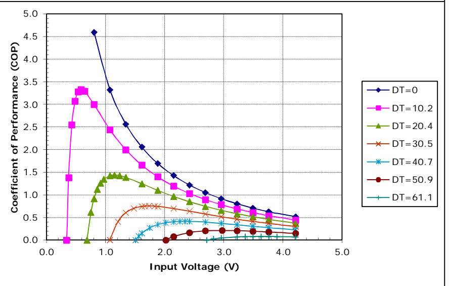
Potted TE-31-1.4-1.15 at a hot-side temperature of 50 °C
