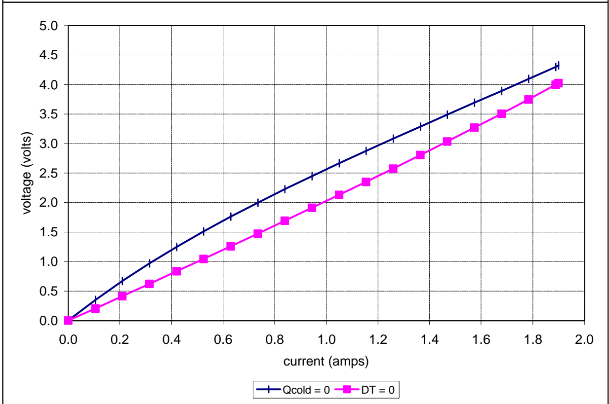
Potted TE-31-1.0-2.5 at a hot-side temperature of 50 °C
