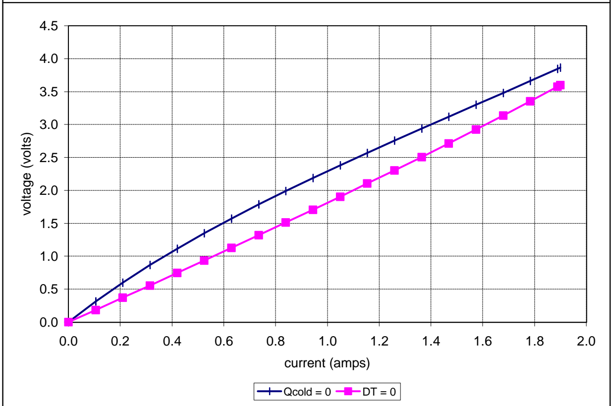
Potted TE-31-1.0-2.5 at a hot-side temperature of 25 °C
