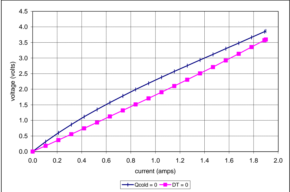
Unpotted TE-31-1.0-2.5 at a hot-side temperature of 25 °C
