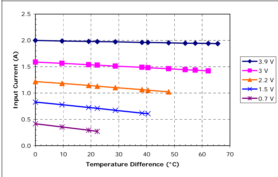
Potted TE-31-1.0-2.5 at a hot-side temperature of 30 °C
