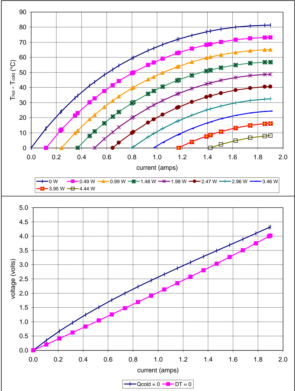
Unpotted TE-31-1.0-2.5 at a hot-side temperature of 50 °C
