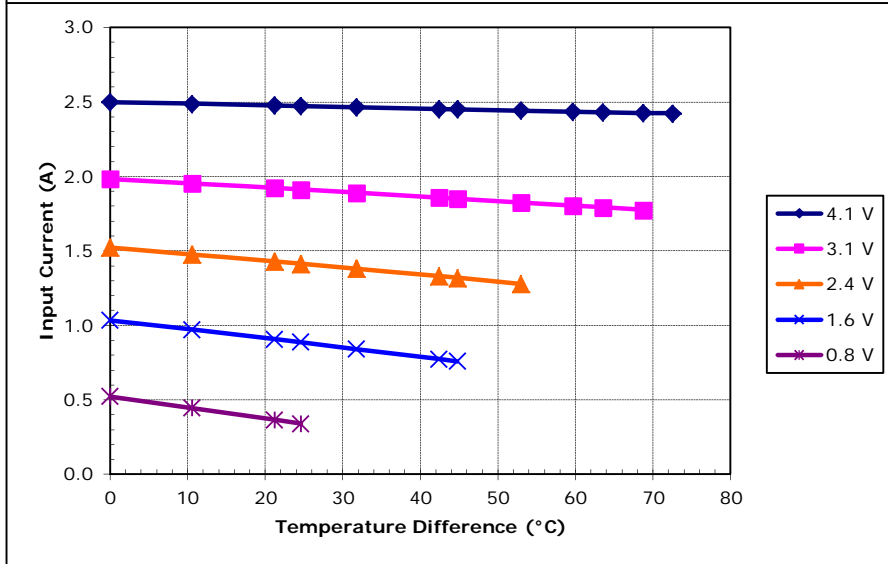
Potted TE-31-1.0-2.0 at a hot-side temperature of 50 °C
