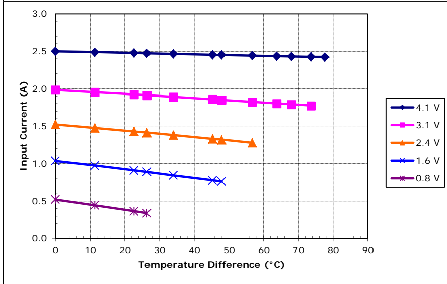
Unpotted TE-31-1.0-2.0 at a hot-side temperature of 50 °C
