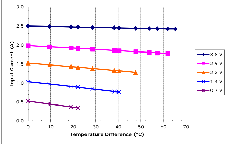
Potted TE-31-1.0-2.0 at a hot-side temperature of 30 °C
