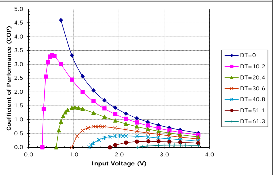
Unpotted TE-31-1.0-2.0 at a hot-side temperature of 30 °C
