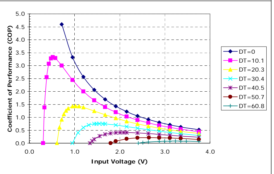
Unpotted TE-31-1.0-1.5 at a hot-side temperature of 30 °C
