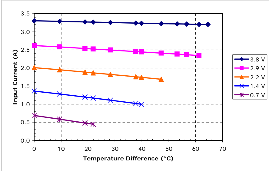
Potted TE-31-1.0-1.5 at a hot-side temperature of 30 °C
