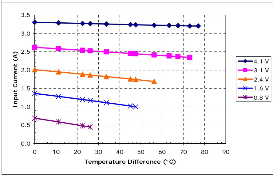
Unpotted TE-31-1.0-1.5 at a hot-side temperature of 50 °C
