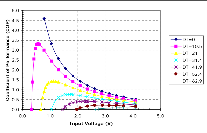
Potted TE-31-1.0-1.5 at a hot-side temperature of 50 °C
