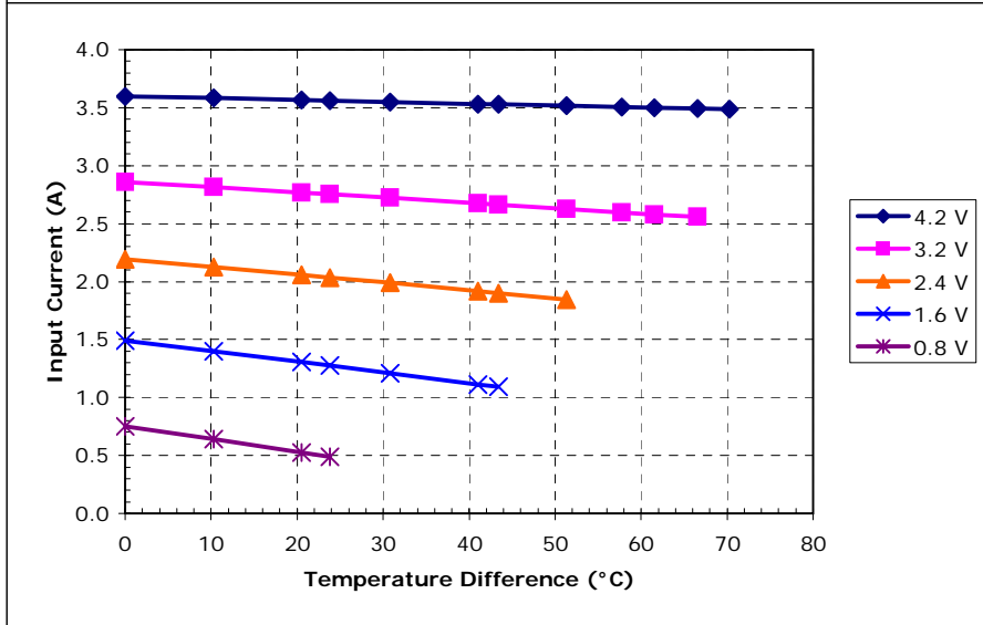
Potted TE-31-1.0-1.3 at a hot-side temperature of 50 °C
