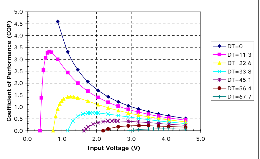
Potted TE-31-1.0-1.3 at a hot-side temperature of 70 °C
