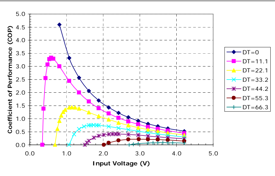
Unpotted TE-31-1.0-1.3 at a hot-side temperature of 50 °C
