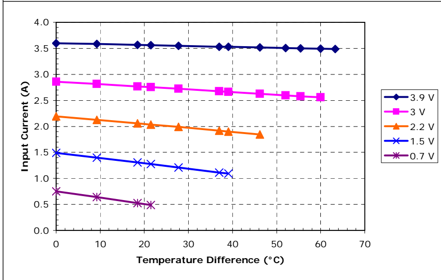
Potted TE-31-1.0-1.3 at a hot-side temperature of 30 °C
