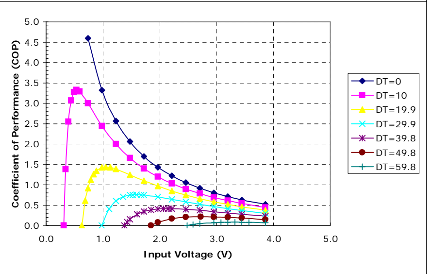
Unpotted TE-31-1.0-1.3 at a hot-side temperature of 30 °C
