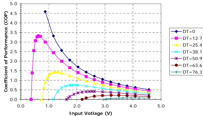
Unpotted TE-31-0.6-1.5 at a hot-side temperature of 70 °C
