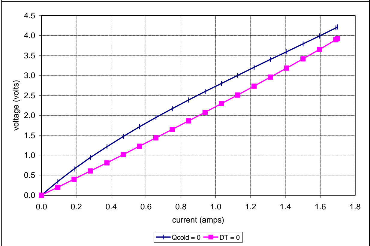
Potted TE-31-0.6-1.0 at a hot-side temperature of 50 °C
