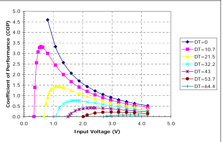
Potted TE-31-0.6-1.0 at a hot-side temperature of 50 °C
