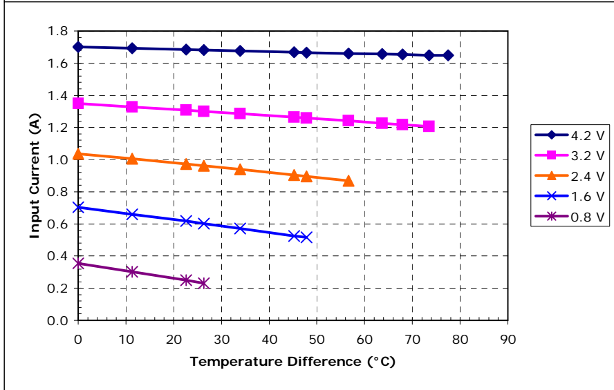
Unpotted TE-31-0.6-1.0 at a hot-side temperature of 50 °C
