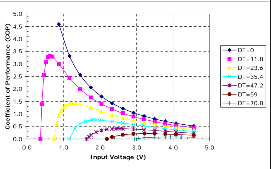
Potted TE-31-0.6-1.0 at a hot-side temperature of 70 °C
