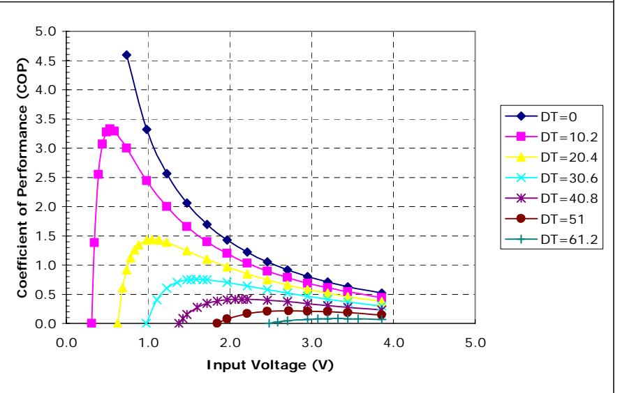
Unpotted TE-31-0.6-1.0 at a hot-side temperature of 30 °C
