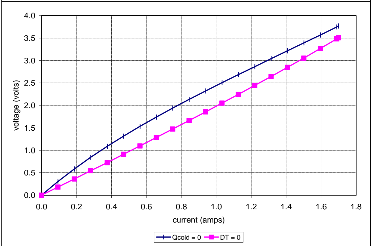
Potted TE-31-0.6-1.0 at a hot-side temperature of 25 °C
