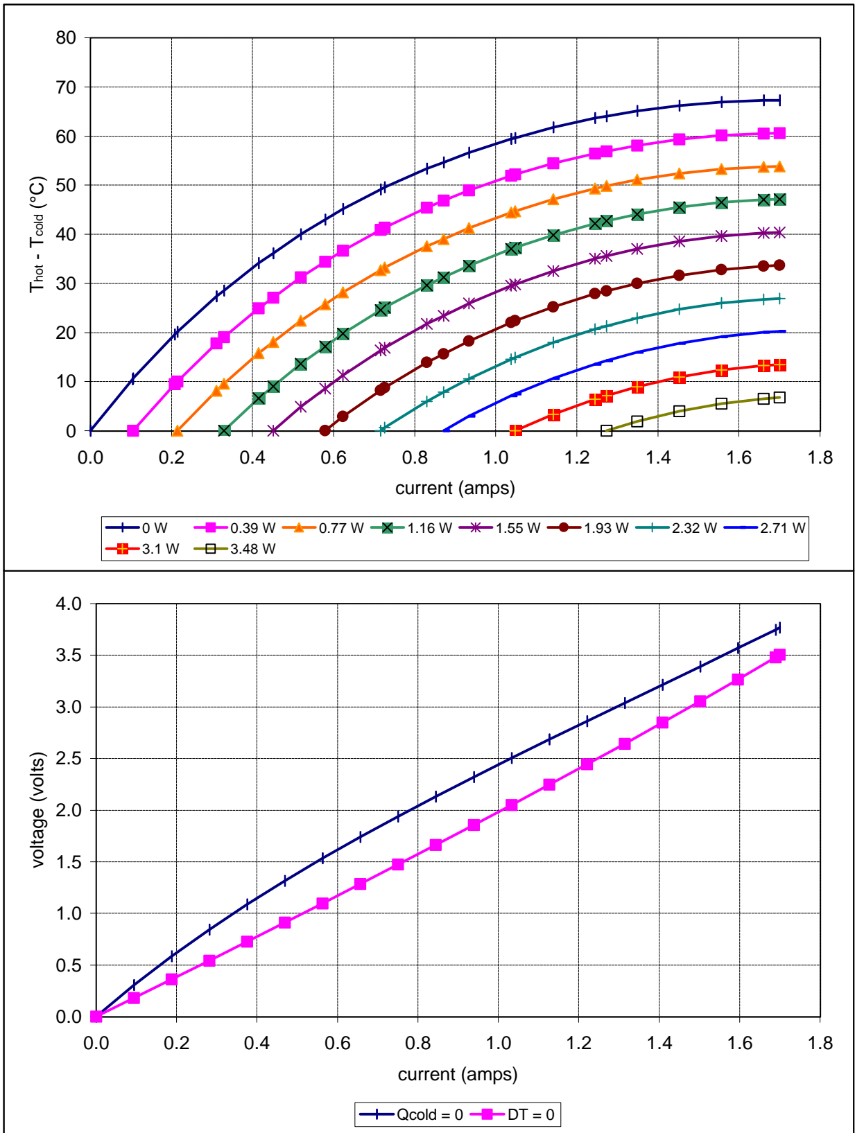
Unpotted TE-31-0.6-1.0 at a hot-side temperature of 25 °C
