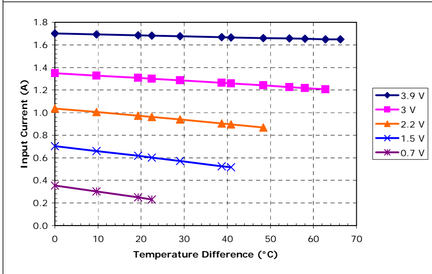
Potted TE-31-0.6-1.0 at a hot-side temperature of 30 °C
