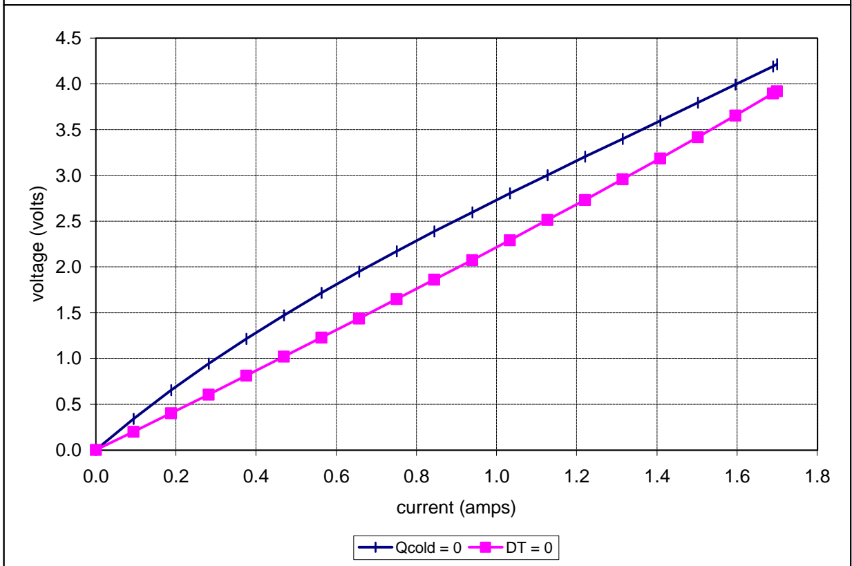
Unpotted TE-31-0.6-1.0 at a hot-side temperature of 50 °C
