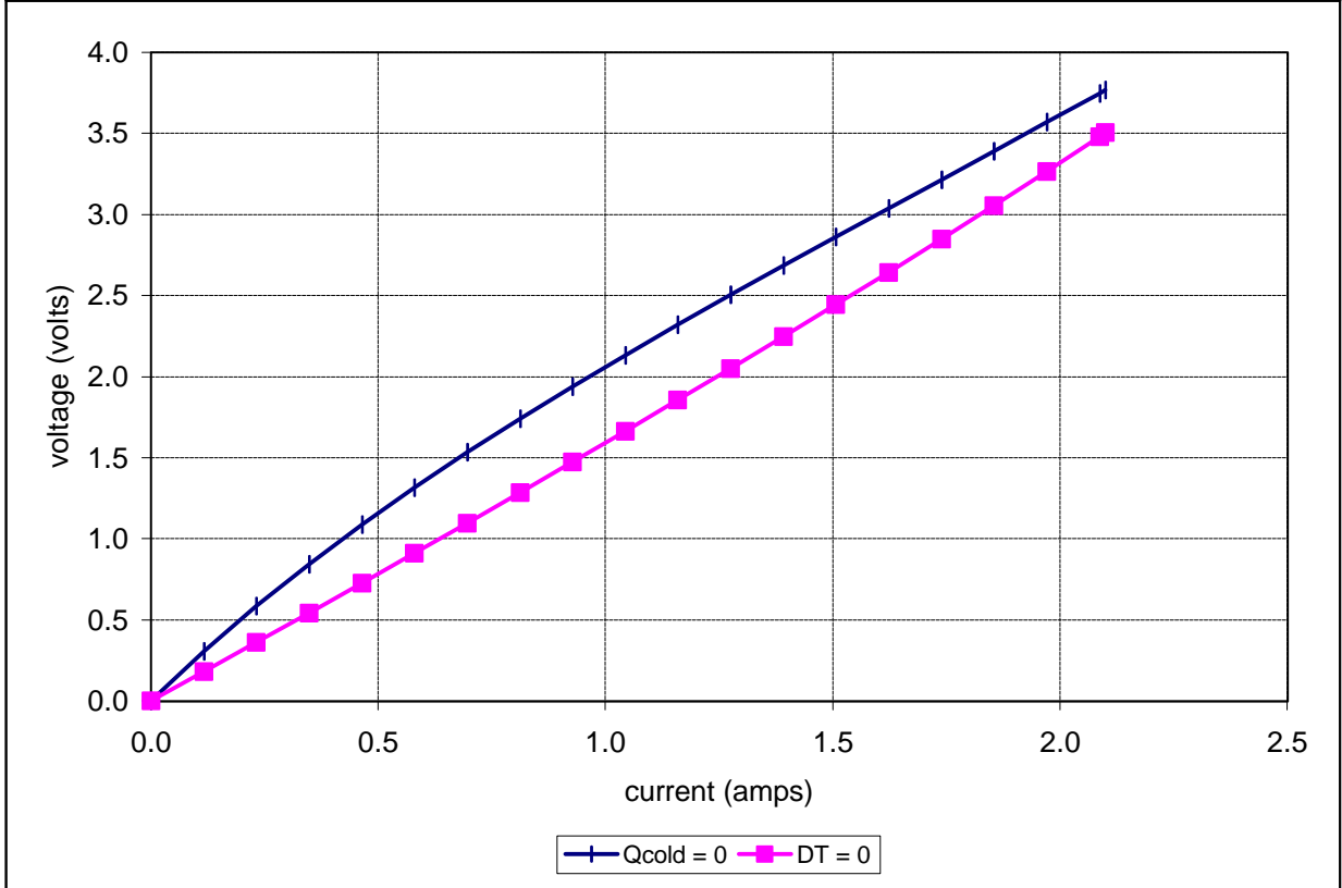
Unpotted TE-31-0.6-0.8 at a hot-side temperature of 25 °C
