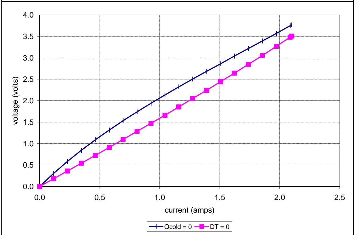
Potted TE-31-0.6-0.8 at a hot-side temperature of 25 °C
