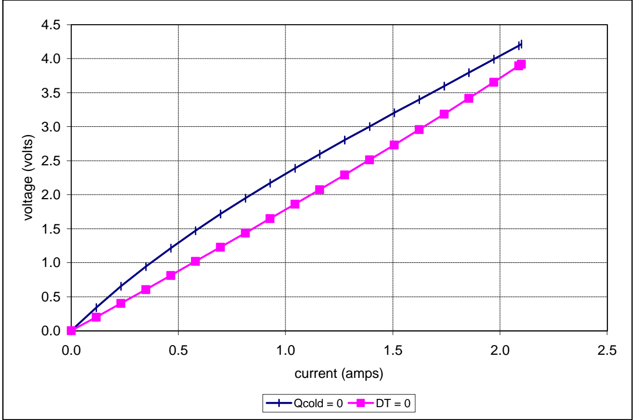
Unpotted TE-31-0.6-0.8 at a hot-side temperature of 50 °C
