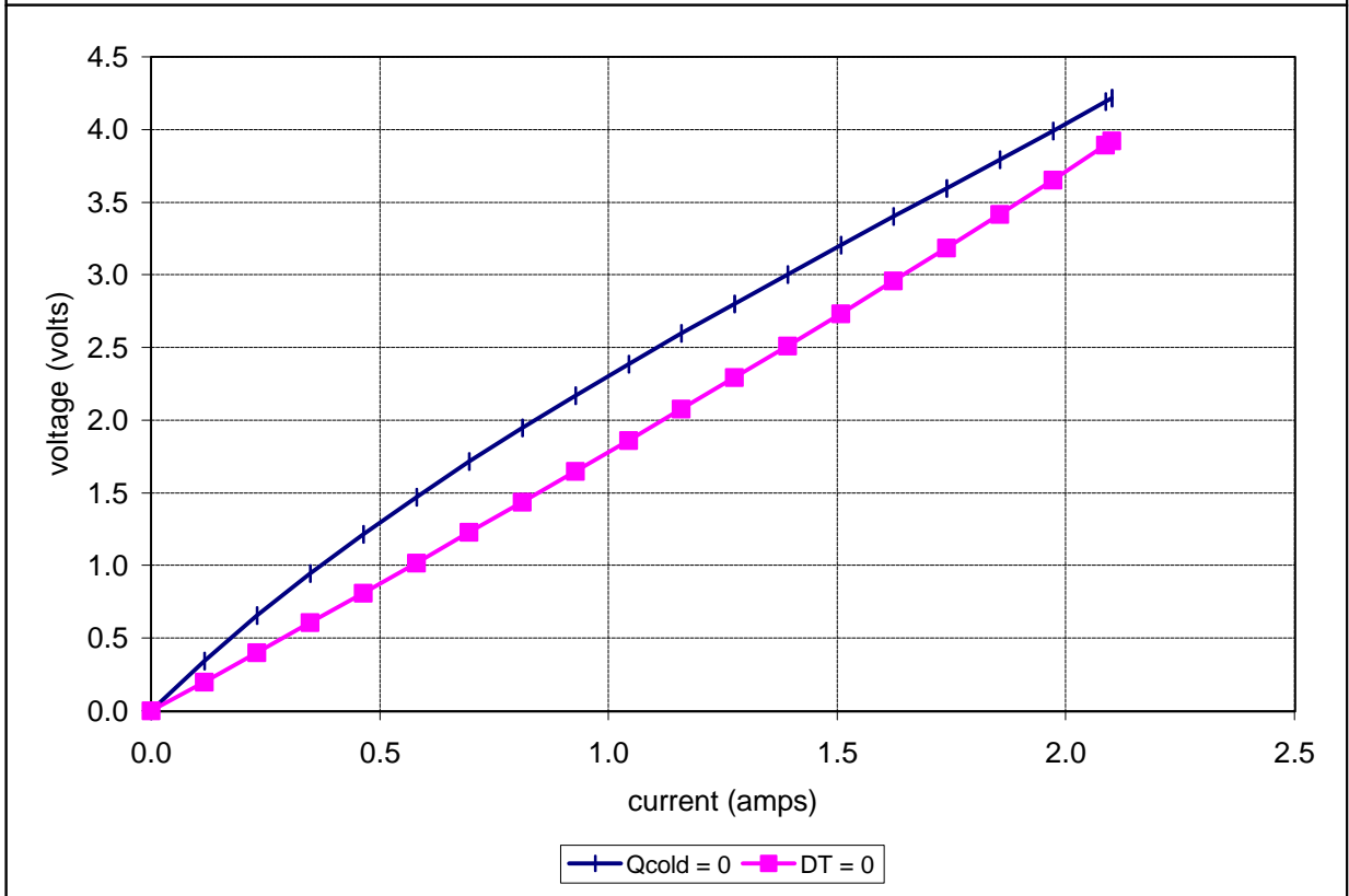
Potted TE-31-0.6-0.8 at a hot-side temperature of 50 °C
