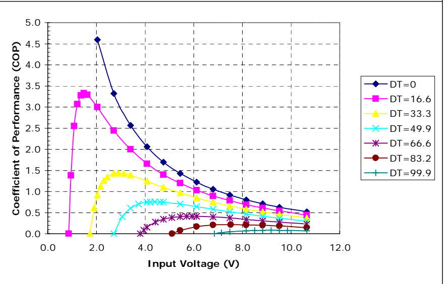
Unpotted TE-3-(83-18-4)-1.3 at a hot-side temperature of 30 °C
