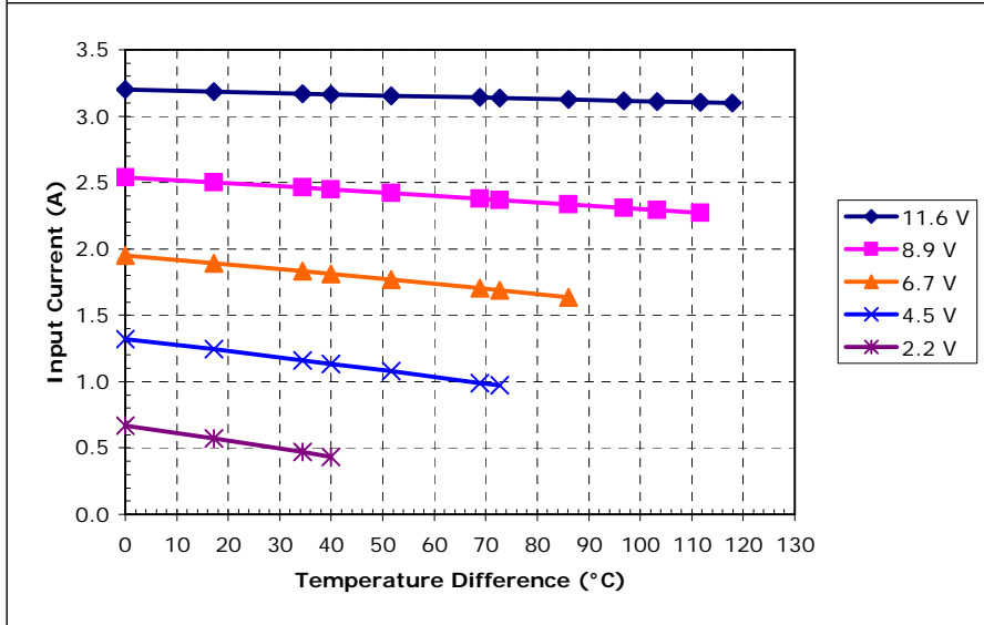
Potted TE-3-(83-18-4)-1.3 at a hot-side temperature of 50 °C
