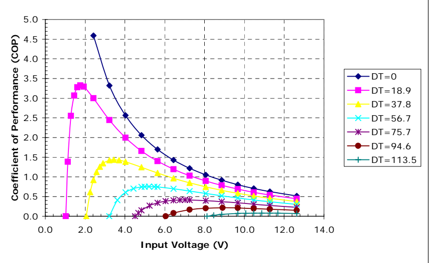
Potted TE-3-(83-18-4)-1.3 at a hot-side temperature of 70 °C
