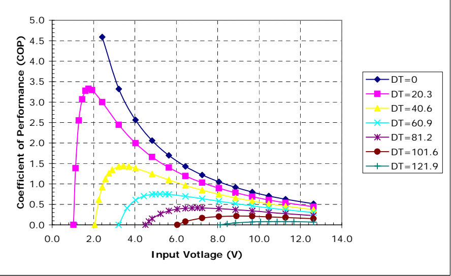
Unpotted TE-3-(83-18-4)-1.3 at a hot-side temperature of 70 °C
