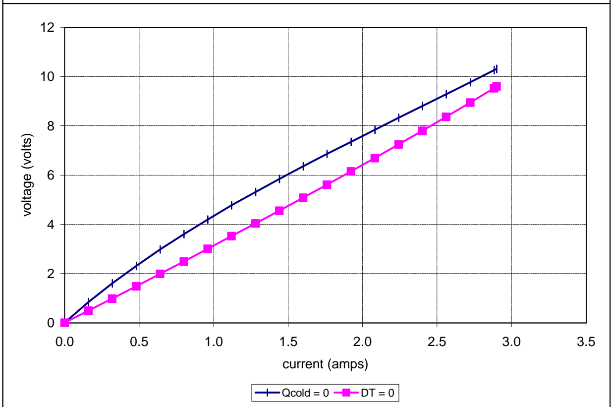
Unpotted TE-3-(83-18-4)-1.3 at a hot-side temperature of 50 °C
