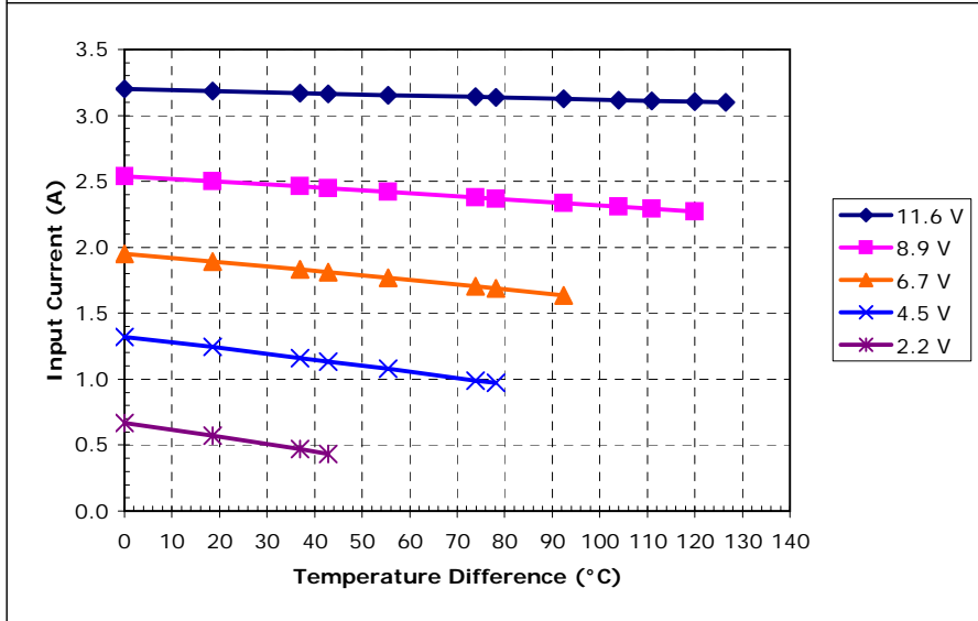
Unpotted TE-3-(83-18-4)-1.3 at a hot-side temperature of 50 °C
