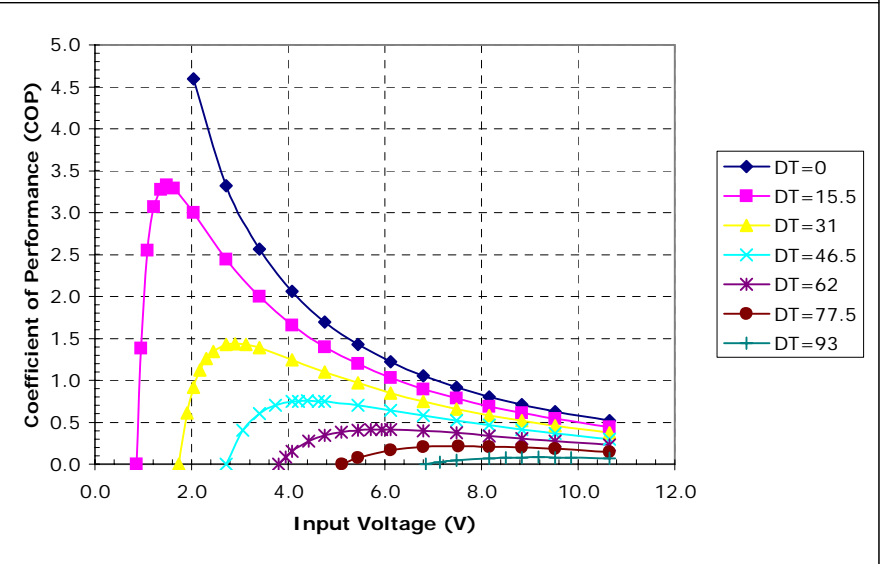
Potted TE-3-(83-18-4)-1.3 at a hot-side temperature of 30 °C
