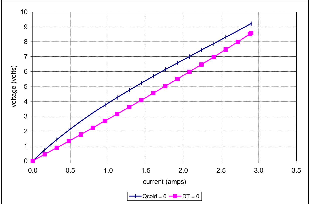
Unpotted TE-3-(83-18-4)-1.3 at a hot-side temperature of 25 °C
